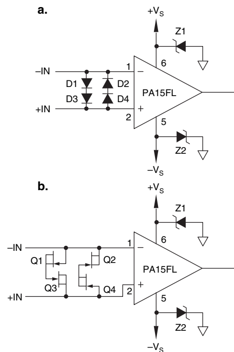
FIGURE 2. OVERVOLTAGE PROTECTION
