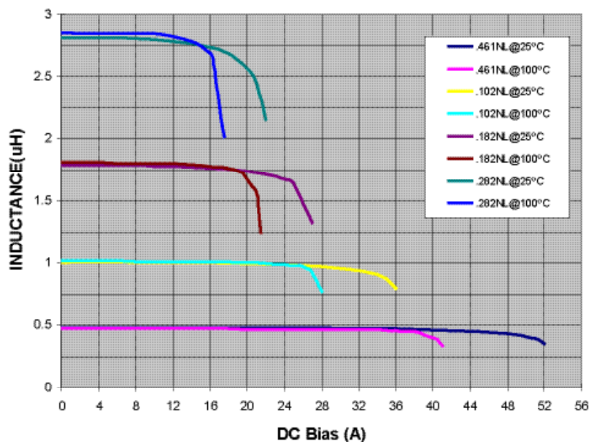
Typical Inductance vs DC Bias
