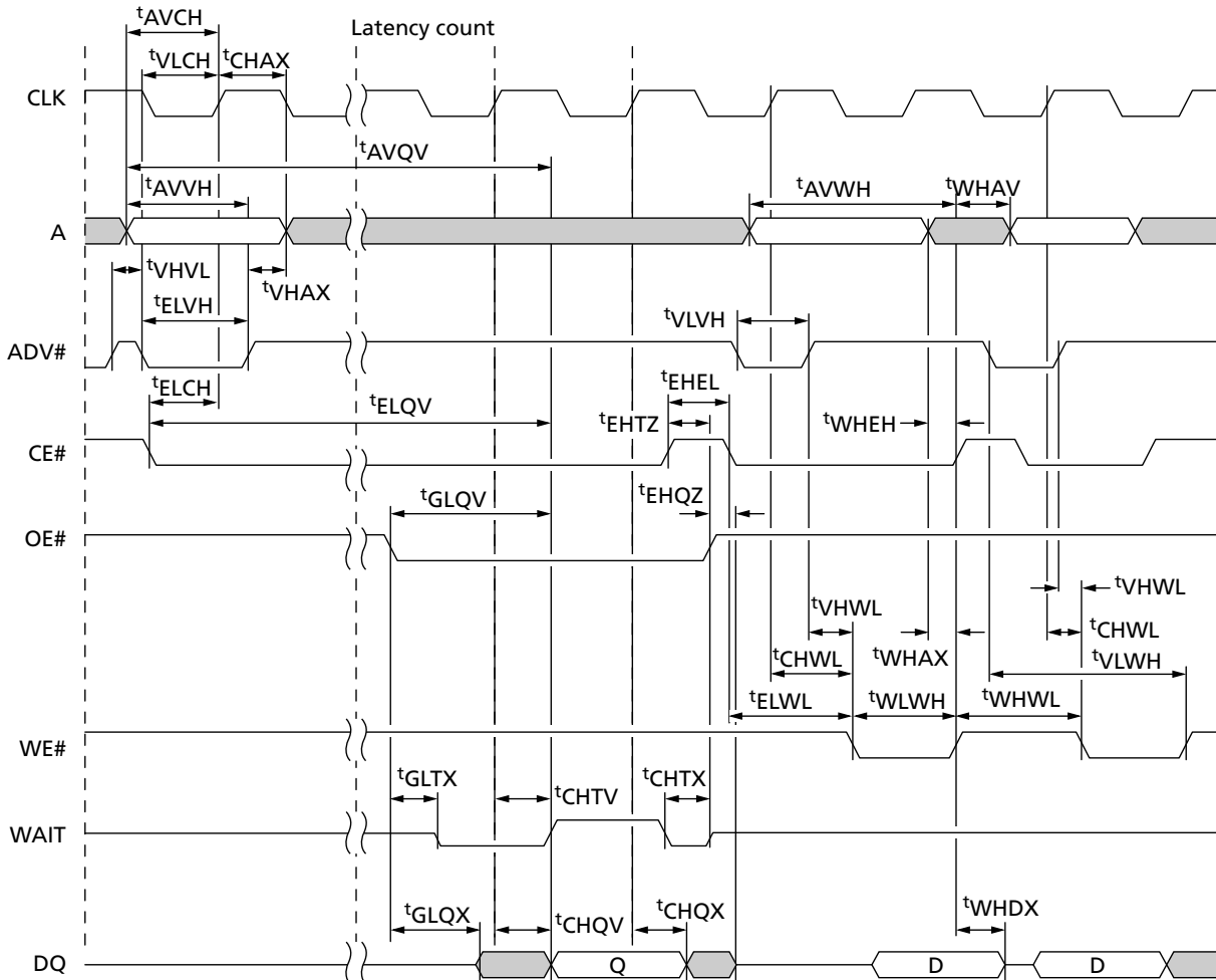
Figure 36: Synchronous Read to Write Timing
