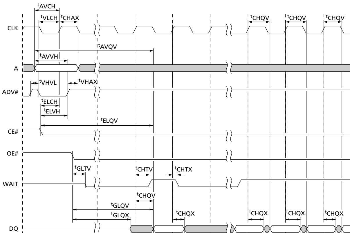
Figure 31: Continuous Burst Read with Output Delay (ADV# LOW)
