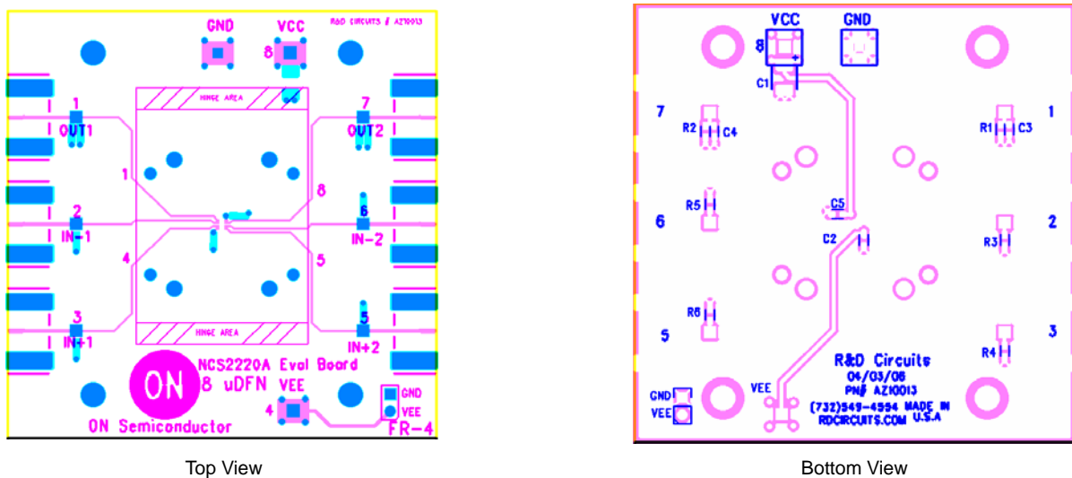
Figure 3. Evaluation Board Layout
