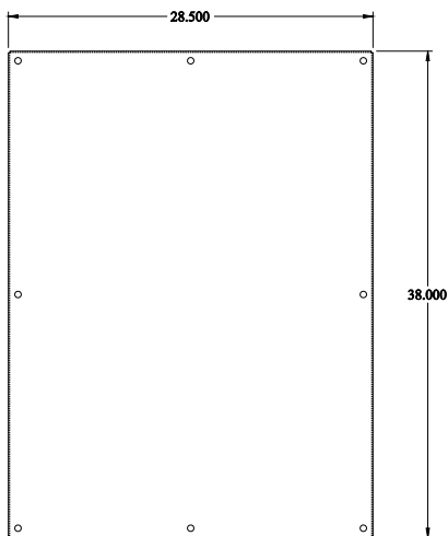
INNER PANEL
