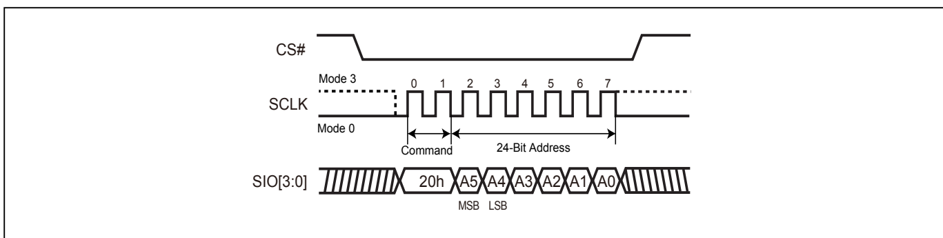
Figure 43. Sector Erase (SE) Sequence (Command 20) (QPI Mode)
