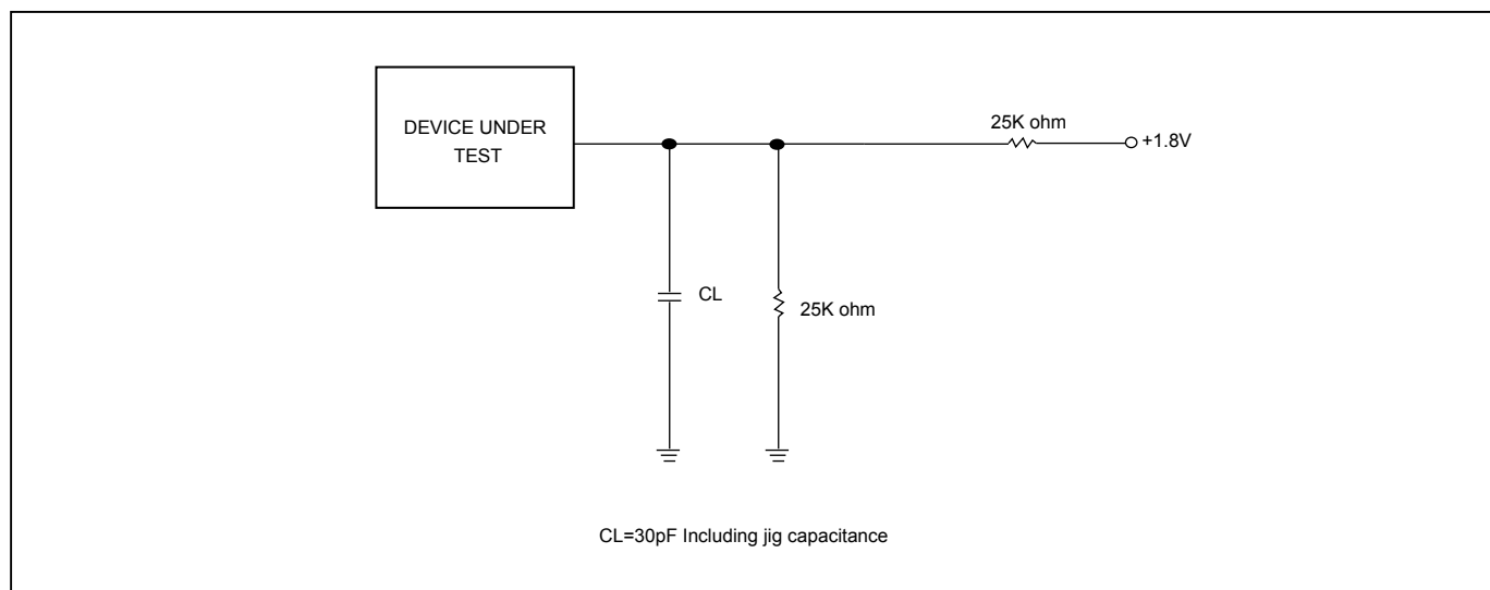
Figure 8. Output Loading
