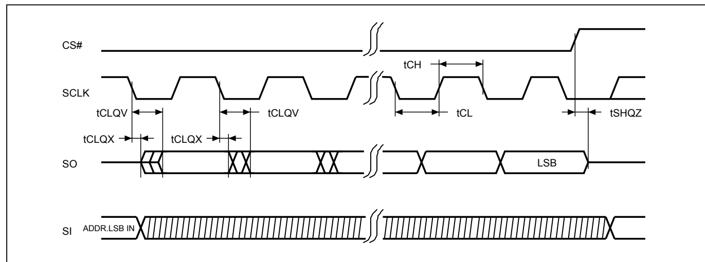
Figure 10. Output Timing
