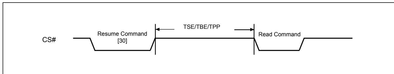
Figure 38-2. Resume to Read Latency
