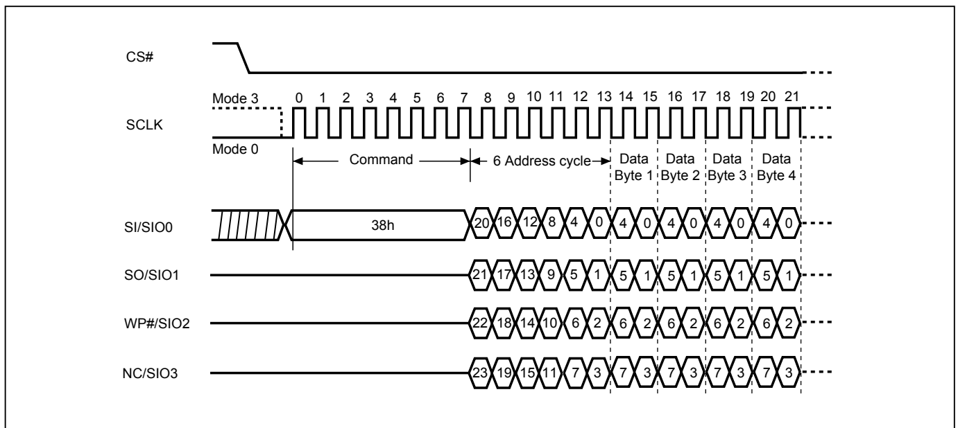
Figure 23. 4 x I/O Page Program (4PP) Sequence (Command 38) (SPI Mode only)
