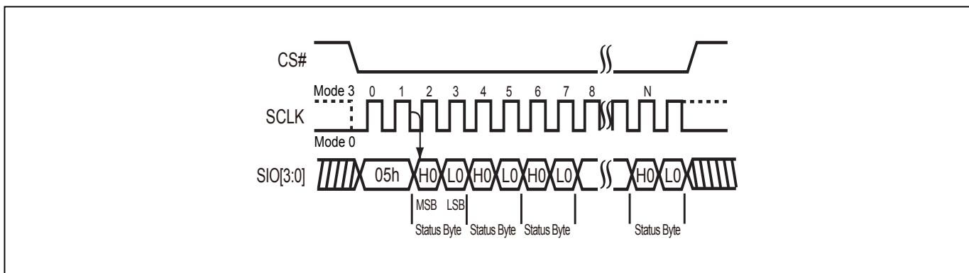
Figure 15-2. Read Status Register (RDSR) Sequence (Command 05) (QPI Mode)
