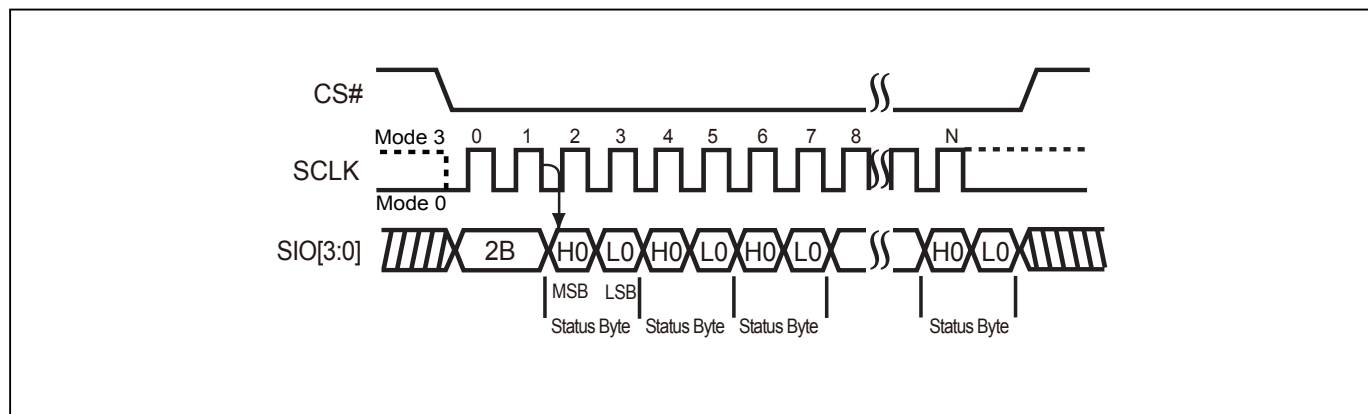
Figure 32-2. Read Security Register (RDSCUR) Sequence (Command 2B) (QPI Mode)
