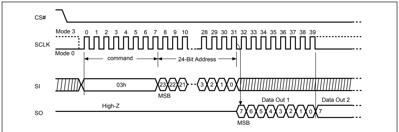
Figure 17. Read Data Bytes (READ) Sequence (Command 03) (SPI Mode only) (33MHz)
