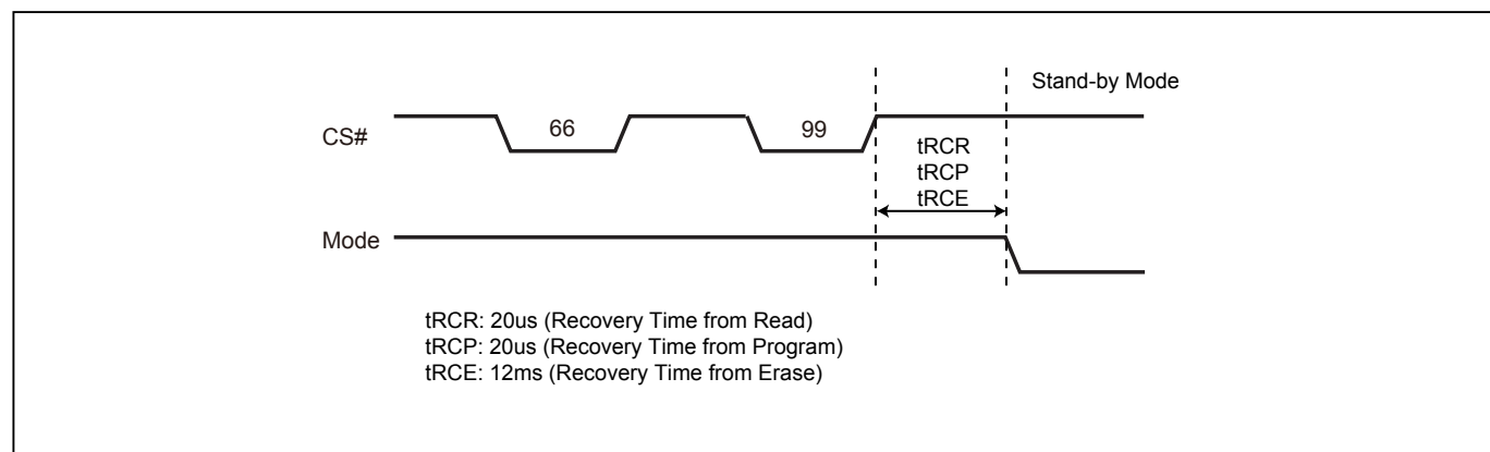
Figure 39. Software Reset Recovery
