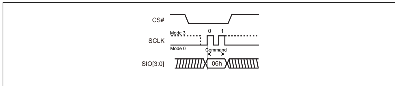
Figure 12-2. Write Enable (WREN) Sequence (Command 06) (QPI Mode)
