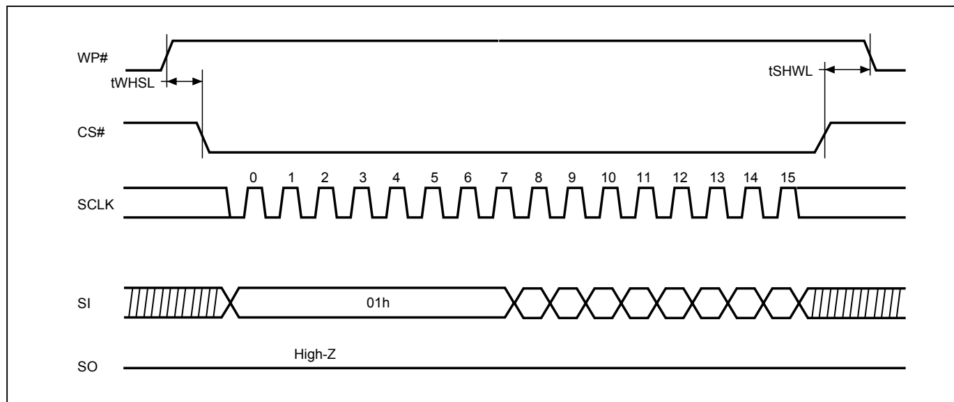
Figure 11. WP# Setup Timing and Hold Timing during WRSR when SRWD=1
