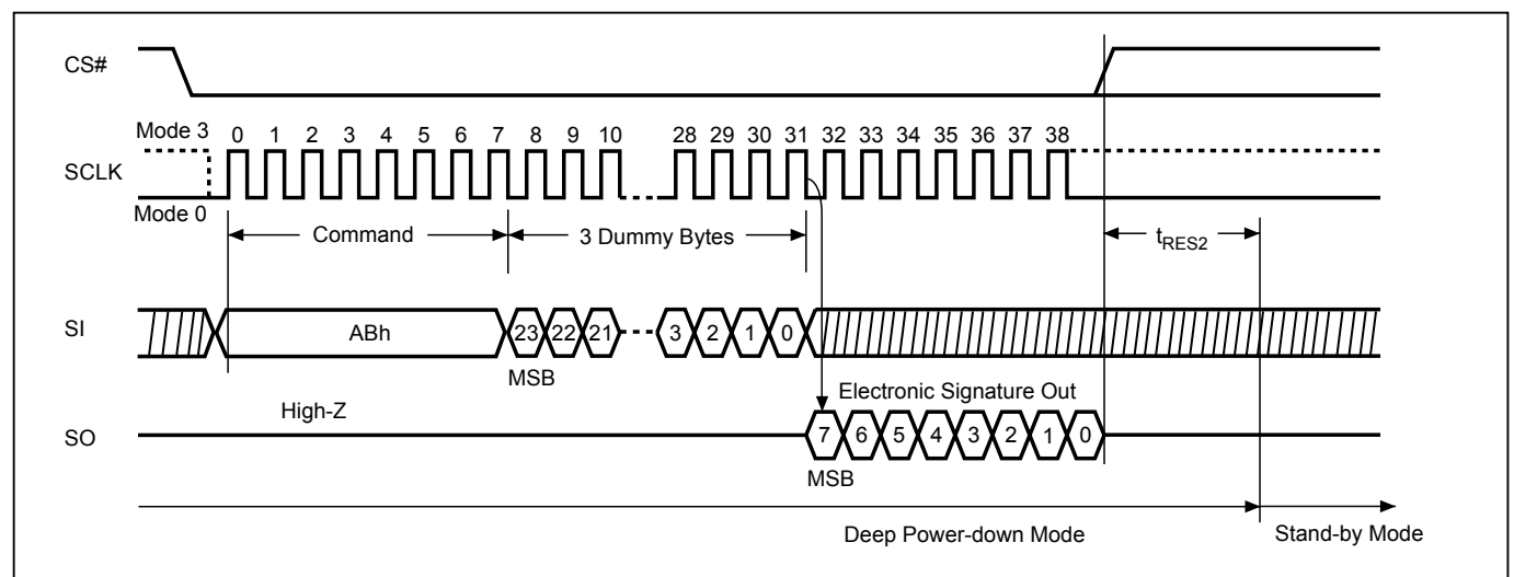
Figure 29. Read Electronic Signature (RES) Sequence (Command AB) (SPI Mode Only)
