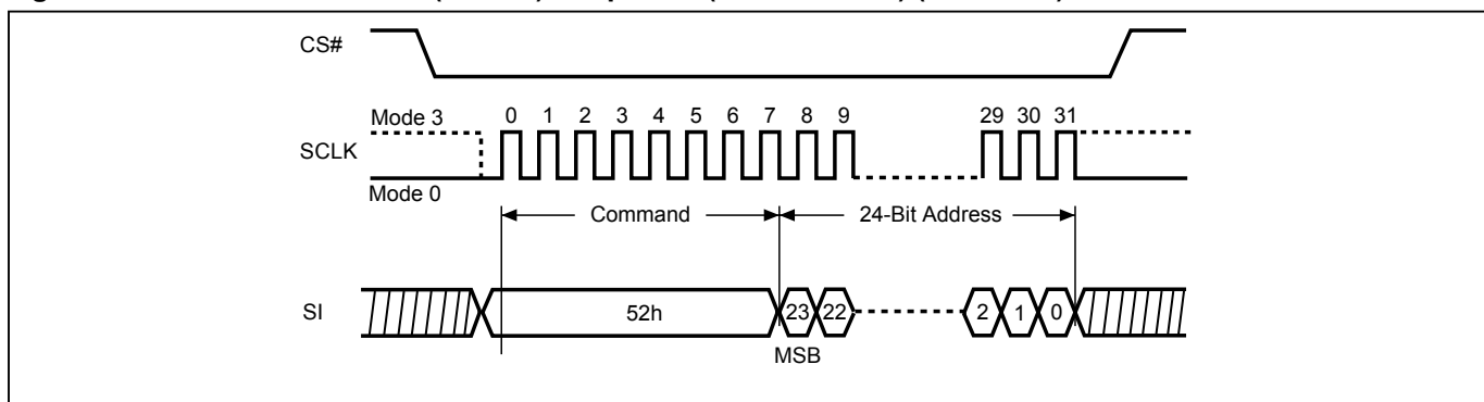
Figure 25-1. Block Erase 32KB (BE32K) Sequence (Command 52) (SPI Mode)
