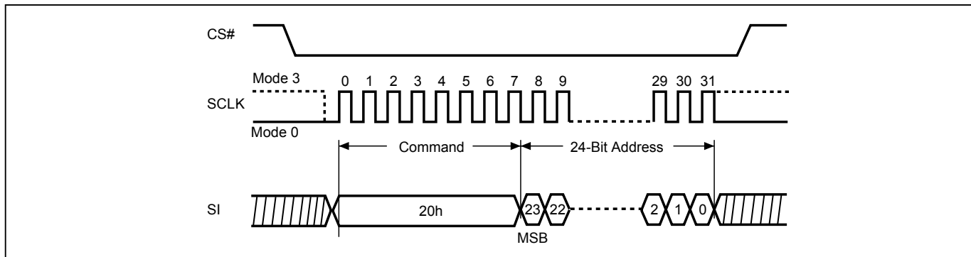
Figure 24-1. Sector Erase (SE) Sequence (Command 20) (SPI Mode)
