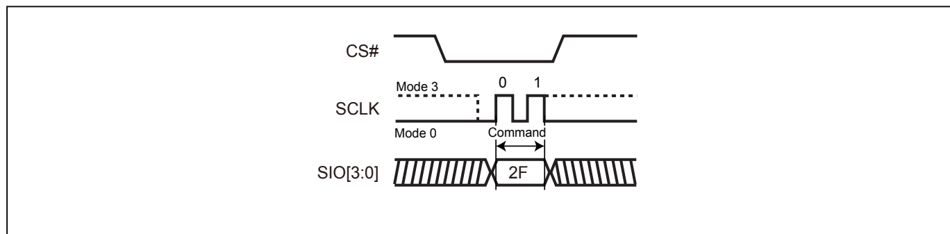
Figure 33-2. Write Security Register (WRSCUR) Sequence (Command 2F) (QPI Mode)
