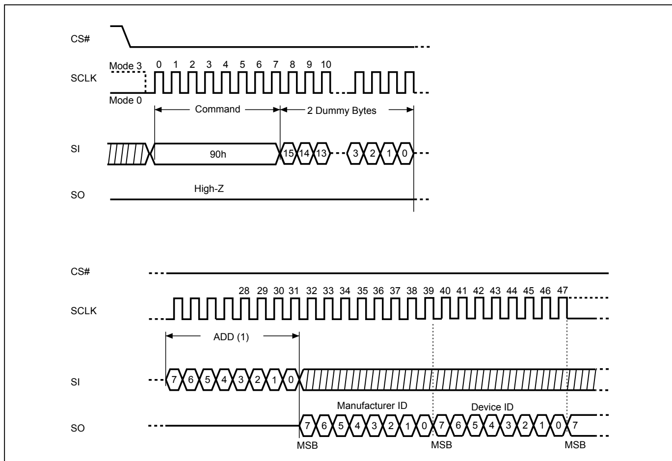
Figure 31. Read Electronic Manufacturer & Device ID (REMS) Sequence (Command 90) (SPI Mode only)
