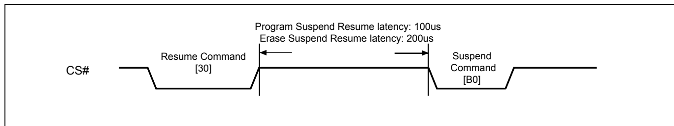
Figure 38-3. Resume to Suspend Latency
