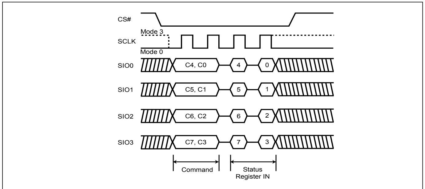
Figure 16-2. Write Status Register (WRSR) Sequence (Command 01) (QPI Mode)
