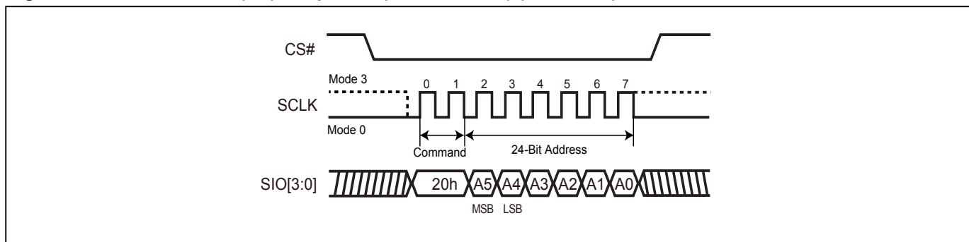
Figure 24-2. Sector Erase (SE) Sequence (Command 20) (QPI Mode)
