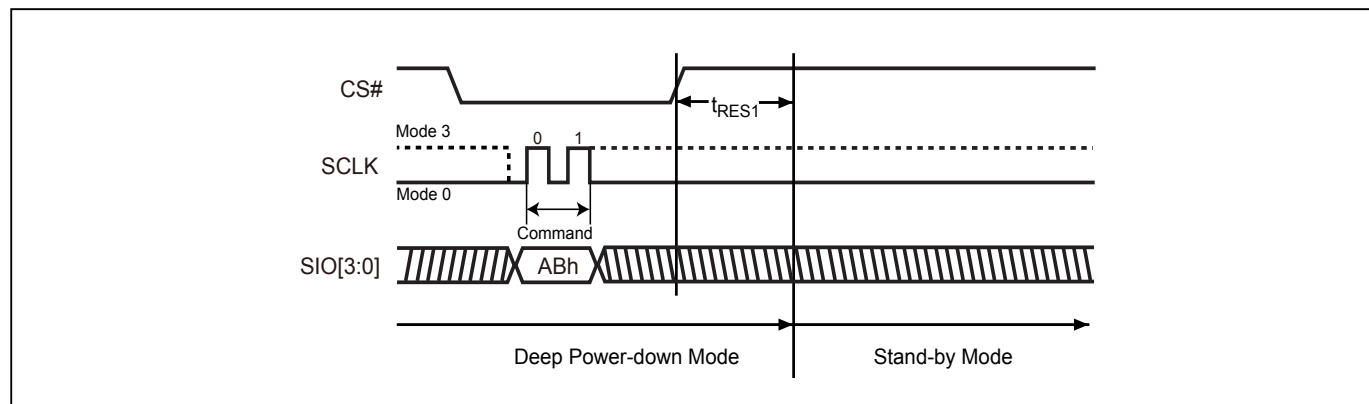
Figure 30-2. Release from Deep Power-down (RDP) Sequence (Command AB) (QPI Mode)
