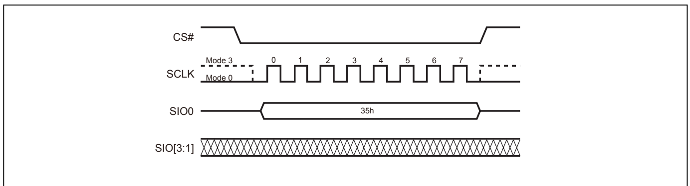
Figure 37. Enable Quad I/O Sequence
