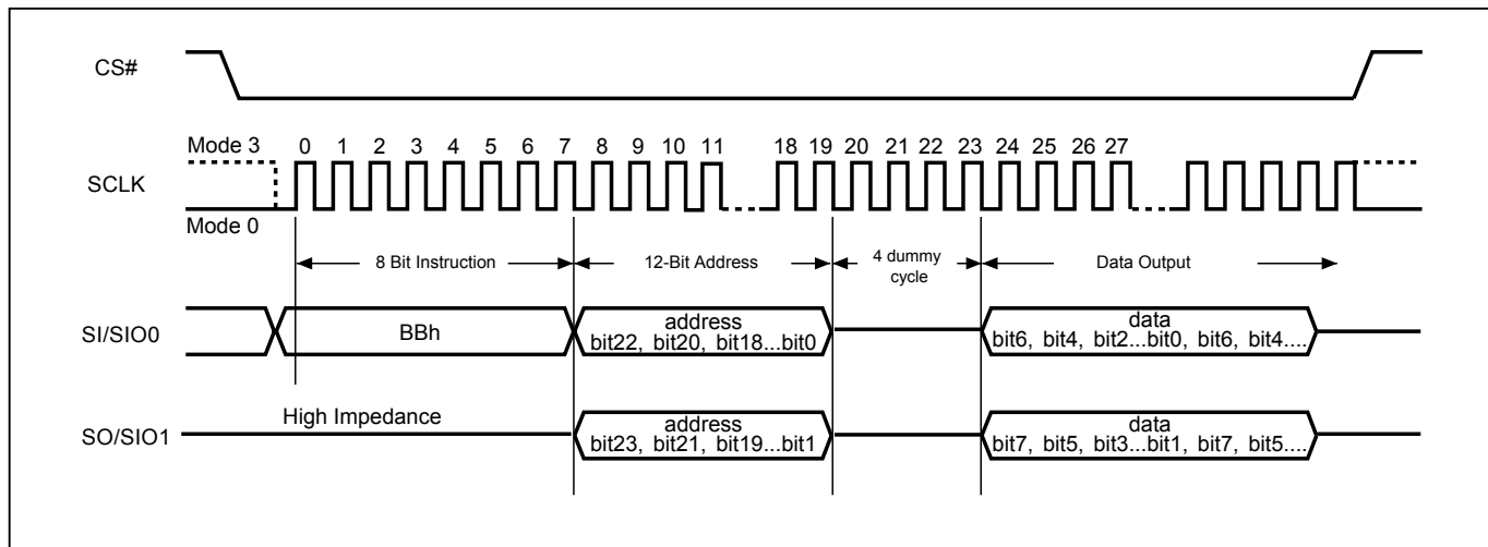
Figure 19. 2 x I/O Read Mode Sequence (Command BB) (SPI Mode only) (84MHz)
