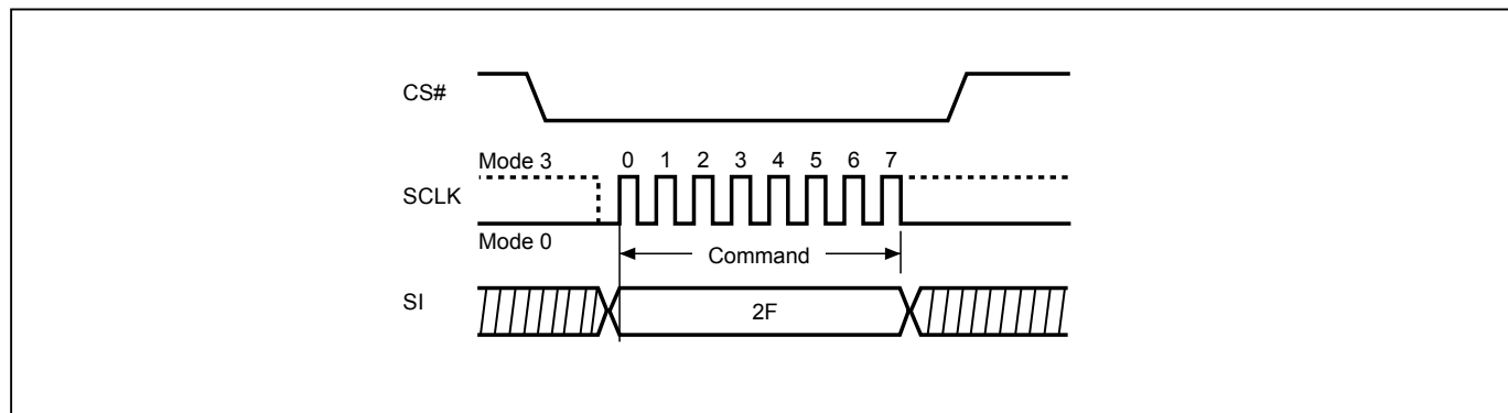
Figure 33-1. Write Security Register (WRSCUR) Sequence (Command 2F) (SPI Mode)
