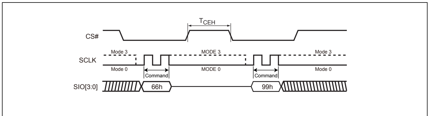
Figure 36-2. Reset Sequence (QPI mode)
