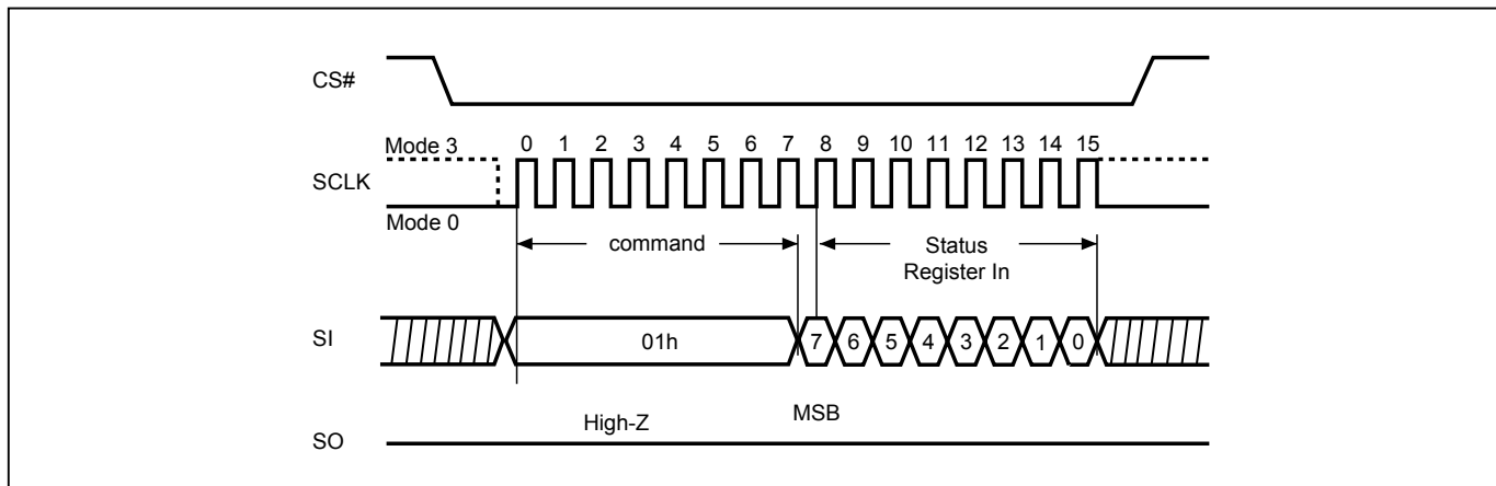
Figure 16-1. Write Status Register (WRSR) Sequence (Command 01) (SPI Mode)
