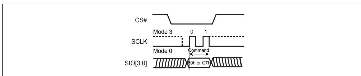
Figure 27-2. Chip Erase (CE) Sequence (Command 60 or C7) (QPI Mode)
