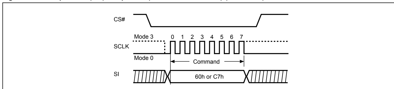
Figure 27-1. Chip Erase (CE) Sequence (Command 60 or C7) (SPI Mode)
