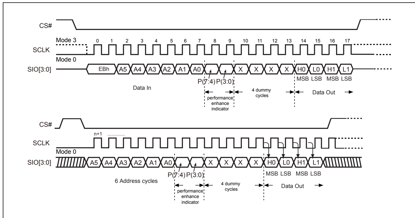
Figure 21-2. 4 x I/O Read enhance performance Mode Sequence (Command EB) (QPI Mode) (104MHz)
