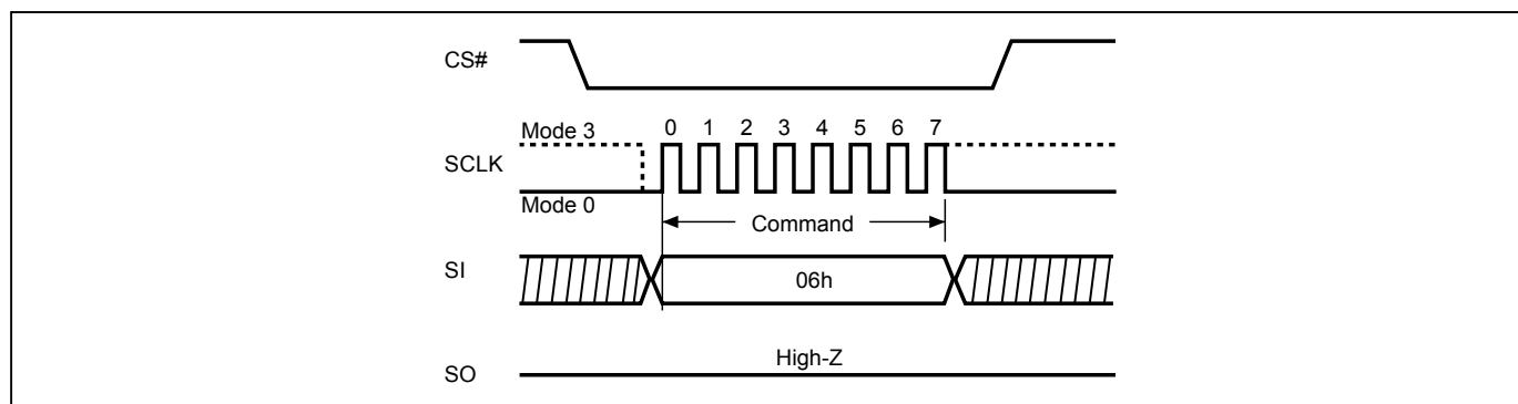
Figure 12-1. Write Enable (WREN) Sequence (Command 06) (SPI Mode)
