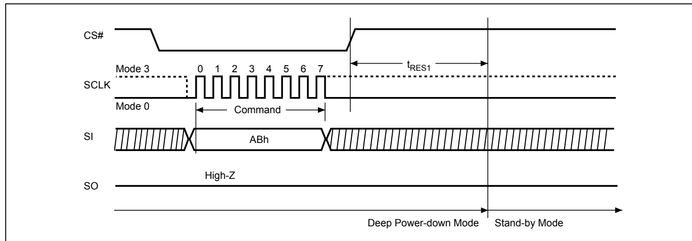
Figure 30-1. Release from Deep Power-down (RDP) Sequence (Command AB) (SPI Mode)
