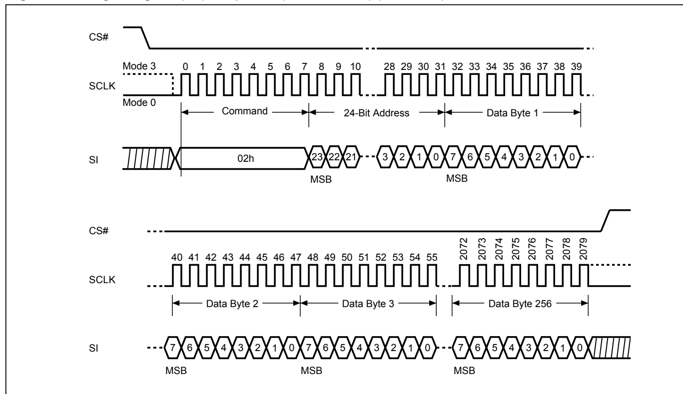
Figure 22-1. Page Program (PP) Sequence (Command 02) (SPI Mode)
