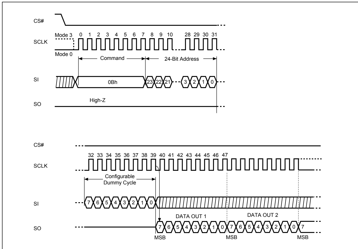
Figure 18-1. Read at Higher Speed (FAST_READ) Sequence (Command 0B) (SPI Mode) (104MHz)
