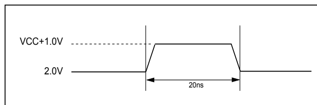
Figure 6. Maximum Positive Overshoot Waveform
