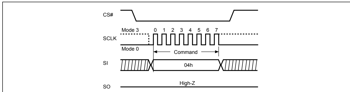
Figure 13-1. Write Disable (WRDI) Sequence (Command 04) (SPI Mode)
