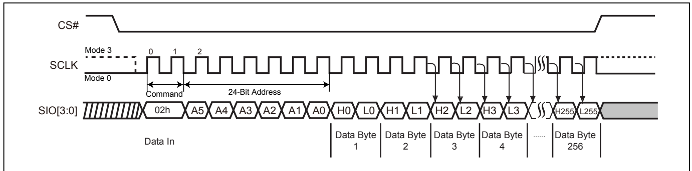
Figure 22-2. Page Program (PP) Sequence (Command 02) (QPI Mode)
