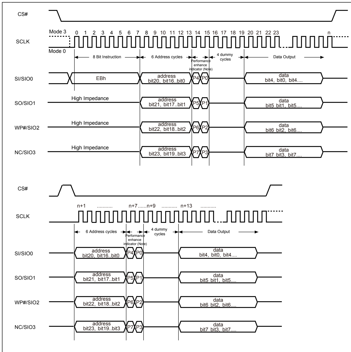
Figure 21-1. 4 x I/O Read enhance performance Mode Sequence (Command EB) (SPI Mode) (104MHz)
