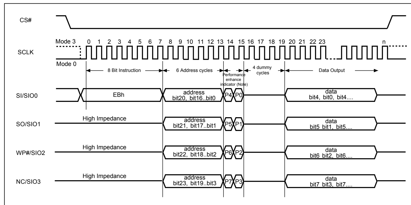
Figure 20. 4 x I/O Read Mode Sequence (Command EB) (SPI Mode) (104MHz)
