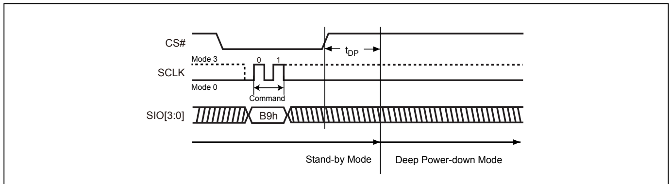
Figure 28-2. Deep Power-down (DP) Sequence (Command B9) (QPI Mode)
