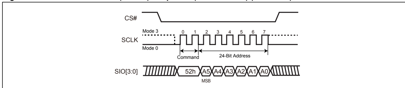
Figure 25-2. Block Erase 32KB (BE32K) Sequence (Command 52) (QPI Mode)
