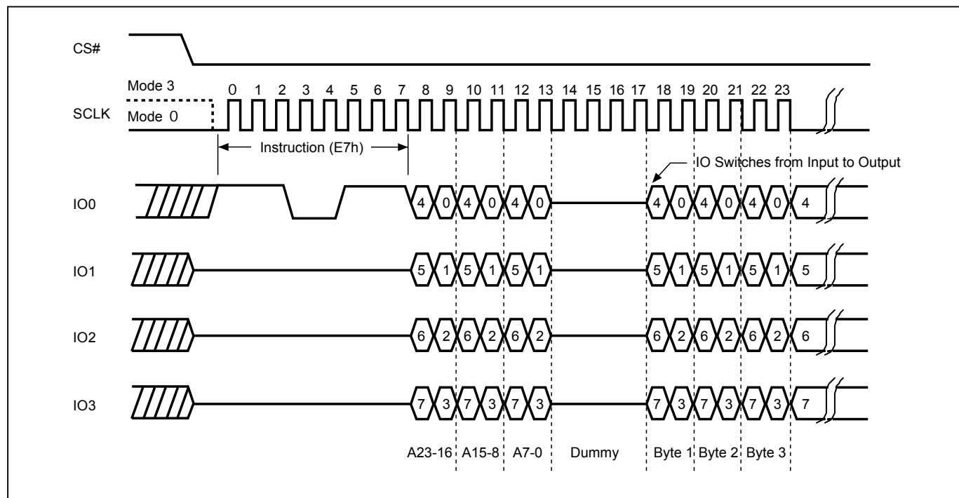
Figure 34. Word Read Quad I/O Instruction Sequence (Initial Word Read Quad I/O instruction or previous P4=1) (SPI Mode only) (84MHz)
