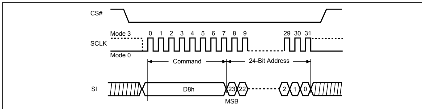
Figure 26-1. Block Erase (BE) Sequence (Command D8) (SPI Mode)
