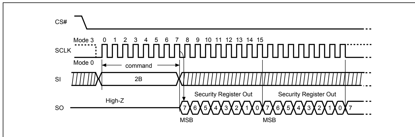
Figure 32-1. Read Security Register (RDSCUR) Sequence (Command 2B) (SPI Mode)
