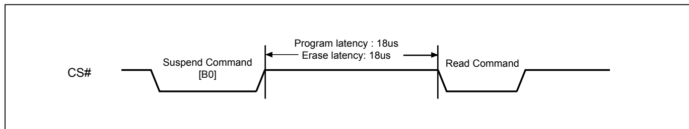
Figure 38-1. Suspend to Read Latency
