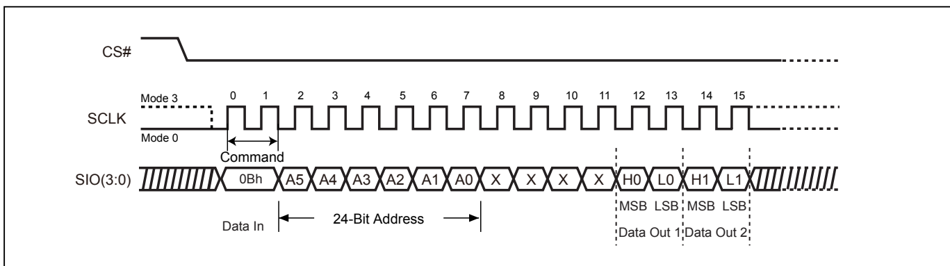
Figure 18-2. Read at Higher Speed (FAST_READ) Sequence (Command 0B) (QPI Mode) (84MHz)
