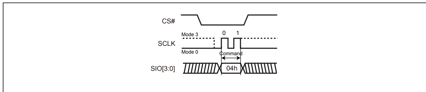
Figure 13-2. Write Disable (WRDI) Sequence (Command 04) (QPI Mode)
