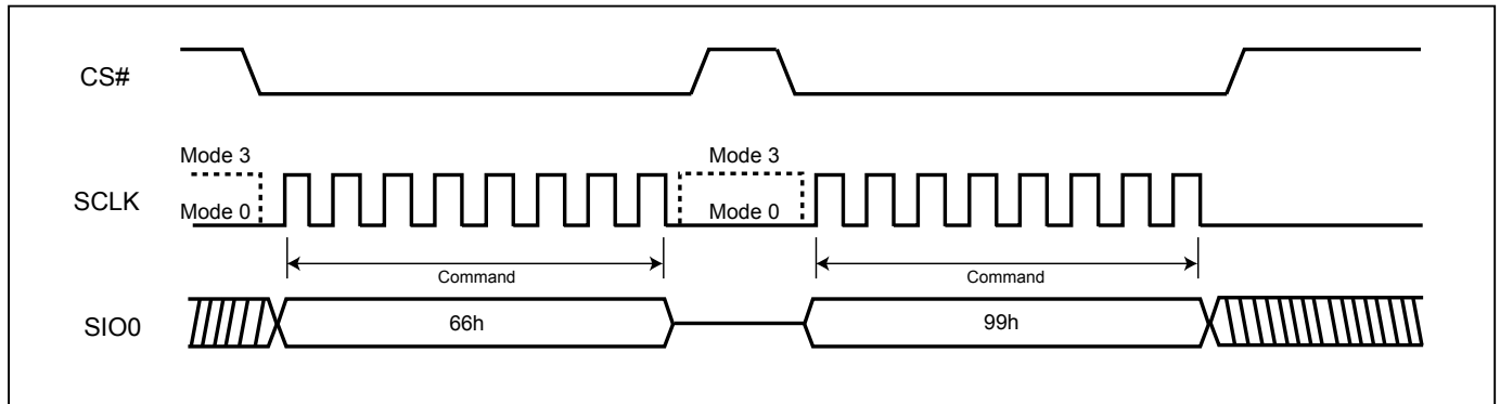
Figure 36-1. Reset Sequence (SPI mode)
