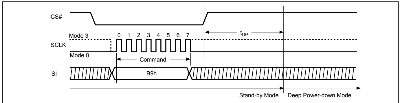
Figure 28-1. Deep Power-down (DP) Sequence (Command B9) (SPI Mode)
