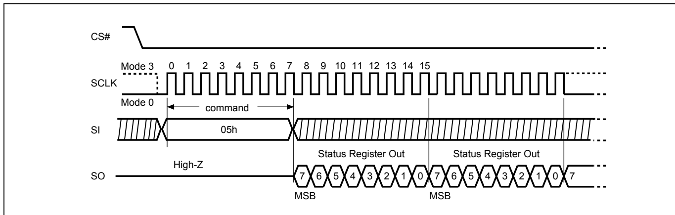
Figure 15-1. Read Status Register (RDSR) Sequence (Command 05) (SPI Mode)
