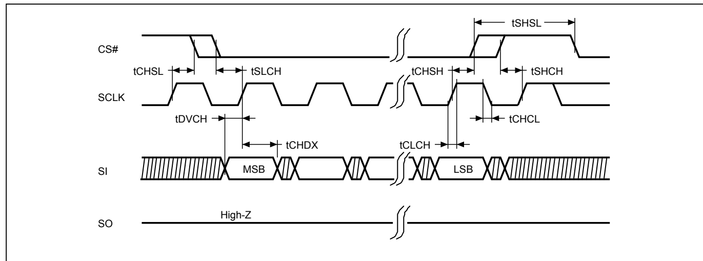
Figure 9. Serial Input Timing
