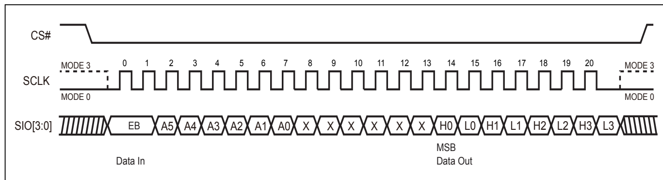
Figure 4. Fast QPI Read Mode (FASTRDQ) (Command EBH)
