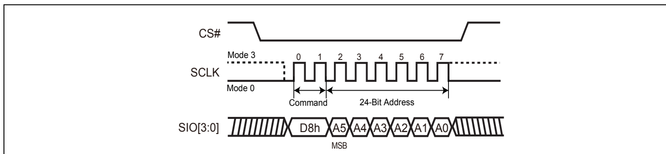
Figure 26-2. Block Erase (BE) Sequence (Command D8) (QPI Mode)
