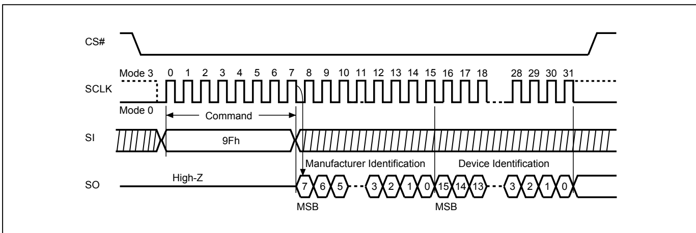
Figure 14. Read Identification (RDID) Sequence (Command 9F) (SPI mode only)
