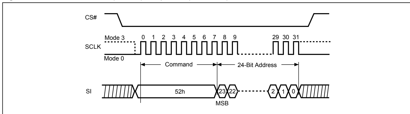
Figure 45. Block Erase 32KB (BE32K) Sequence (SPI Mode)
