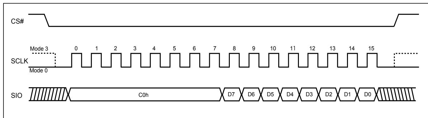
Figure 35. SPI Mode
