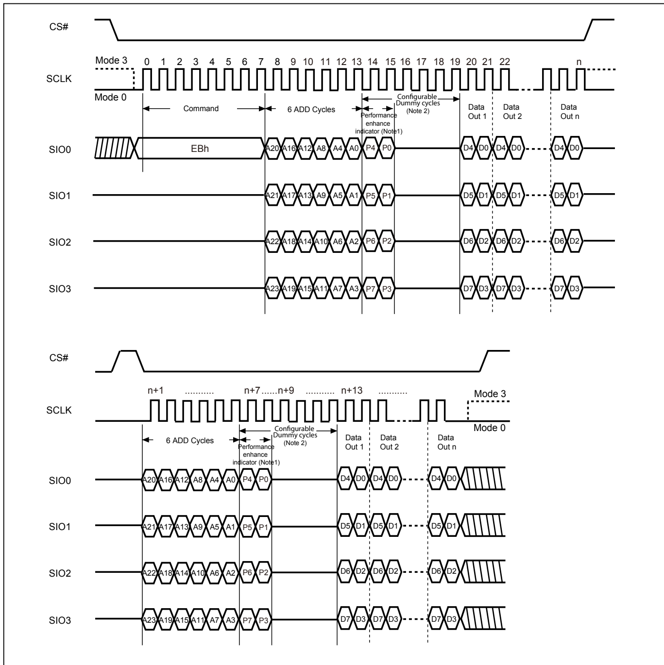
Figure 38. 4 x I/O Read enhance performance Mode Sequence (SPI Mode), for MX25U12835FZNI-08G only
