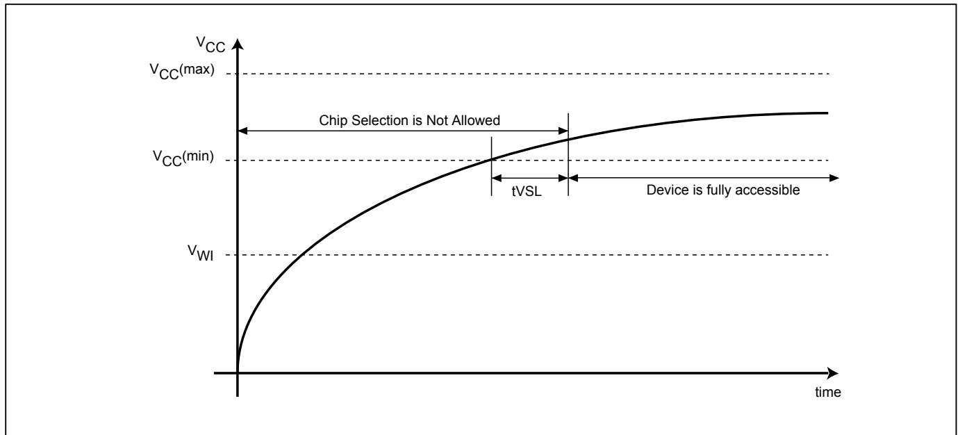
Figure 73. Power-up Timing
