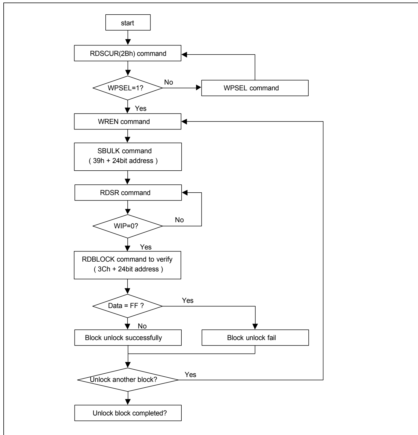
Figure 58. Block Unlock Flow
