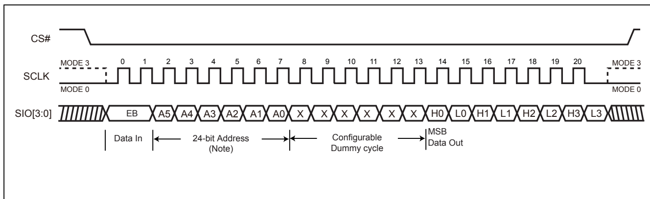
Figure 33. 4 x I/O Read Mode Sequence (QPI Mode), for MX25U12835FZNI-08G only
