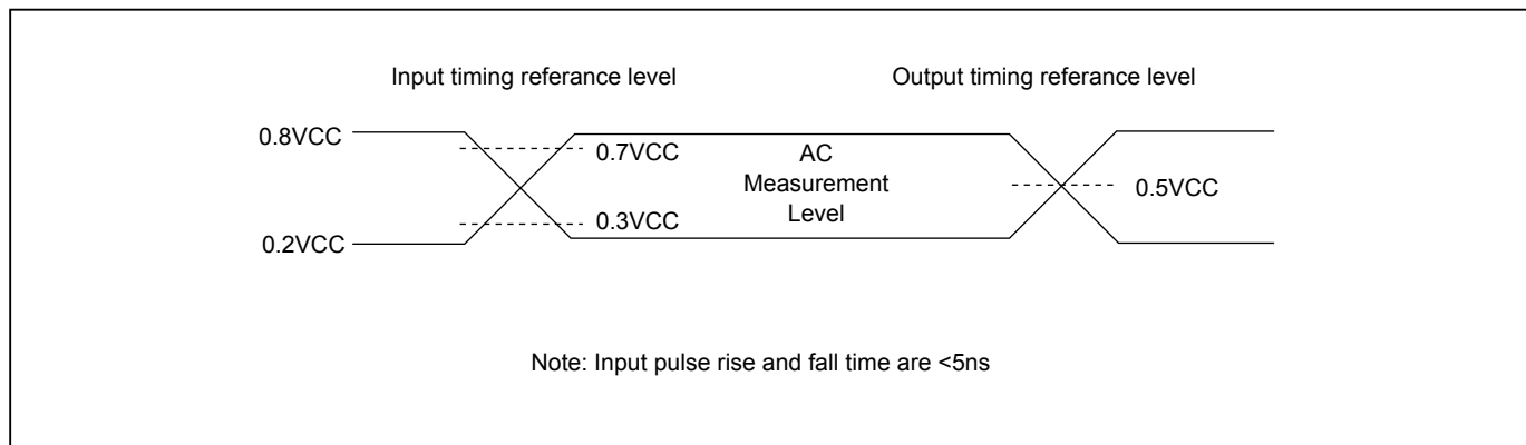
Figure 69. Input Test Waveforms and Measurement Level
