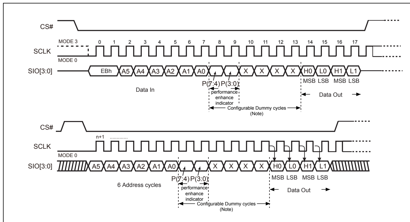
Figure 40. 4 x I/O Read enhance performance Mode Sequence (QPI Mode), for MX25U12835FZNI-08G only
