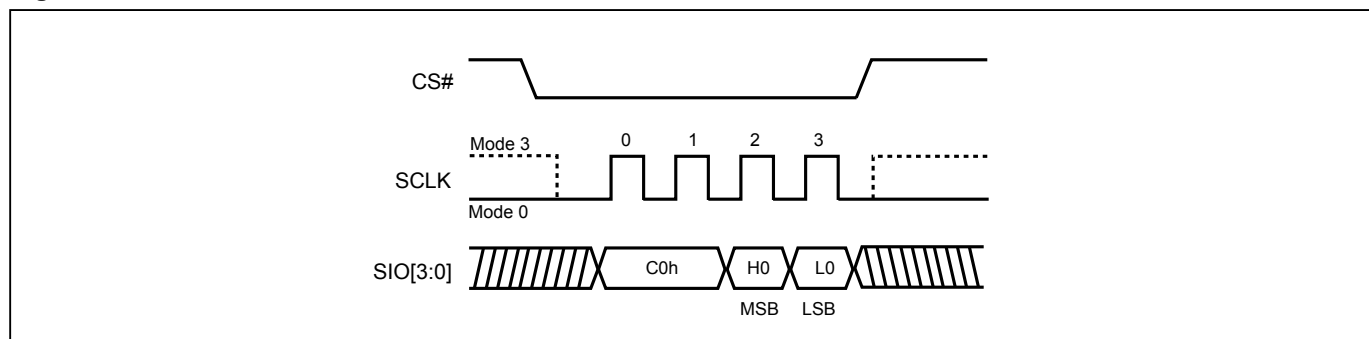
Figure 36. QPI Mode
