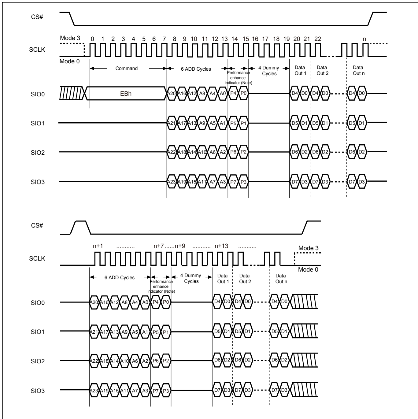
Figure 37. 4 x I/O Read enhance performance Mode Sequence (SPI Mode)
