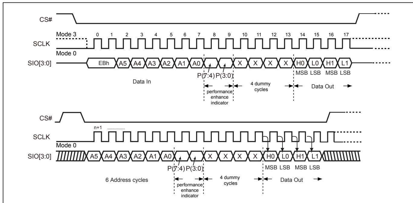
Figure 39. 4 x I/O Read enhance performance Mode Sequence (QPI Mode)
