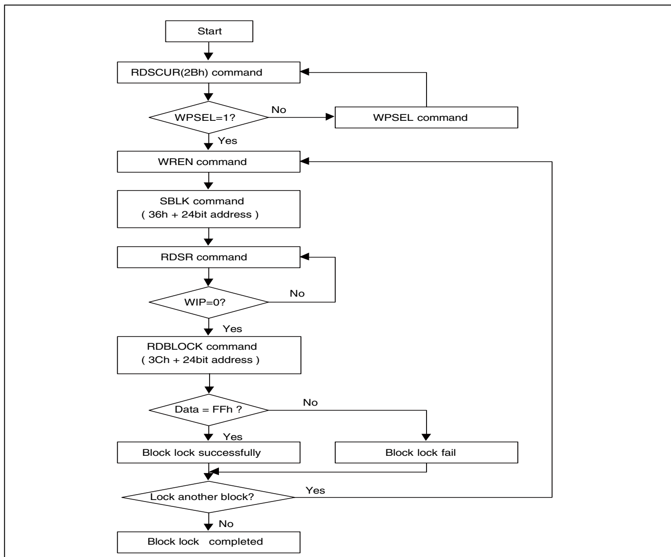
Figure 57. Block Lock Flow
