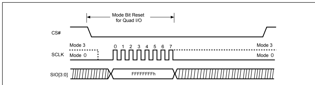
Figure 42. Performance Enhance Mode Reset for Fast Read Quad I/O (QPI Mode)
