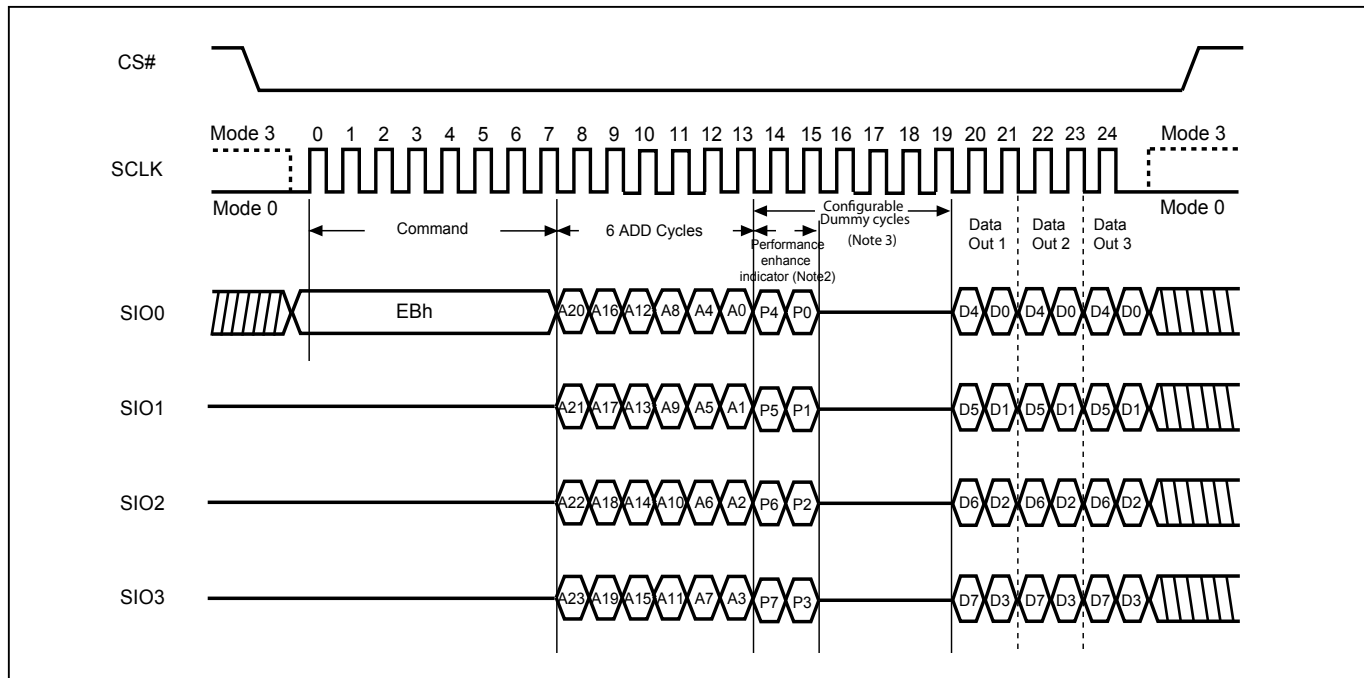
Figure 31. 4 x I/O Read Mode Sequence (SPI Mode), for MX25U12835FZNI-08G only
