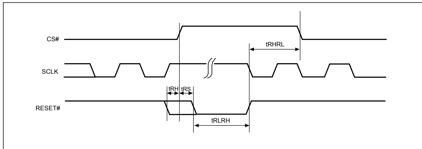
Figure 66. RESET Timing
