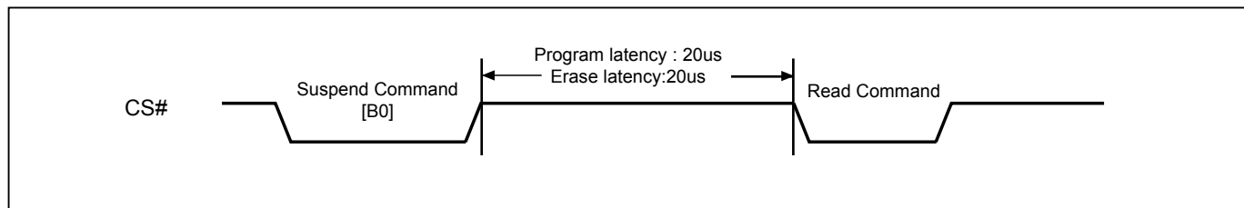
Figure 59. Suspend to Read Latency
