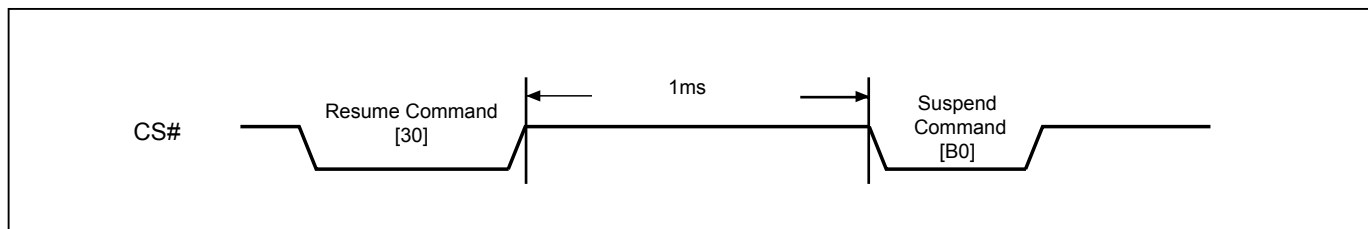
Figure 61. Resume to Suspend Latency
