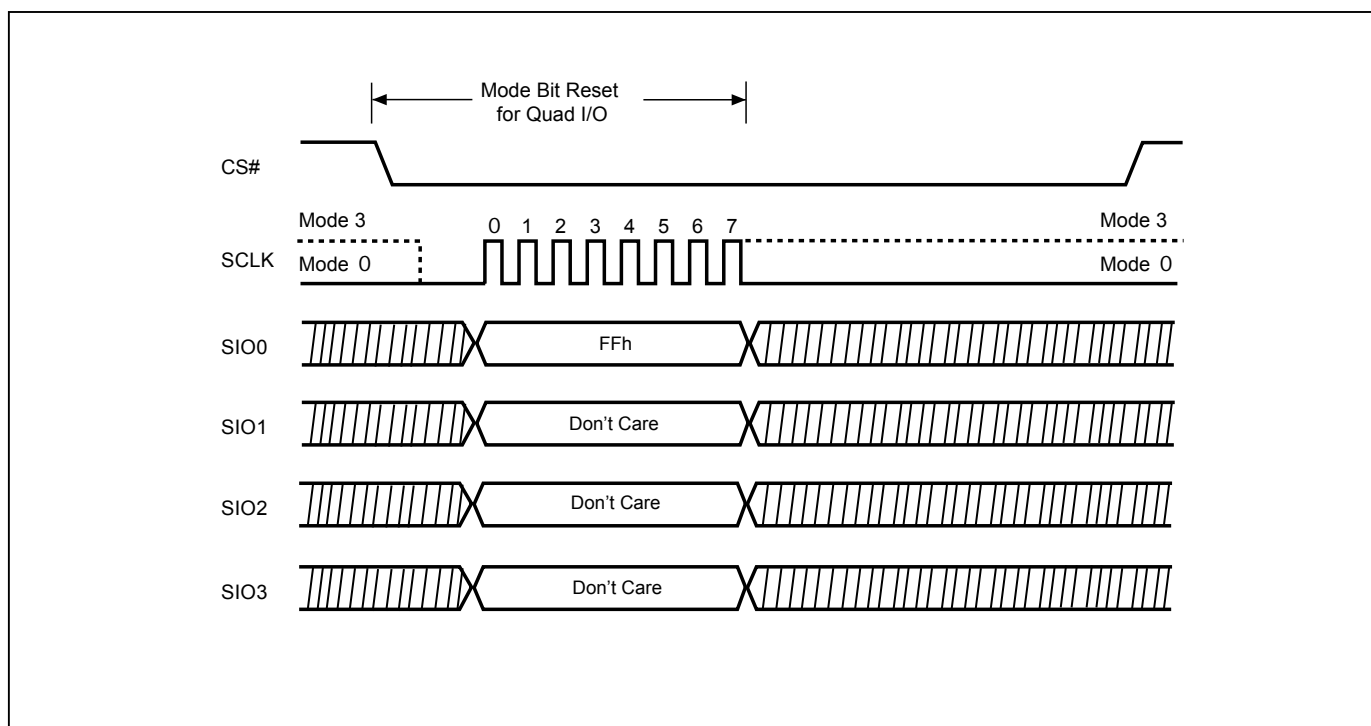
Figure 41. Performance Enhance Mode Reset for Fast Read Quad I/O (SPI Mode)
