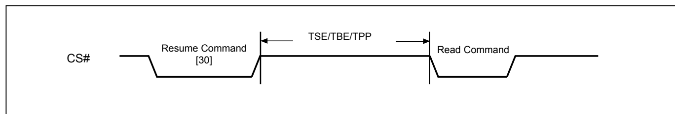
Figure 60. Resume to Read Latency
