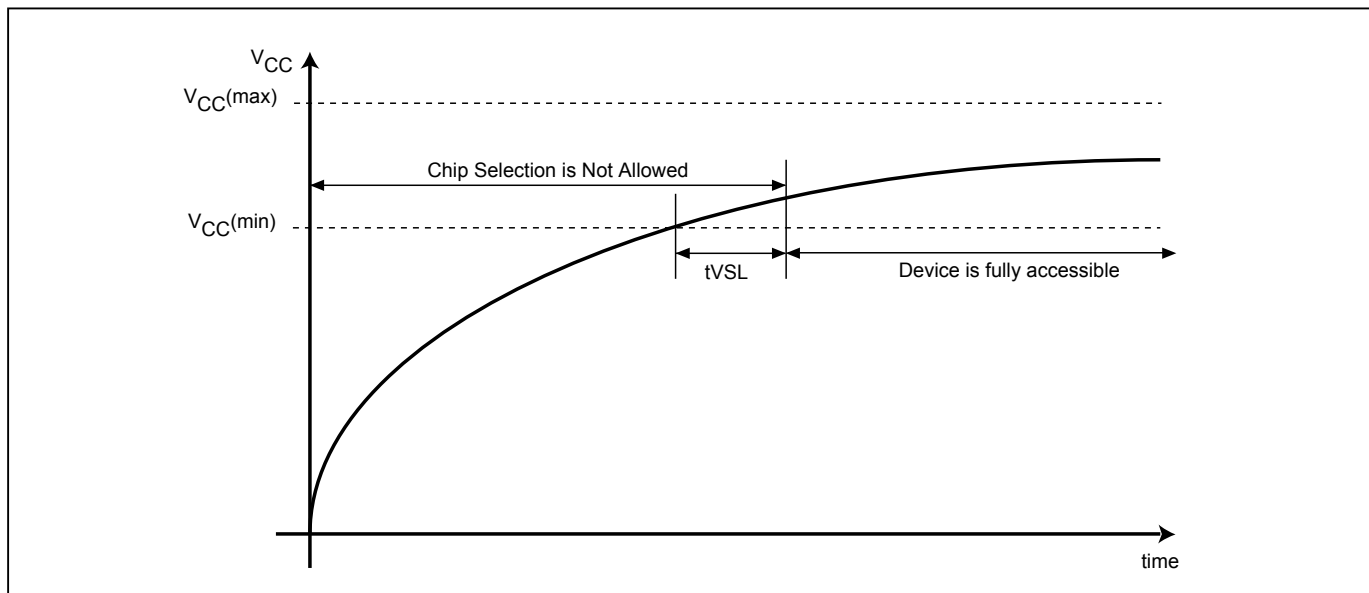
Figure 27. Power-up Timing
