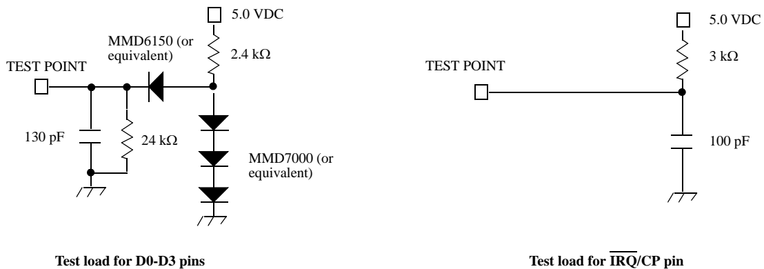
Figure 16 - Test Circuits
