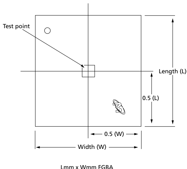
Figure 4: Example Temperature Test Point Location
