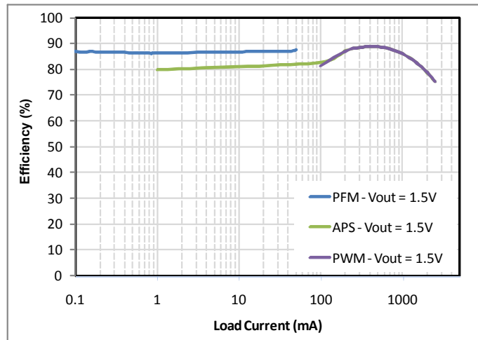
Figure 20. SW3AB Single Phase Efficiency Waveforms
