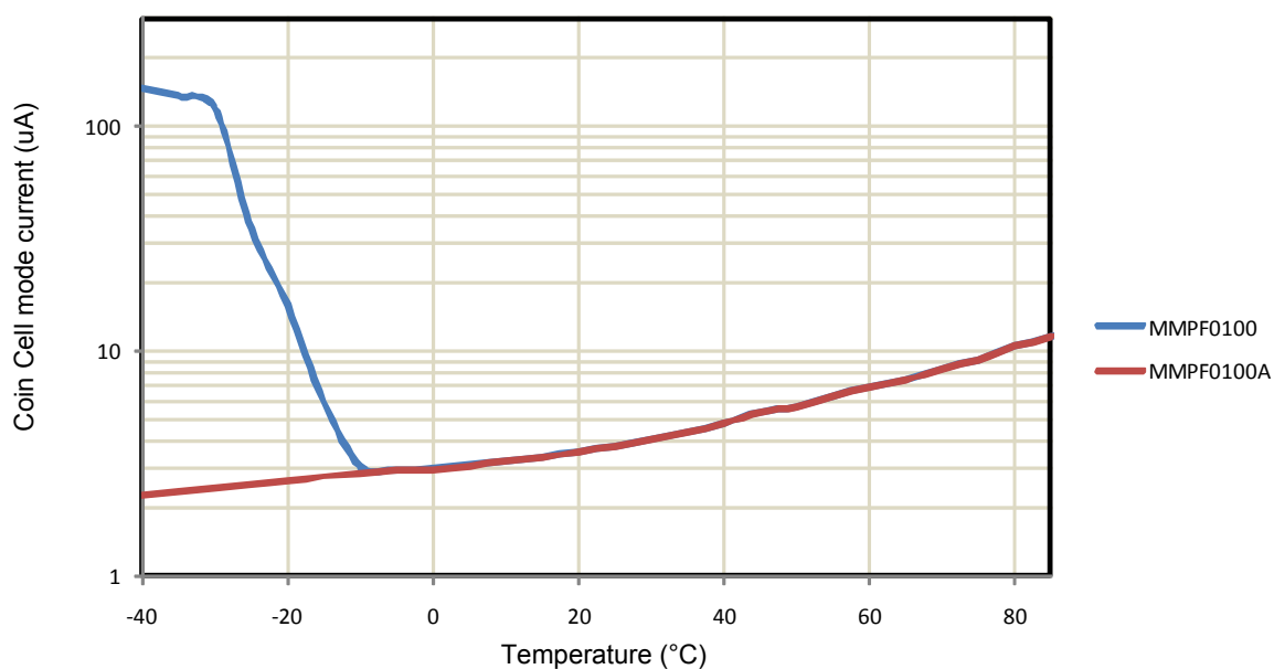
Figure 4. Current Waveforms Over Temperature
