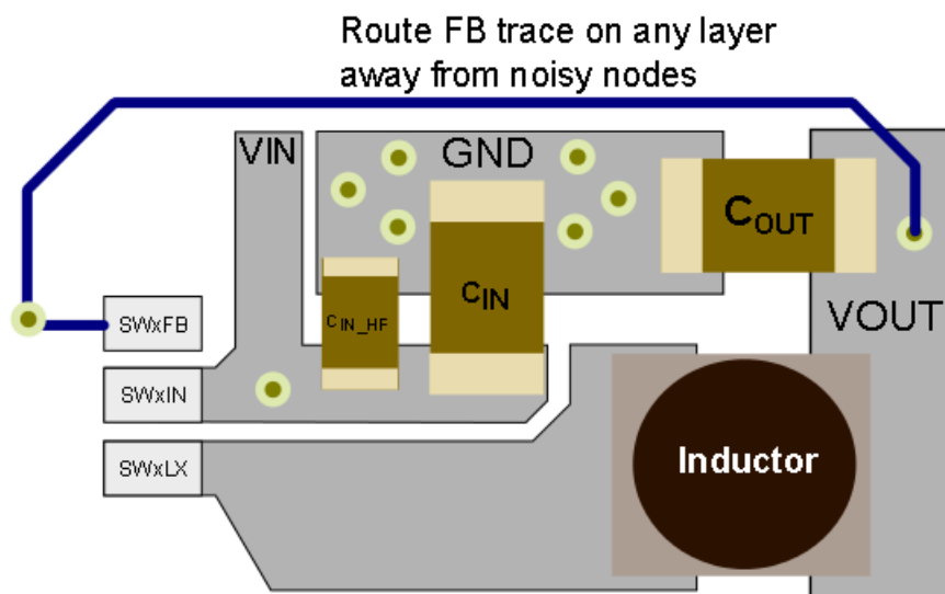
Figure 32. Layout Example for Buck Regulators
