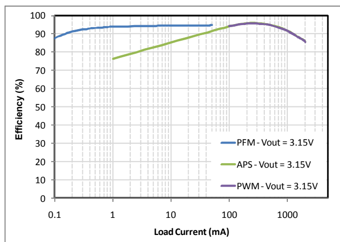
Figure 16. SW2 Efficiency Waveforms
