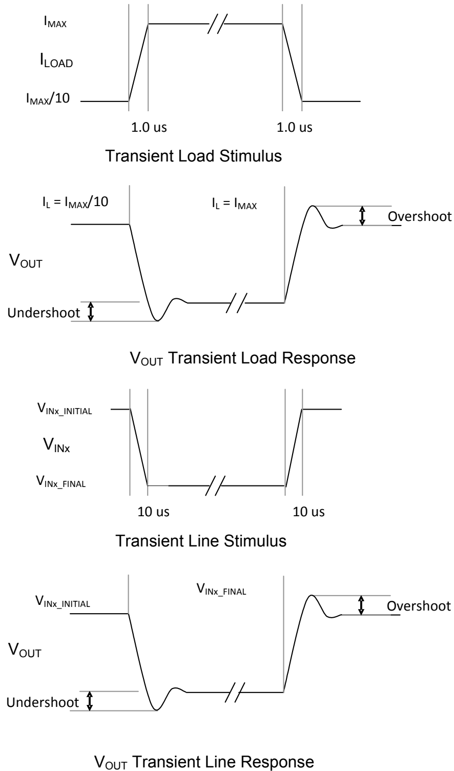
Figure 25. Transient Waveforms
