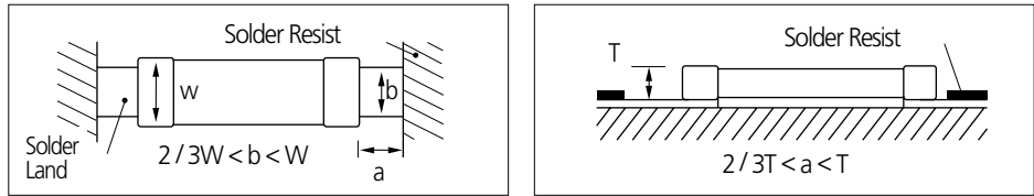
Recommendation of solder Land Shape and Size
