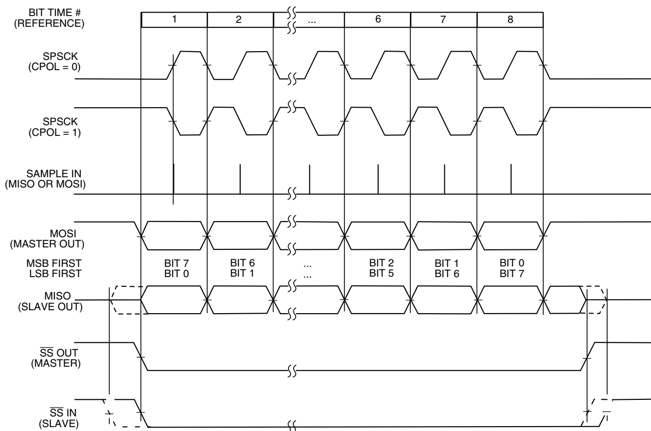
Figure 37-39. SPI clock formats ( \text{CPHA} = 0 )
