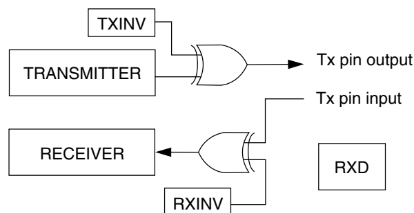
Figure 38-174. Single-wire operation (C1[LOOPS] = 1, C1[RSRC] = 1)
