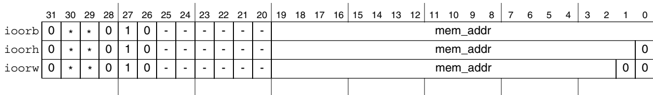
Figure 43-4. Decorated address store: logical OR
