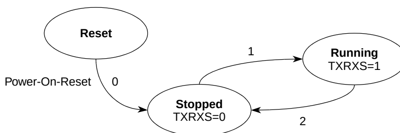
Figure 28-12. DSPI Start and Stop State Diagram
