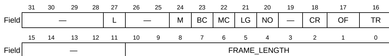
Figure 31-39. Receive Frame Status Word Format (RFSW)
