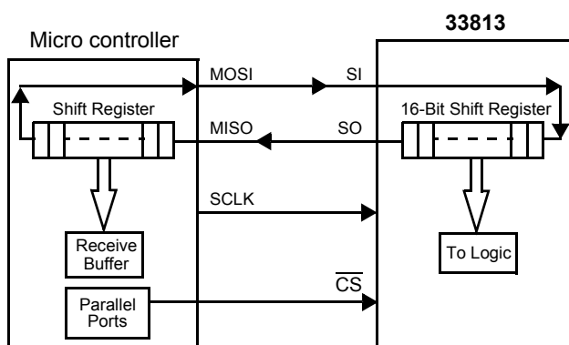
Figure 9. SPI Interface with Microprocessor
