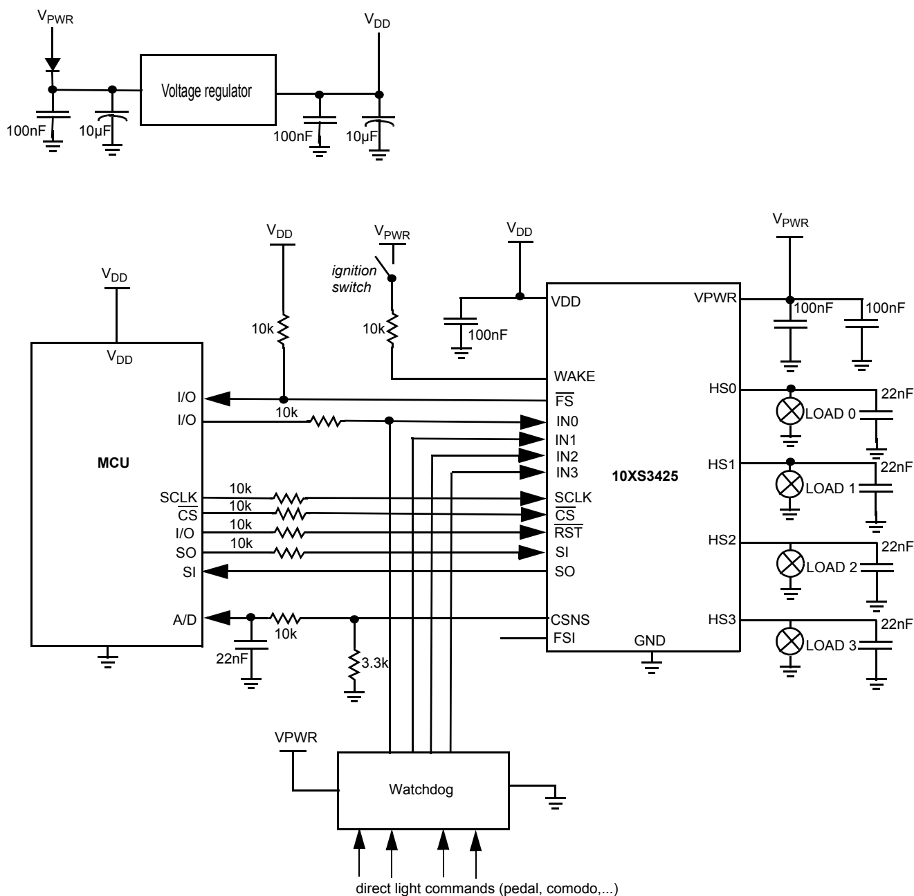
Figure 16. Typical Automotive Lighting (One Corner)
