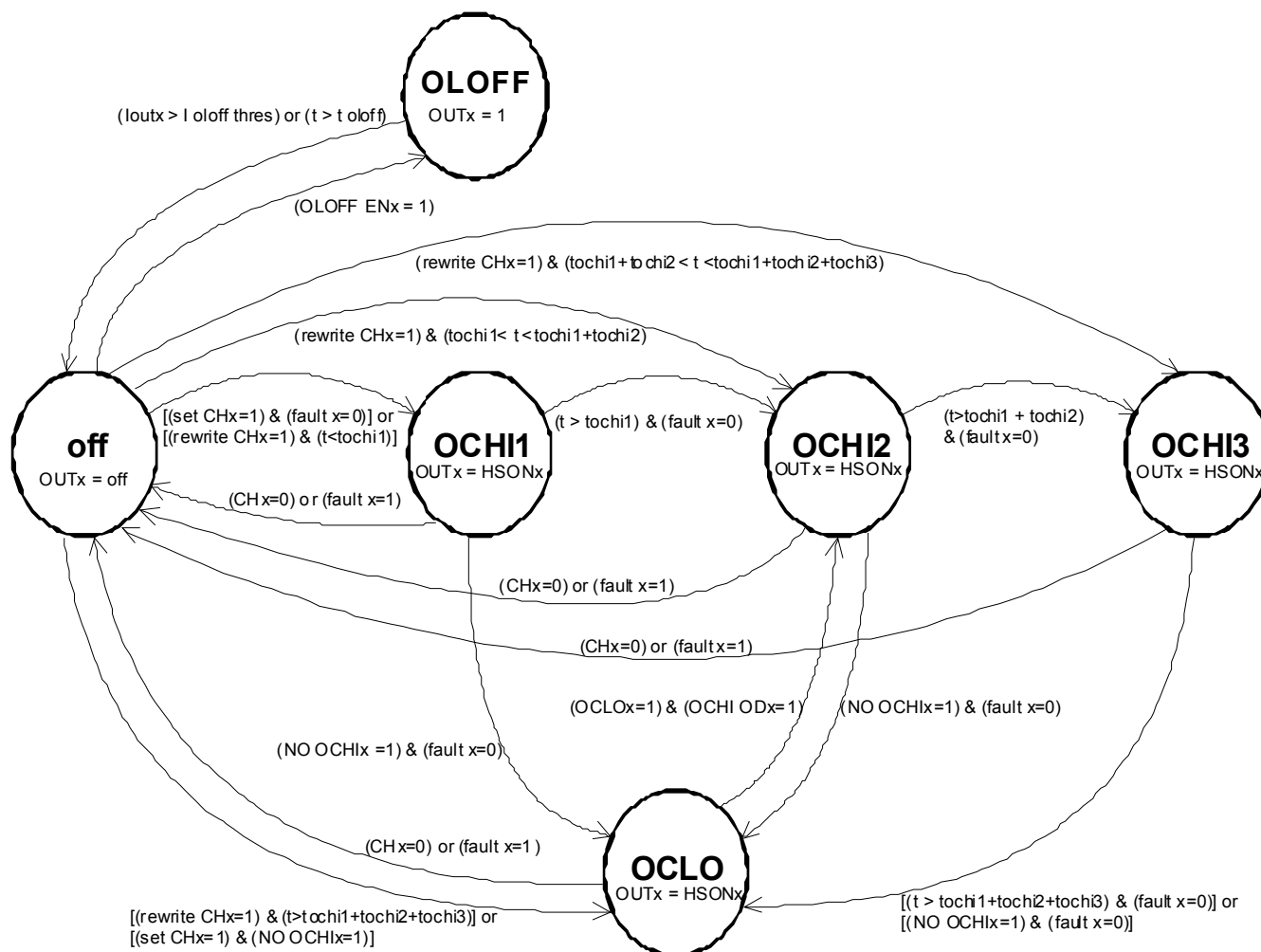
Figure 12. Output Control Diagram in Normal Mode
