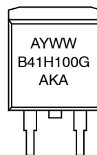
D 2 PAK CASE 418B STYLE 3
