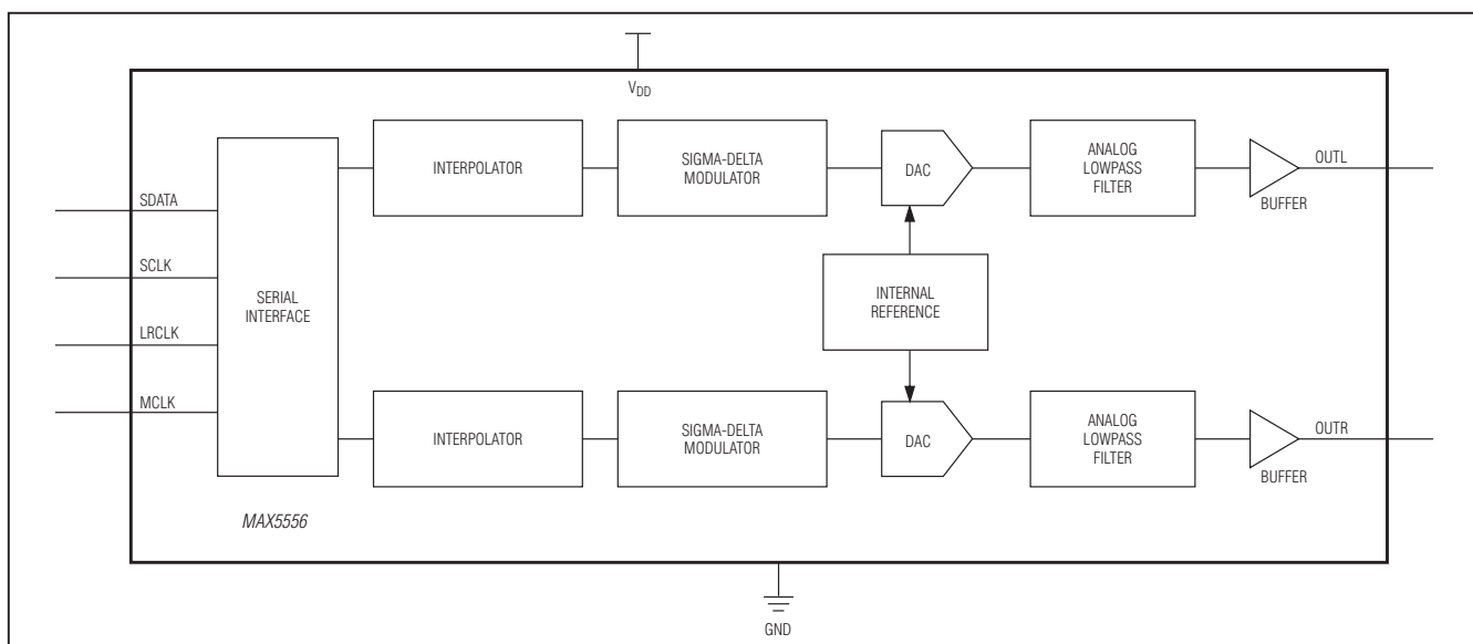
Figure 2. Functional Diagram
