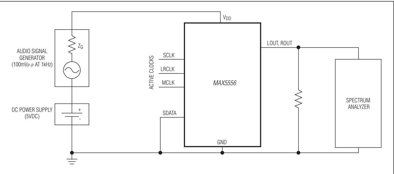
Figure 1. PSRR Test Block Diagram
