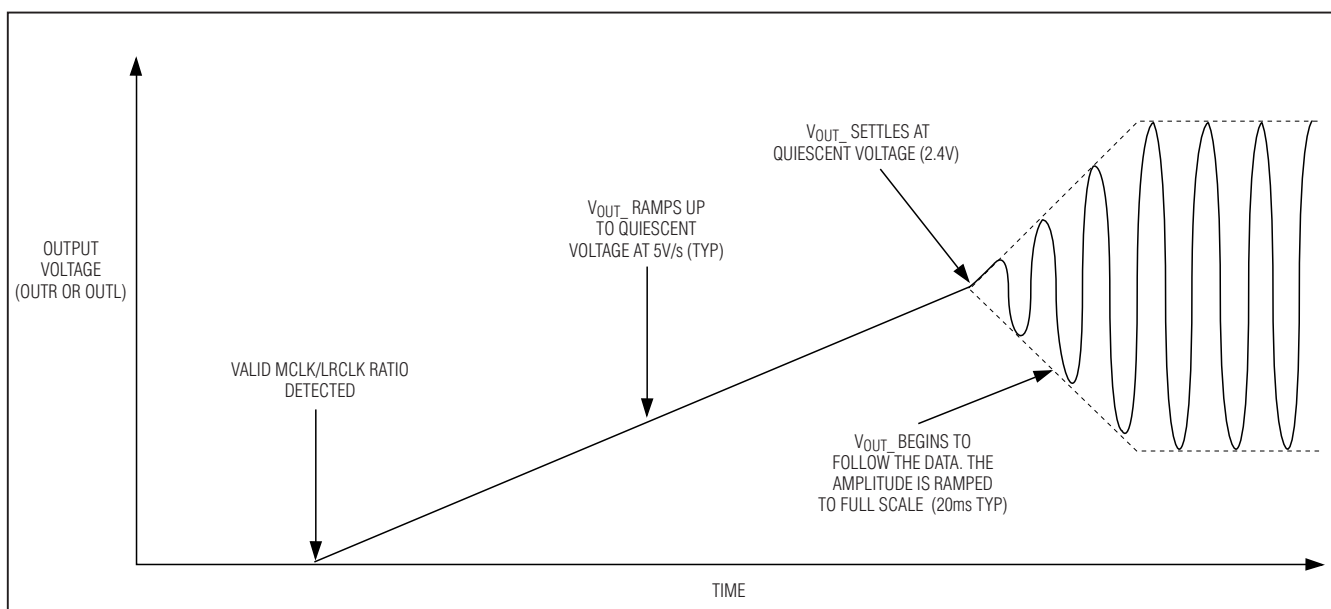
Figure 11. Power-Up Sequence
