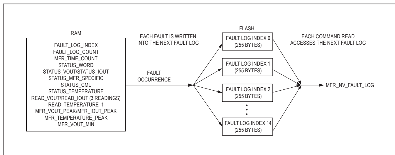
Figure 11. MFR_NV_FAULT_LOG
