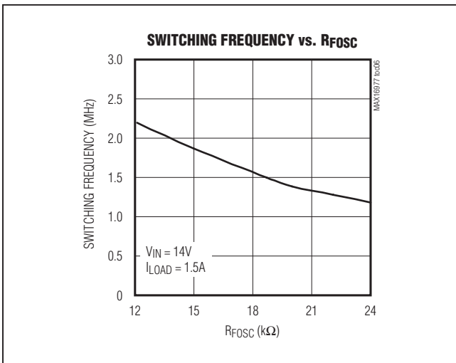
Figure 2. Switching Frequency vs. R_{\text{FOSC}}
