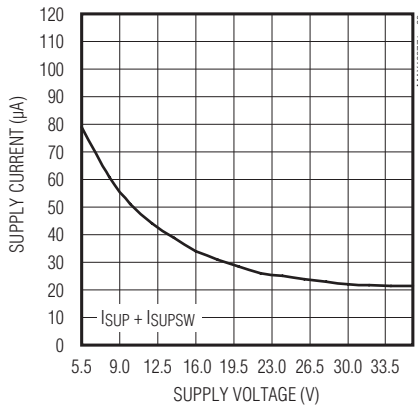
SUPPLY CURRENT vs. SUPPLY VOLTAGE (5V/2.2MHz)
