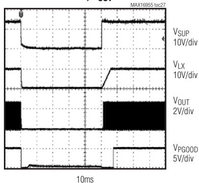
DIPS AND DROPS TEST, PWM MODE, V_{OUT} = 5V
