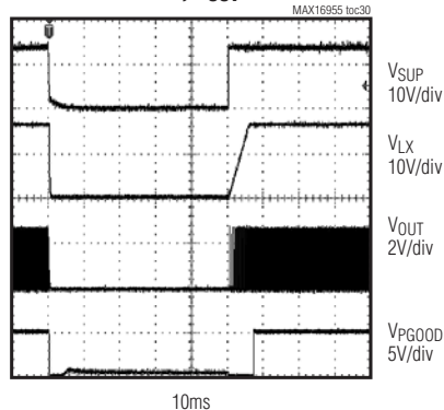
DIPS AND DROPS TEST, SKIP MODE, V_{OUT} = 3.3V
