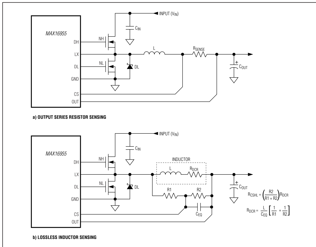
Figure 4. Current-Sense Configurations
