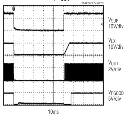
DIPS AND DROPS TEST, SKIP MODE, V_{OUT} = 5V
