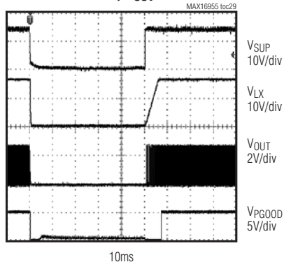
DIPS AND DROPS TEST, PWM MODE, V_{OUT} = 3.3V
