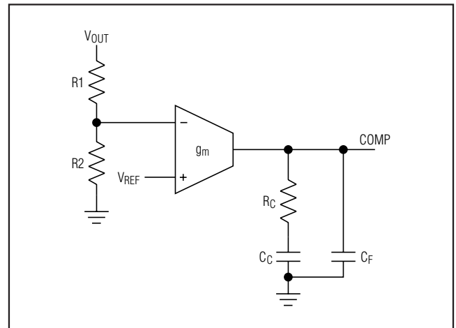
Figure 5. Compensation Network
