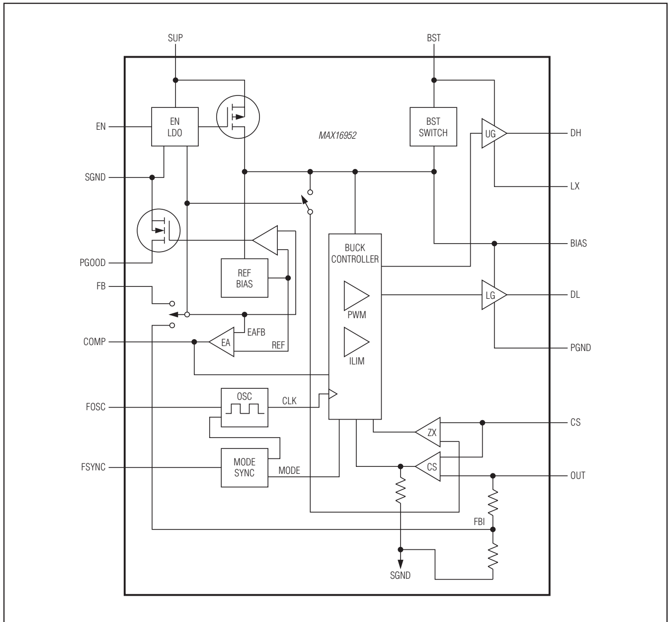
Functional Diagram
