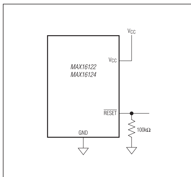
Figure 2. Ensuring \overline{RESET} Output to V_{CC} = 0V
