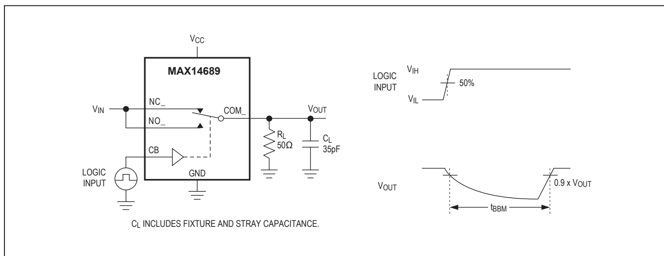
Figure 2. Break-Before-Make Interval
