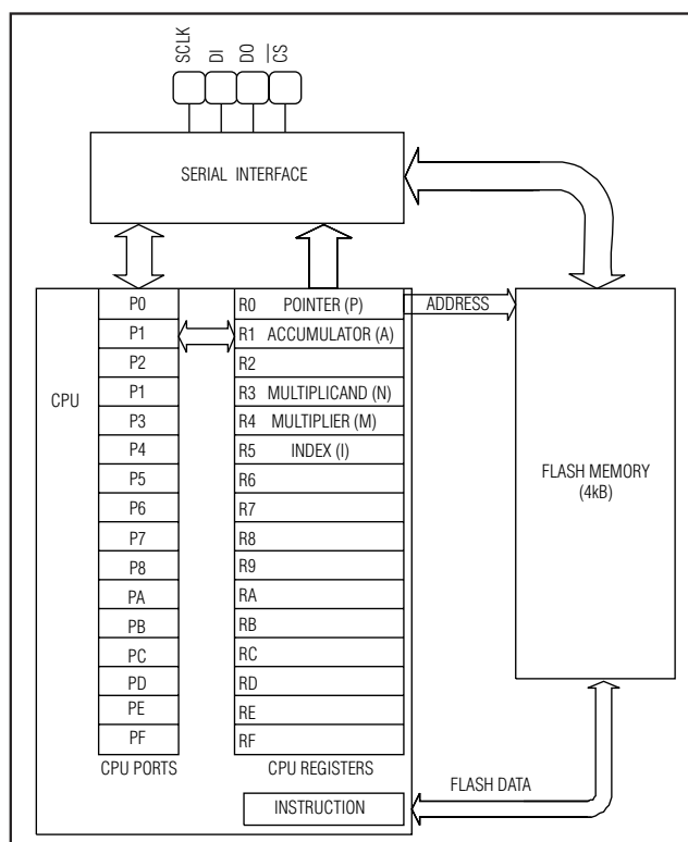
Figure 3. CPU Architecture
