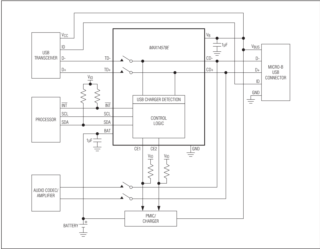
MAX14578E Functional Diagram/Typical Application Circuit
