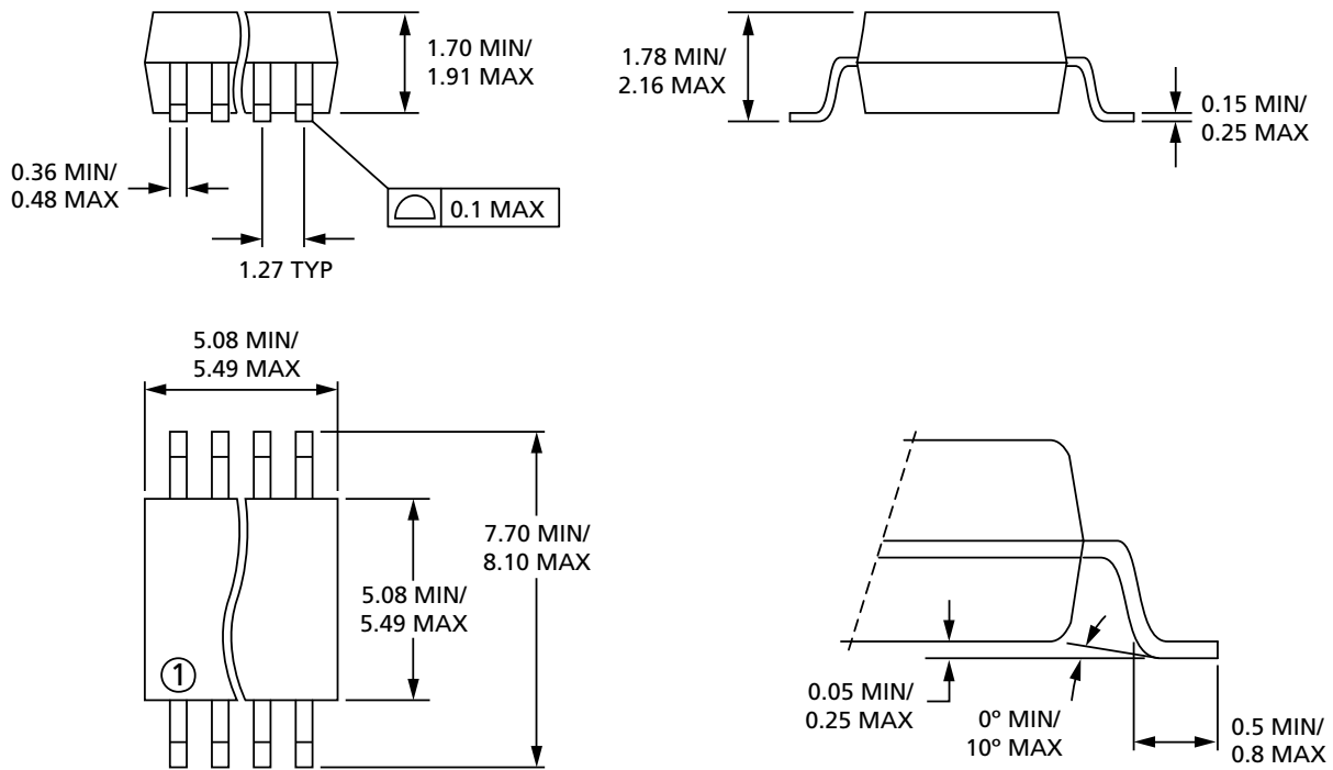
Figure 27: S08W 208 mils Body Width
