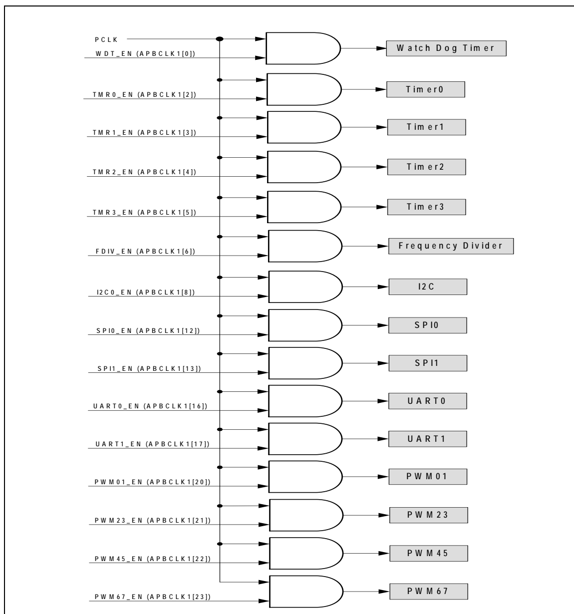
Figure 6-7 Peripherals Clock Source Select for PCLK
