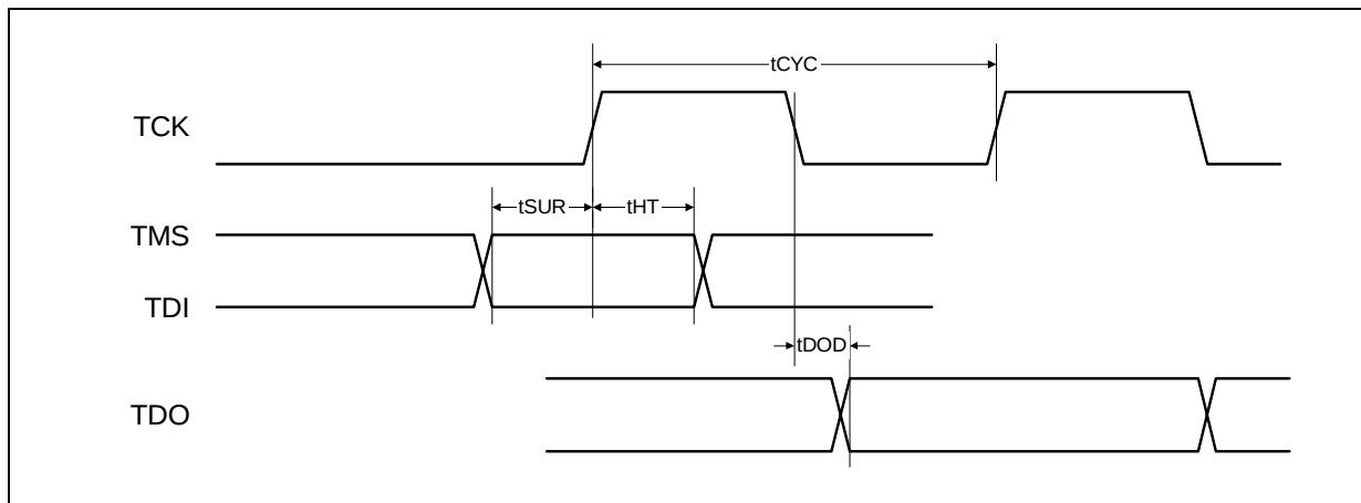
Figure 20. JTAG Timing
