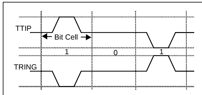
Figure 6. 50% AMI Encoding
