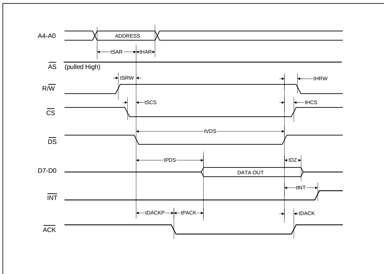
Figure 25. Non-Multiplexed Motorola Mode Read Timing
