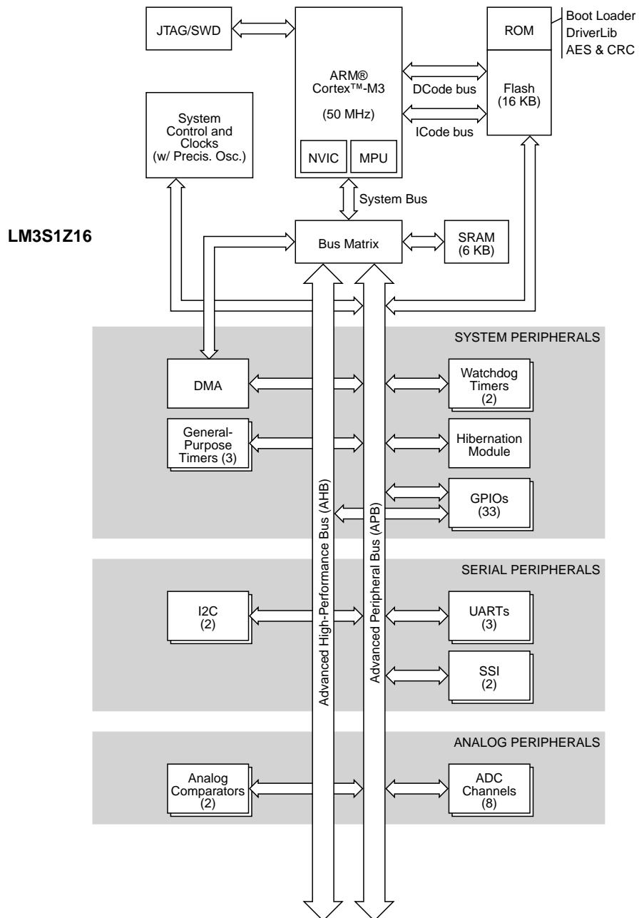
Figure 1-1. Stellaris® LM3S1Z16 Microcontroller High-Level Block Diagram
