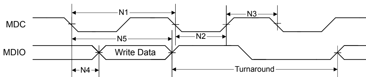
Figure 21-17. Station Management Write Timing
