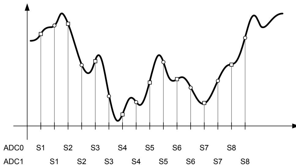
Figure 13-4. Skewed Sampling
