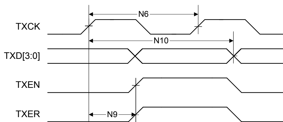
Figure 21-20. MII Transmit Timing
