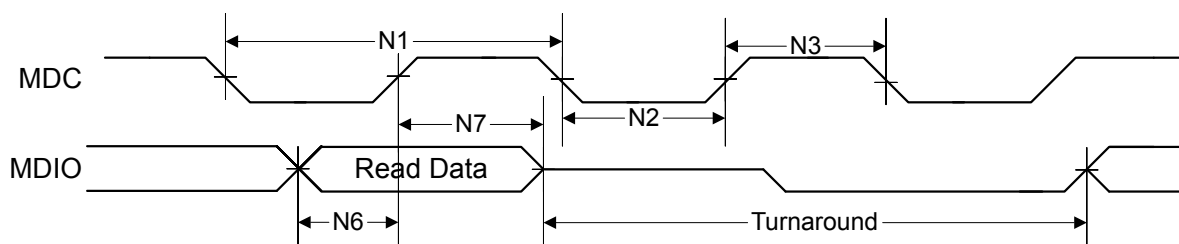
Figure 21-18. Station Management Read Timing
