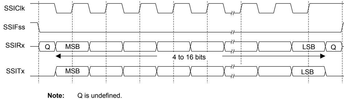
Figure 15-9. Freescale SPI Frame Format with SPO=1 and SPH=1
