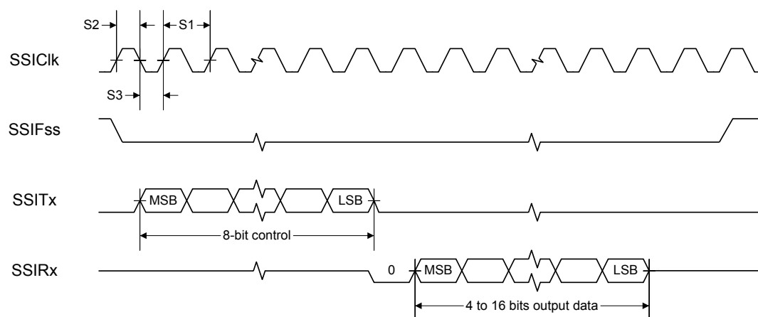
Figure 21-14. SSI Timing for MICROWIRE Frame Format (FRF=10), Single Transfer
