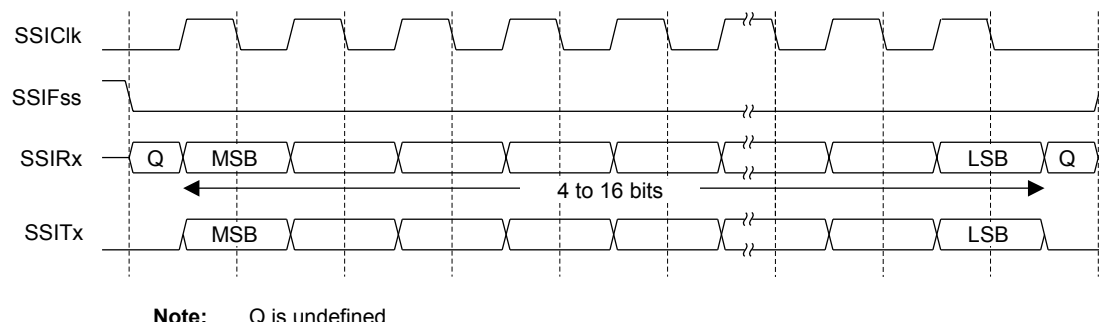
Figure 15-6. Freescale SPI Frame Format with SPO=0 and SPH=1
