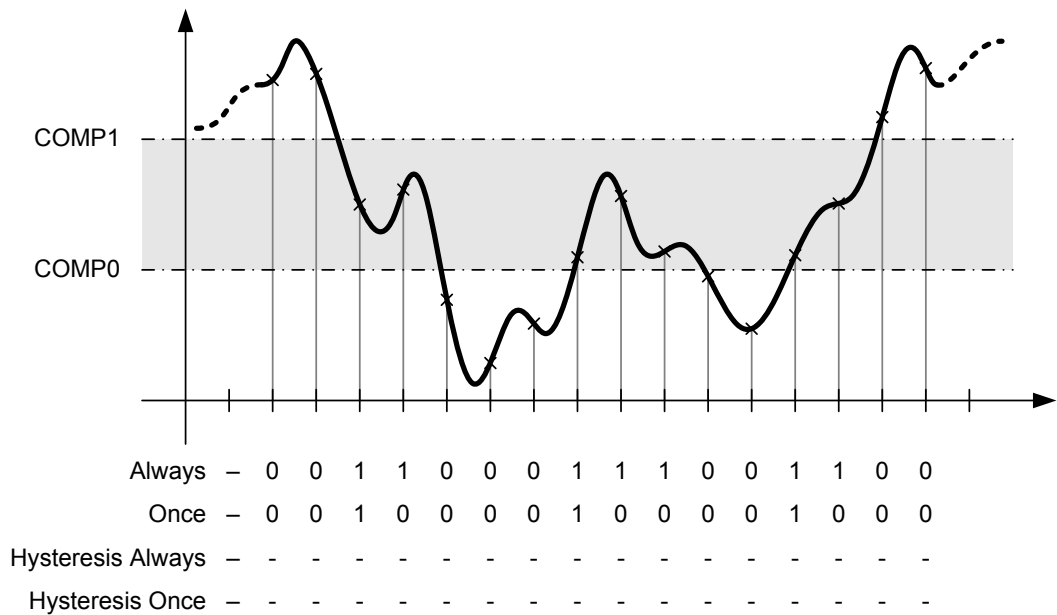
Figure 13-12. Mid-Band Operation (CIC=0x1 and/or CTC=0x1)
