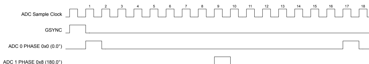
Figure 13-3. Doubling the ADC Sample Rate
