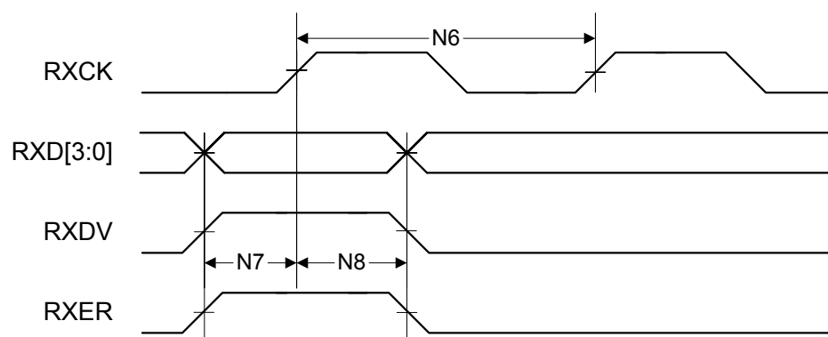
Figure 21-19. MII Receive Timing
