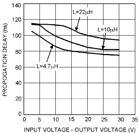
FIGURE 2. Propagation Delay
