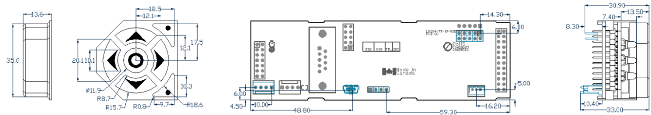
Figure 19: USB Model Dimensional Drawing
