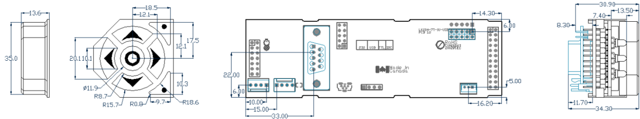
Figure 18: Standard Model Dimensional Drawing
