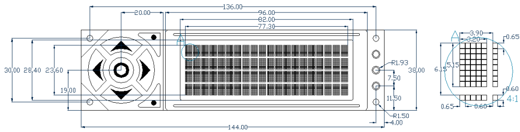
Figure 17: Display Dimensional Drawing
