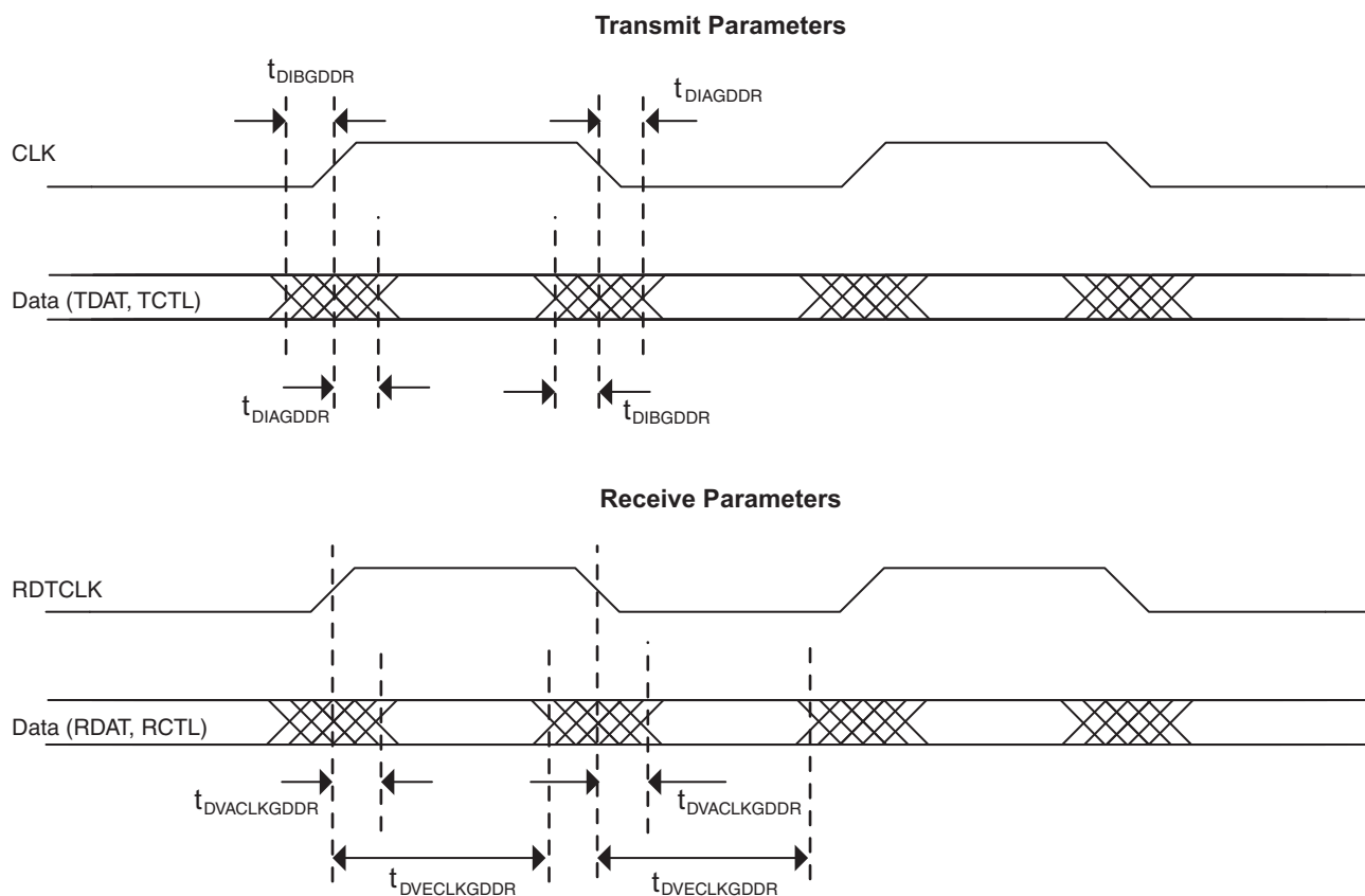
Figure 3-6. Generic DDRX1/DDRX2 (With Clock and Data Edges Aligned)
