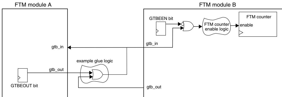
Figure 40-258. Global time base (GTB) block diagram
