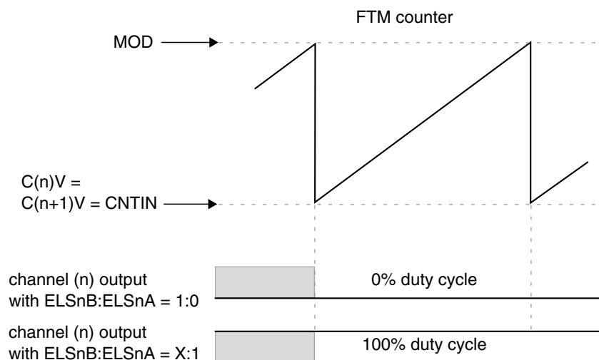
Figure 40-195. Channel (n) output if (C(n)V = C(n+1)V = \text{CNTIN})
