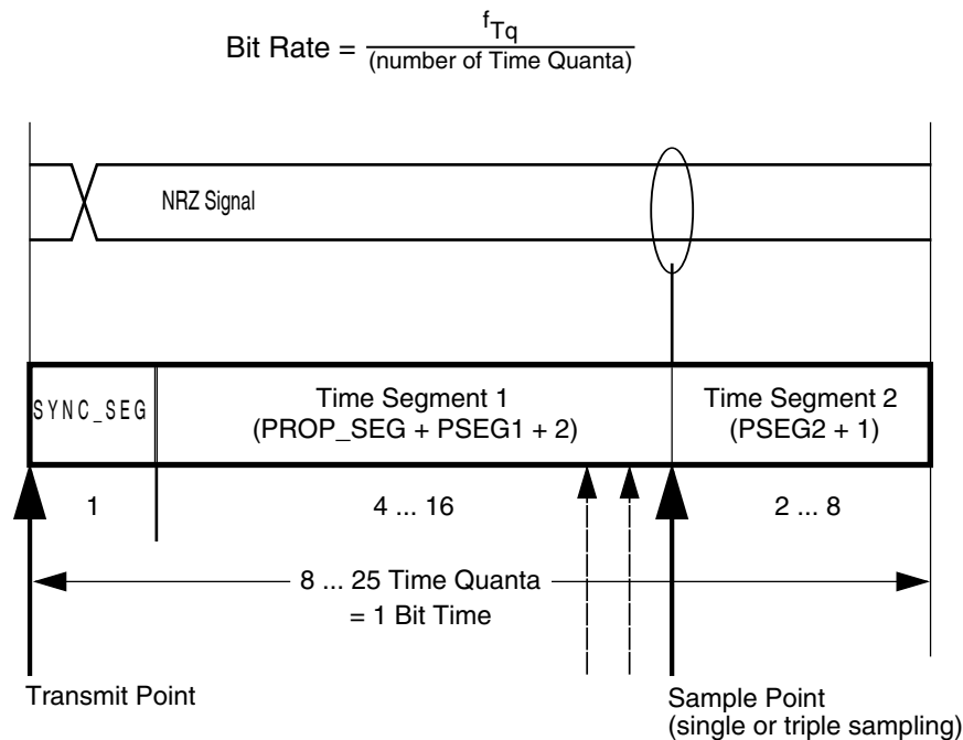
Figure 49-99. Segments within the bit time
