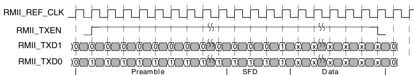
Figure 45-71. RMII transmit operation
