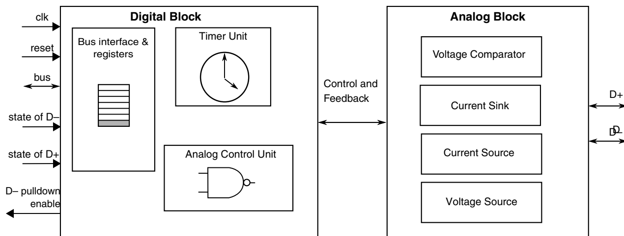
Figure 47-1. Block diagram
