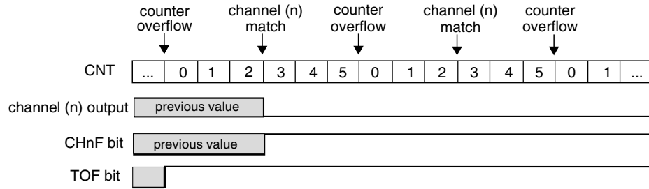
Figure 40-179. Example of the Output Compare mode when the match clears the channel output
