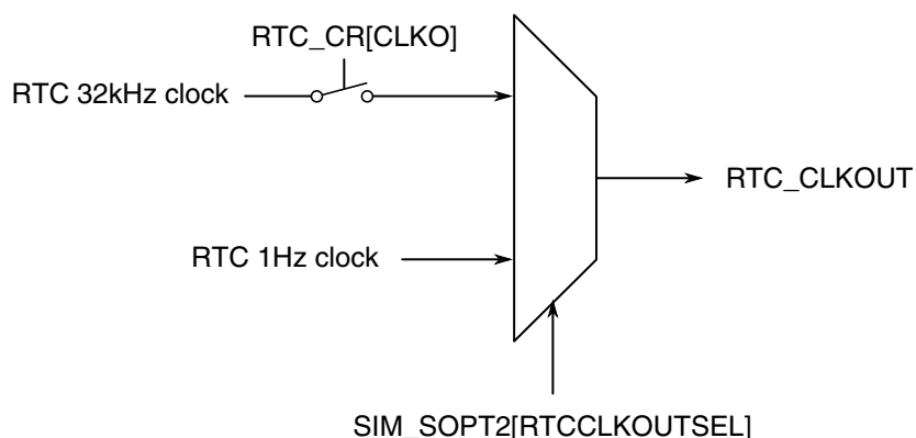
Figure 3-51. RTC_CLKOUT generation
