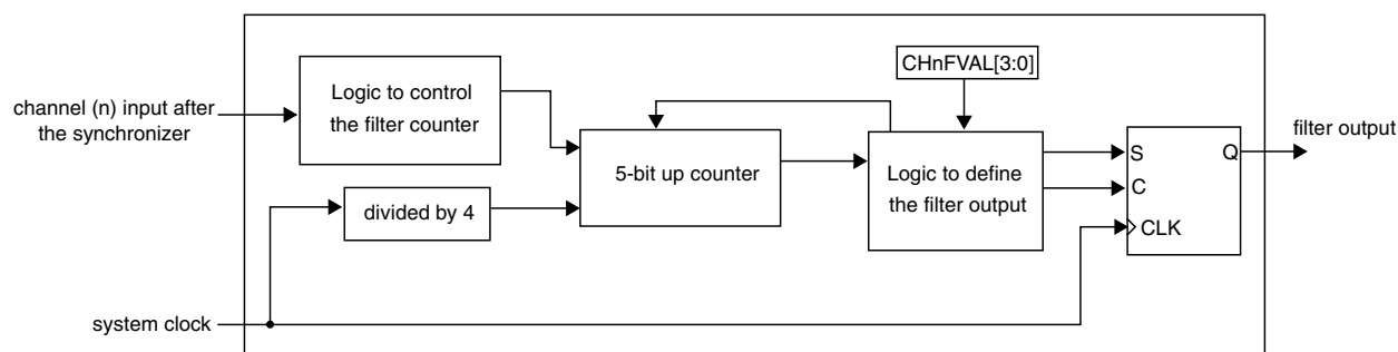
Figure 40-176. Channel input filter
