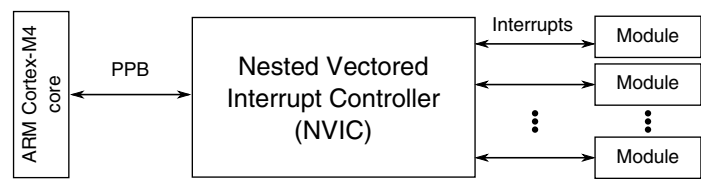
Figure 3-2. NVIC configuration
