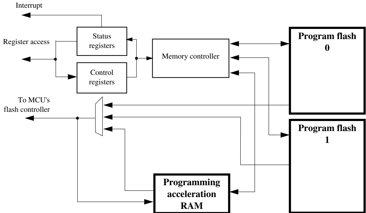
Figure 29-2. Flash Block Diagram
