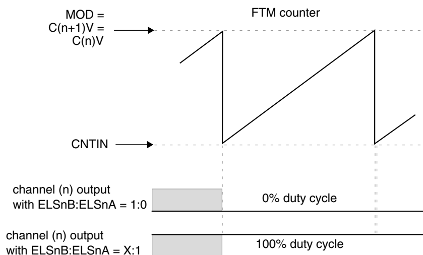
Figure 40-196. Channel (n) output if (C(n)V = C(n+1)V = \text{MOD})
