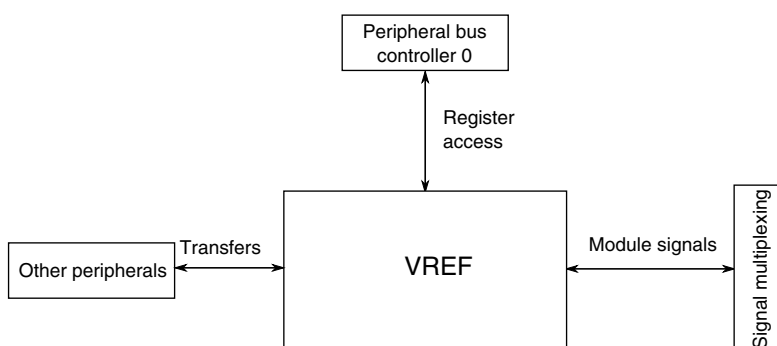
Figure 3-42. VREF configuration
