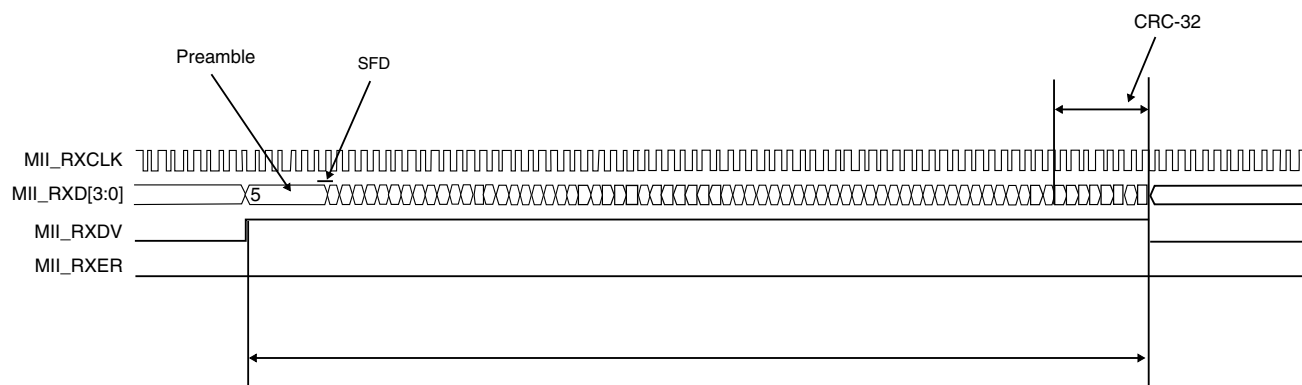
Figure 45-75. MII receive operation
