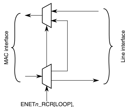
Figure 45-63. Loopback options
