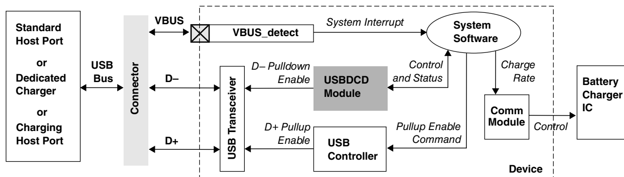
Figure 47-8. USB battery charging subsystem
