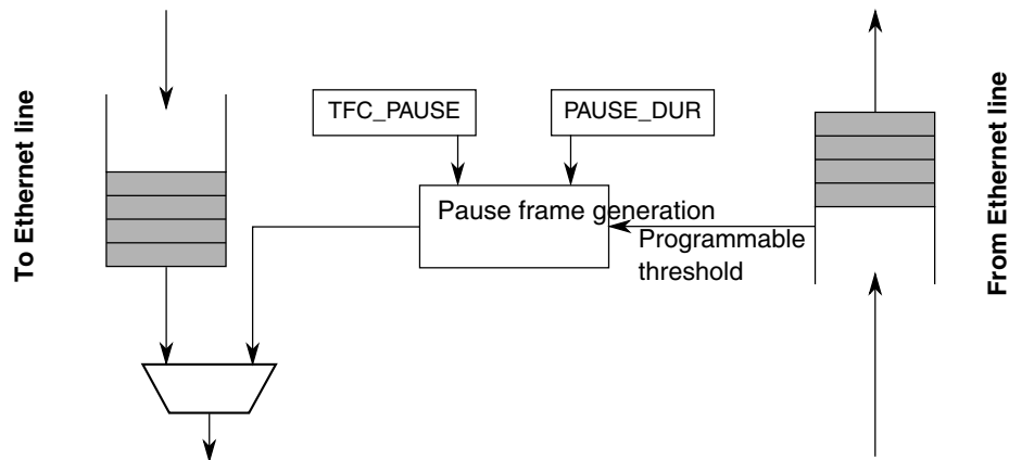
Figure 45-58. Pause frame generation overview
