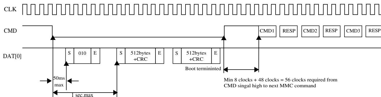
Figure 53-37. Multimediocard state diagram in Normal Boot mode
