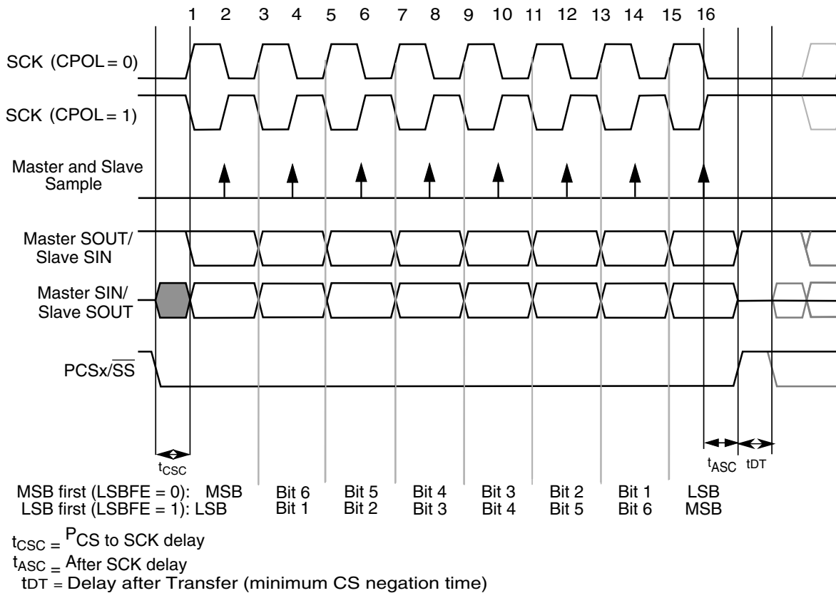
Figure 50-94. Module transfer timing diagram (MTFE=0, CPHA=1, FMSZ=8)
