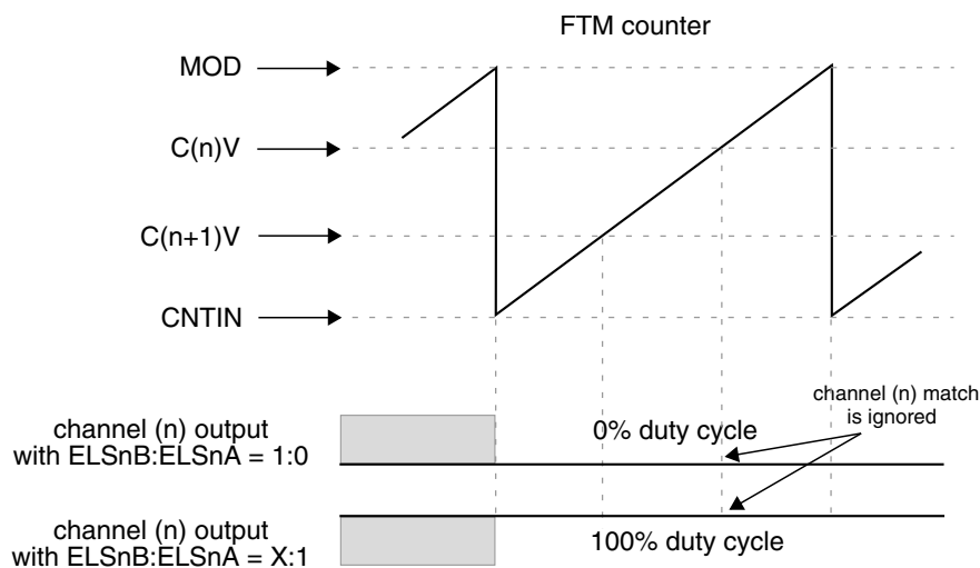
Figure 40-197. Channel (n) output if (\text{CNTIN} < C(n)V < \text{MOD}) and (\text{CNTIN} < C(n+1)V < \text{MOD}) and (C(n)V > C(n+1)V)
