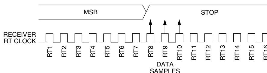
Figure 48-58. Slow data
