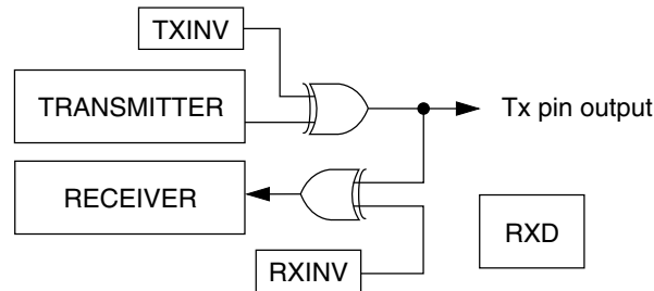
Figure 48-71. Loop operation ( C1[LOOPS] = 1 , C1[RSRC] = 0 )
