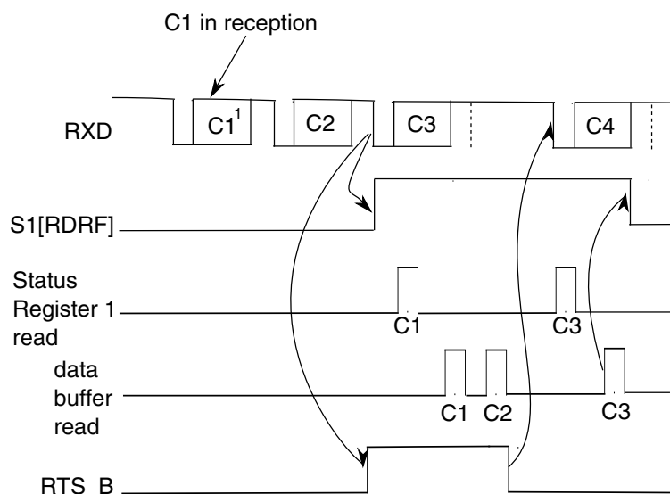
Figure 48-57. Receiver hardware flow control timing diagram
