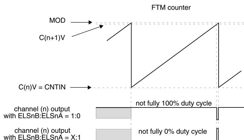
Figure 38-192. Channel (n) output if (C(n)V = CNTIN) and (CNTIN < C(n+1)V < MOD) and (C(n+1)V \text{ is Almost Equal to } MOD)
