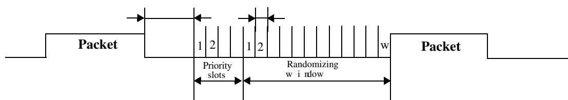
Figure 48-51. CEA709.1-B packet cycle
