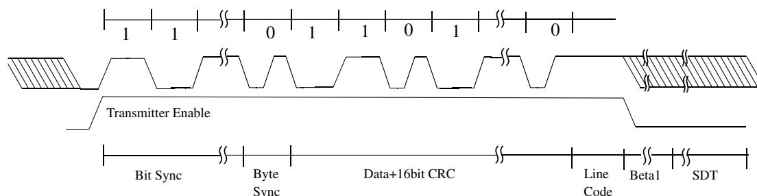
Figure 48-49. Frame format with differential manchester encoding
