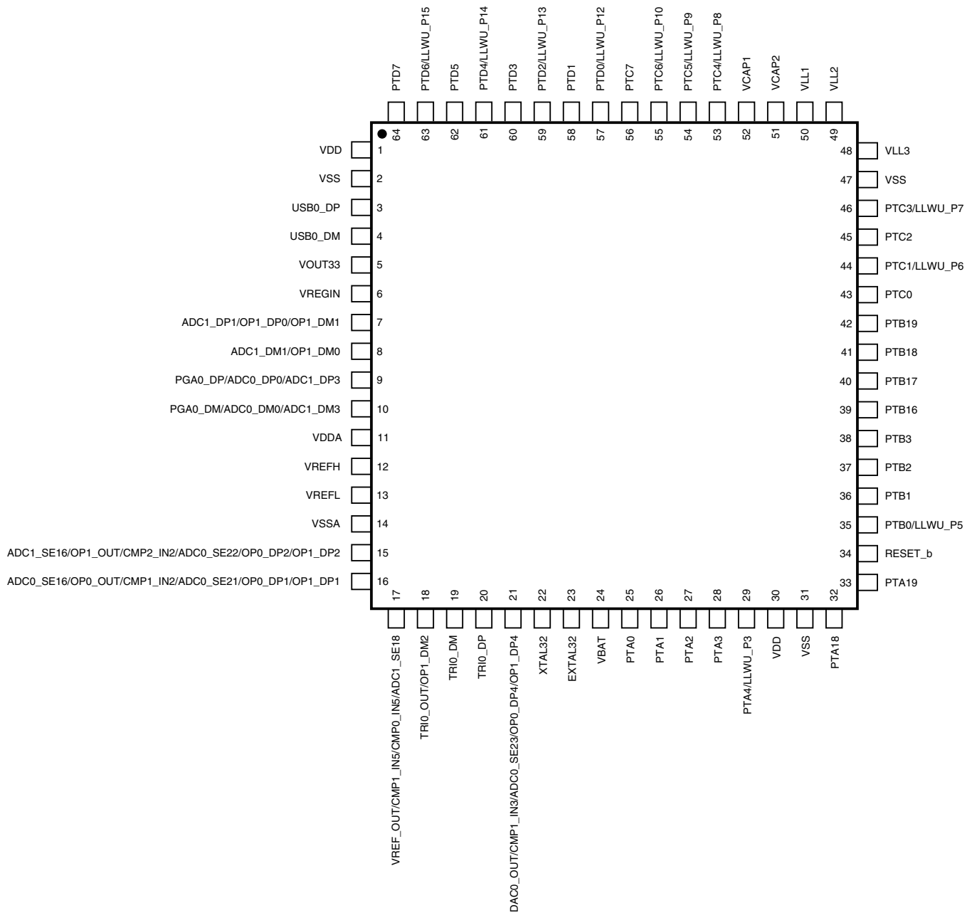
Figure 10-2. K51 64 LQFP/QFN Pinout Diagram
