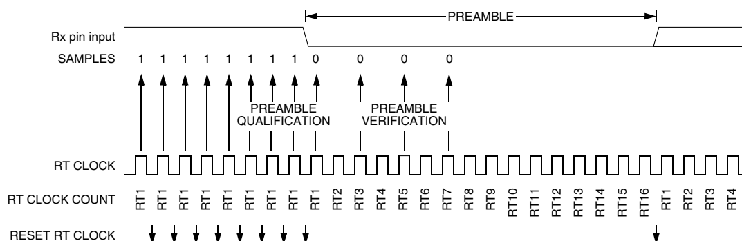
Figure 48-52. Receiver data sampling
