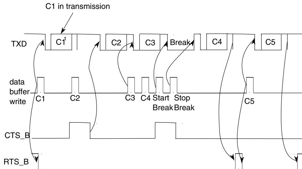
Figure 48-55. Transmitter RTS and CTS timing diagram
