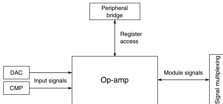
Figure 3-35. Op-amp configuration
