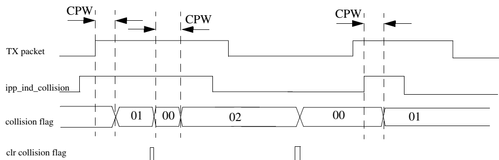
Figure 48-53. Collision pulse detection
