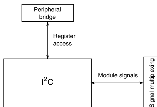
Figure 3-55. I2C configuration
