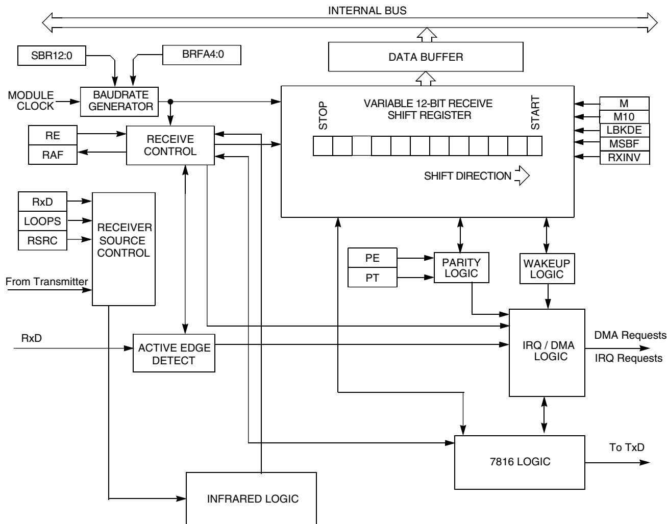
Figure 48-56. UART receiver block diagram
