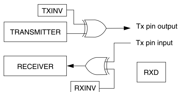
Figure 48-70. Single-wire operation (C1[LOOPS] = 1, C1[RSRC] = 1)
