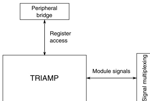
Figure 3-39. TRIAMP configuration
