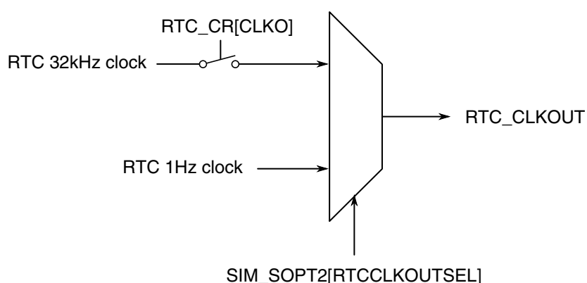
Figure 3-49. RTC_CLKOUT generation
