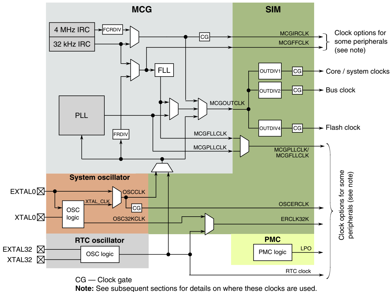
Figure 5-1. Clocking diagram
