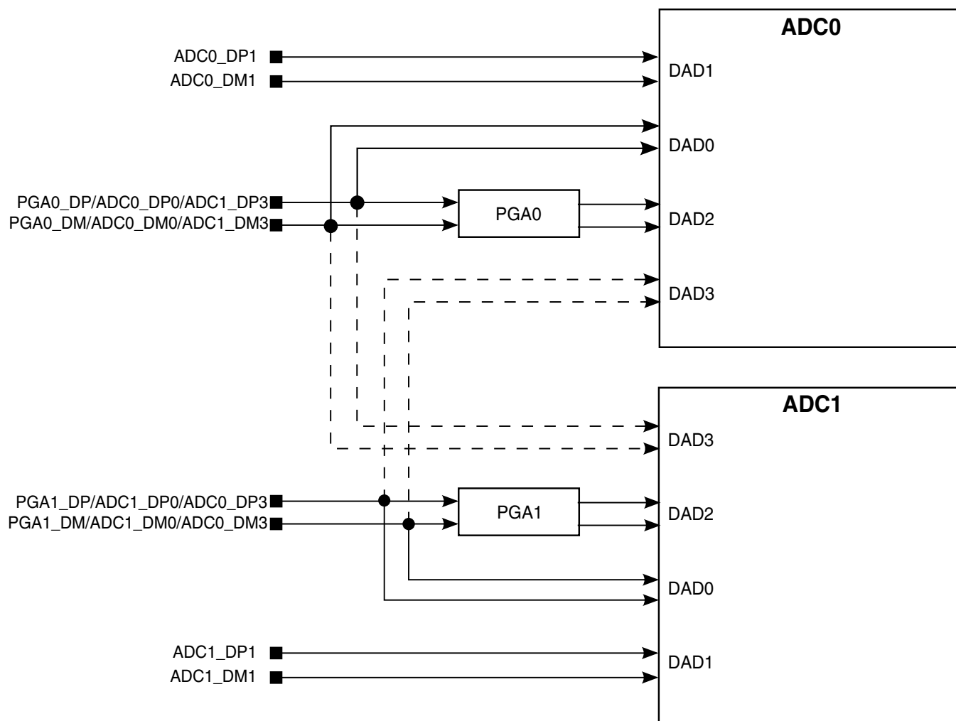
Figure 3-35. PGA Integration
