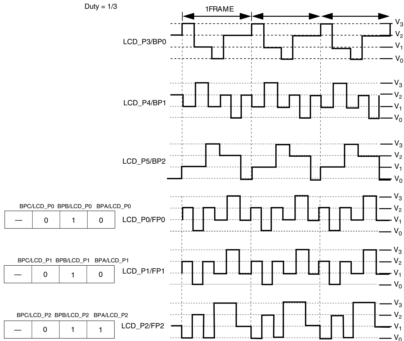
Figure 54-40. LCD waveforms
