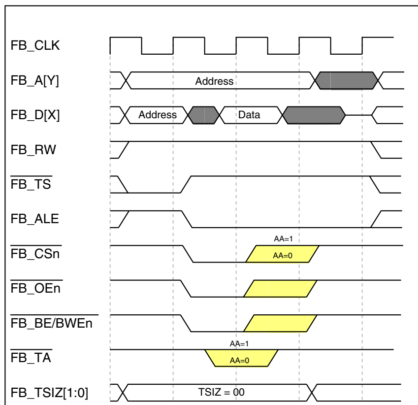
Figure 29-33. Longword-Read Transfer
