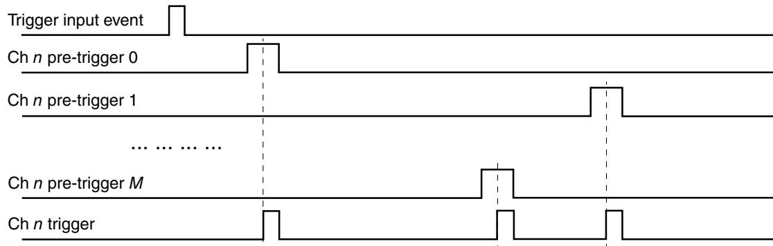
Figure 38-52. Pre-trigger and trigger outputs
