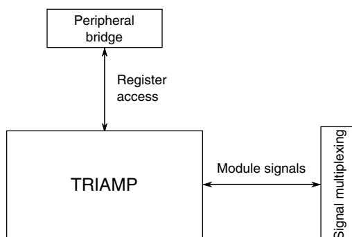
Figure 3-38. TRIAMP configuration
