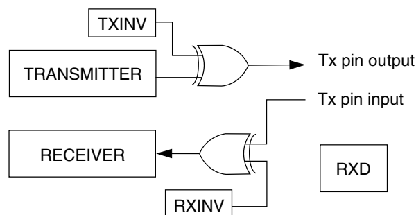
Figure 49-262. Single-wire operation (C1[LOOPS] = 1, C1[RSRC] = 1)
