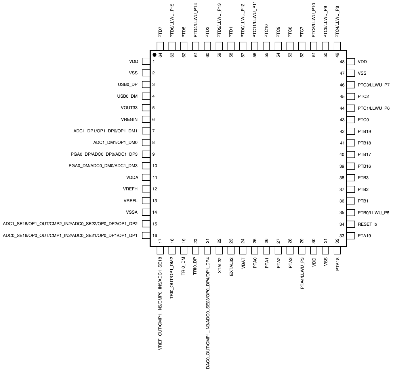
Figure 10-2. K50 64 LQFP/QFN Pinout Diagram
