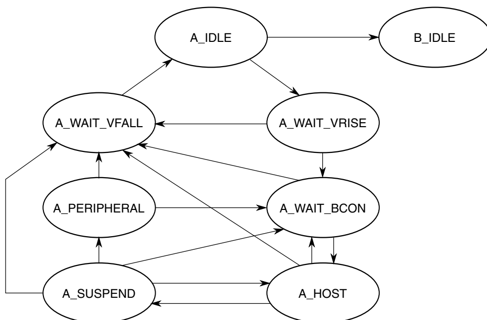
Figure 44-93. Dual role A device flow diagram
