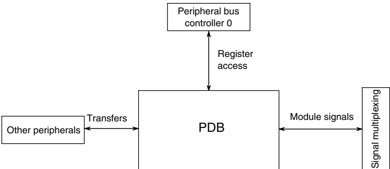
Figure 3-40. PDB configuration
