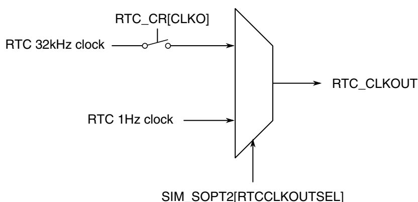
Figure 3-48. RTC_CLKOUT generation
