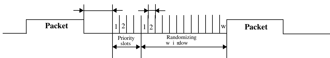
Figure 49-51. CEA709.1-B packet cycle
