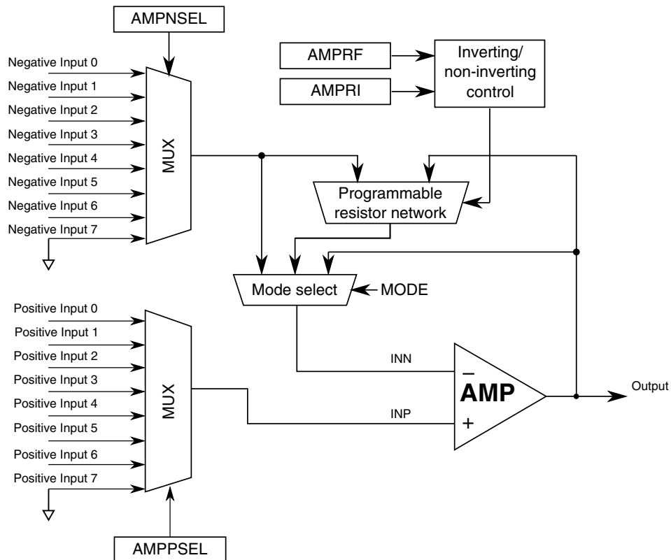
Figure 35-1. Op-Amp Block Diagram
