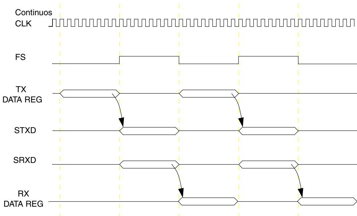
Figure 51-46. Normal mode timing - continuous clock
