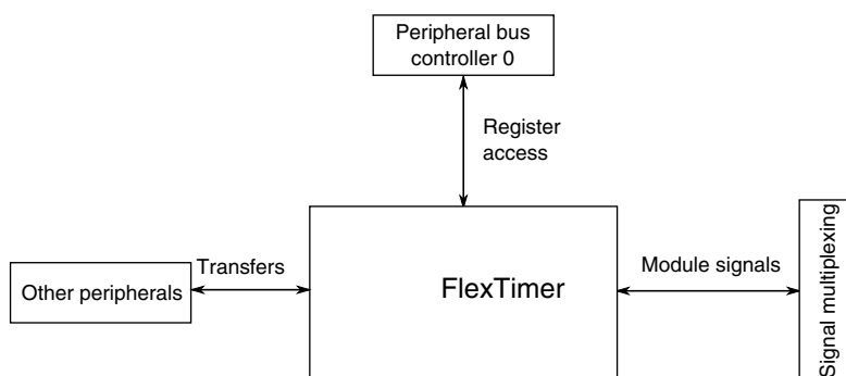
Figure 3-44. FlexTimer configuration
