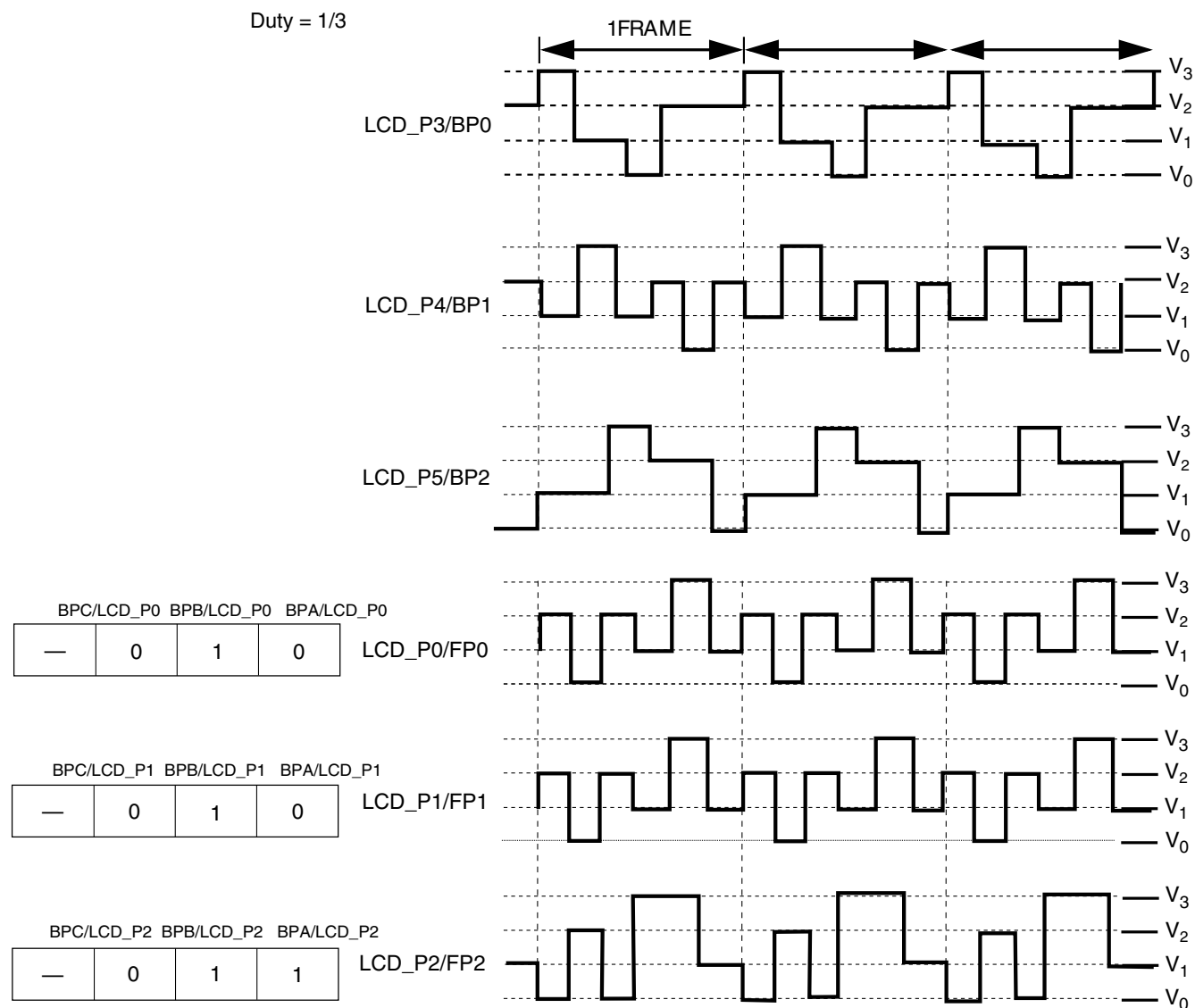
Figure 51-40. LCD waveforms
