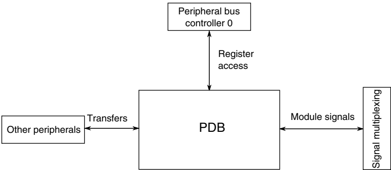
Figure 3-36. PDB configuration
