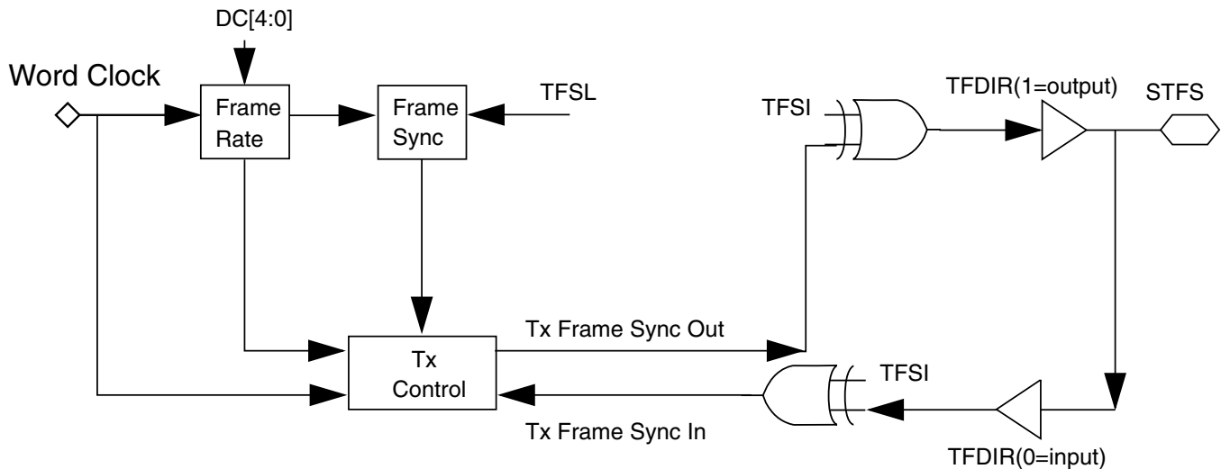
Figure 49-57. I²S transmit frame sync generator block diagram
