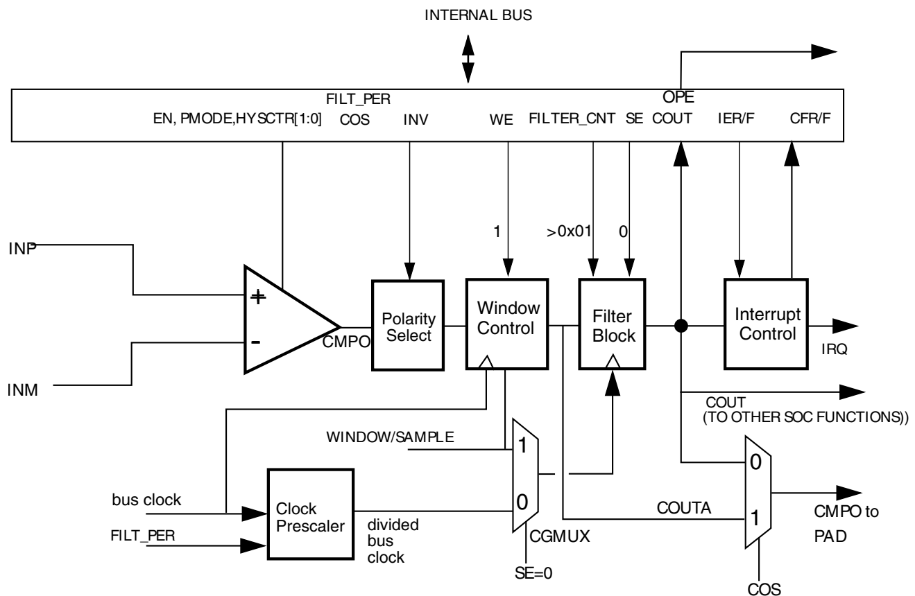
Figure 32-35. Windowed/Filtered Mode
