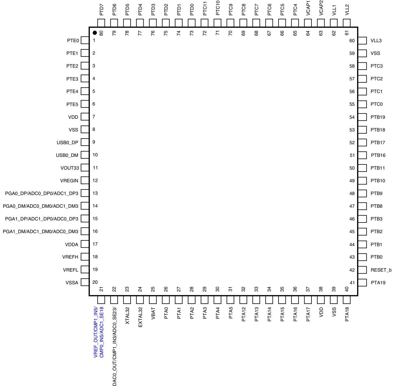
Figure 10-3. K40 80 LQFP Pinout Diagram
