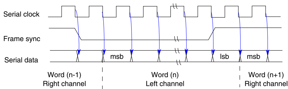
Figure 49-54. I 2 S mode timing - serial clock, frame sync and serial data
