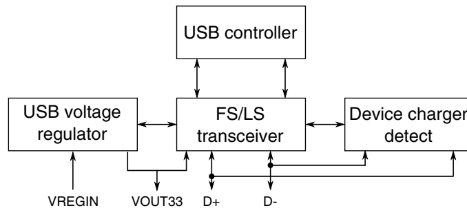
Figure 3-46. USB Subsystem Overview
