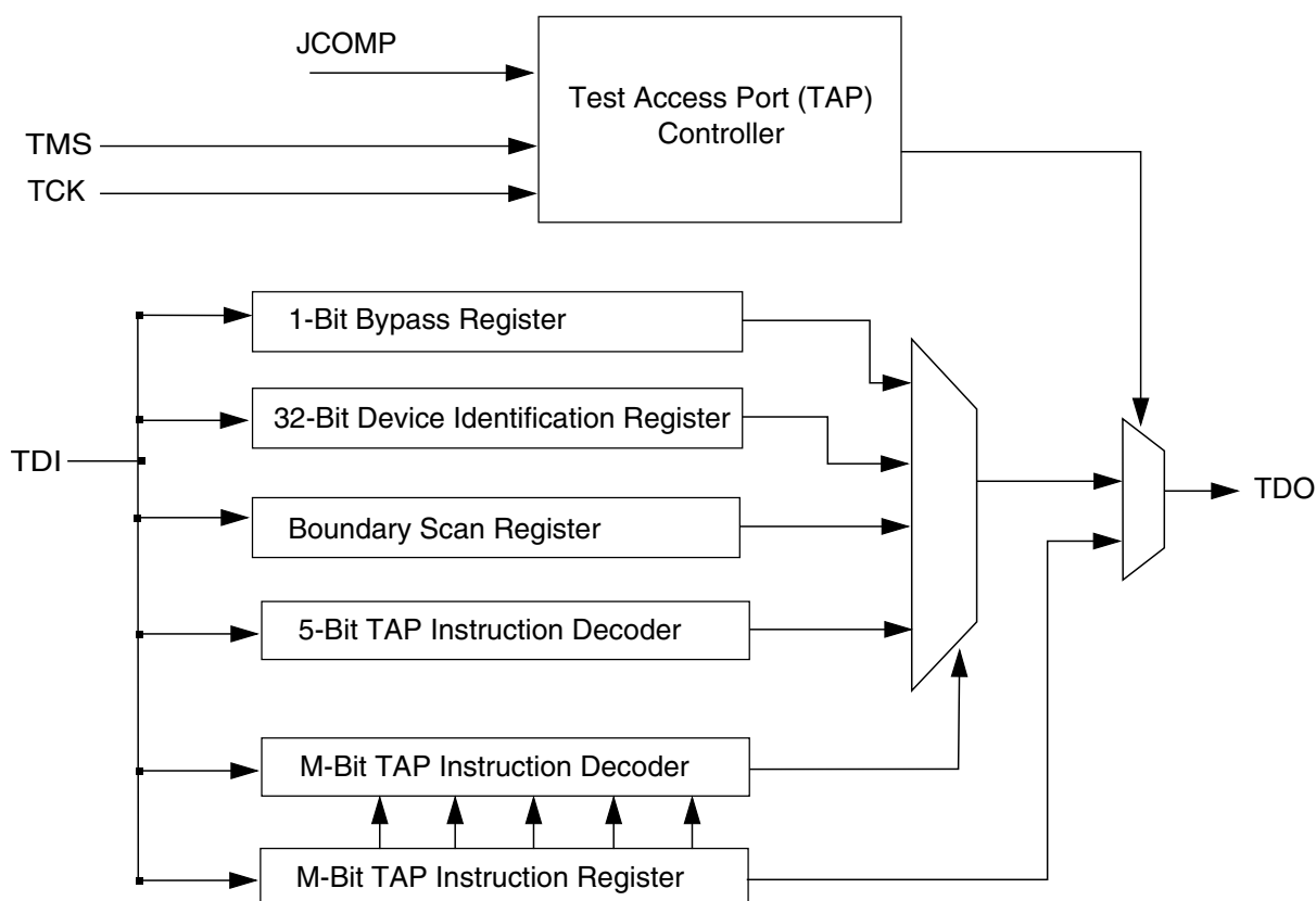
Figure 53-1. JTAG STL (IEEE 1149.1) Block Diagram
