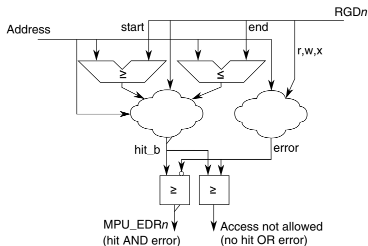
Figure 18-100. MPU Access Evaluation Macro
