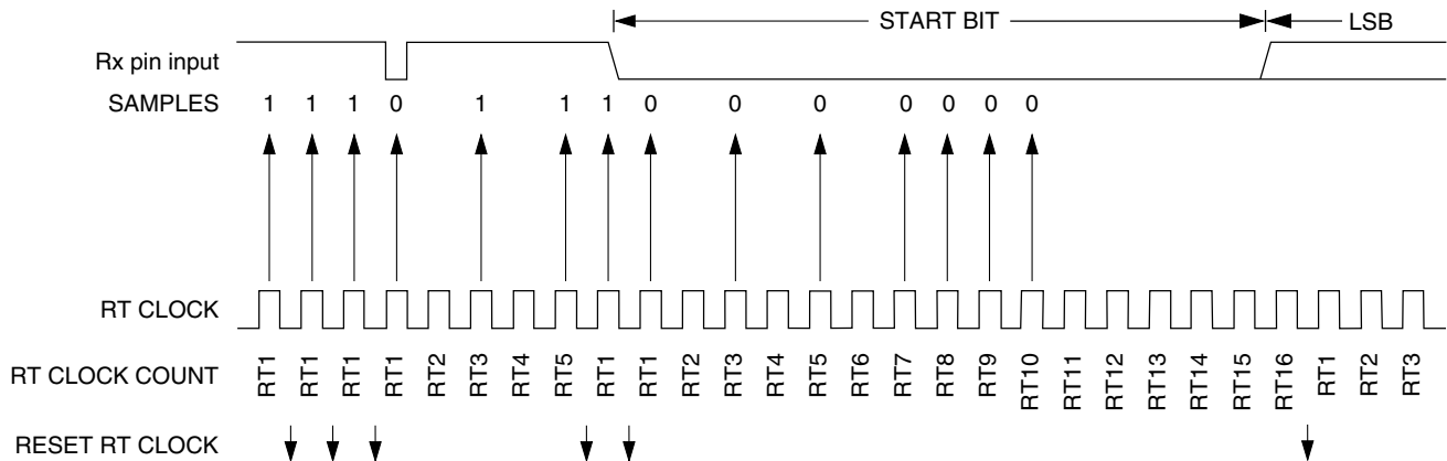
Figure 47-160. Start bit search example 1 ( C7816[ISO\_7816E] = 0 )
