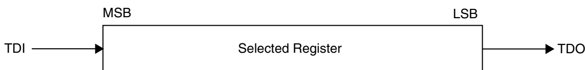
Figure 53-2. Shifting Data Through a Register
