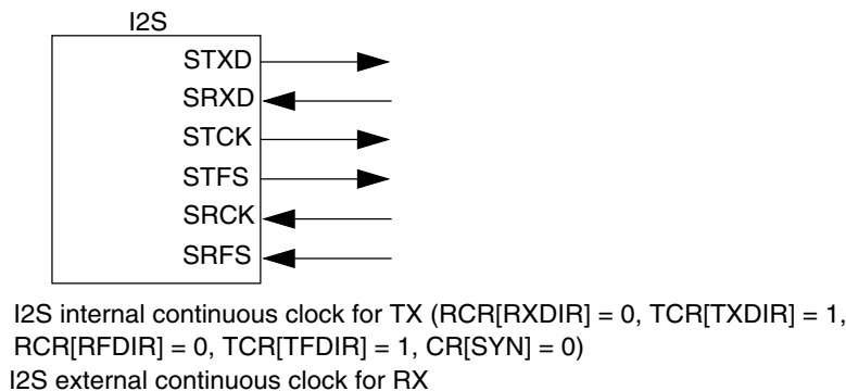
Figure 49-2. Asynchronous (SYN = 0) I 2 S configurations—continuous clock
