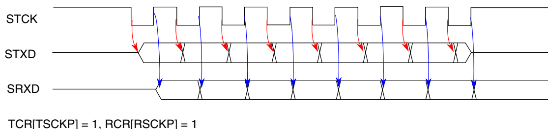
Figure 49-53. External gated mode timing - falling edge clocking/rising edge latching
