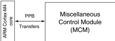
Figure 3-9. MCM configuration
