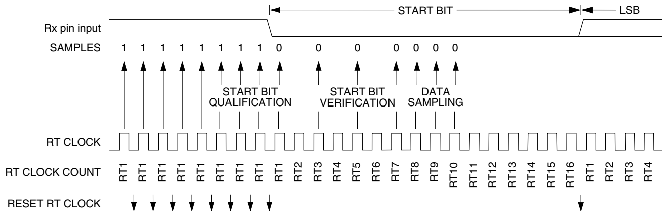
Figure 47-159. Receiver data sampling
