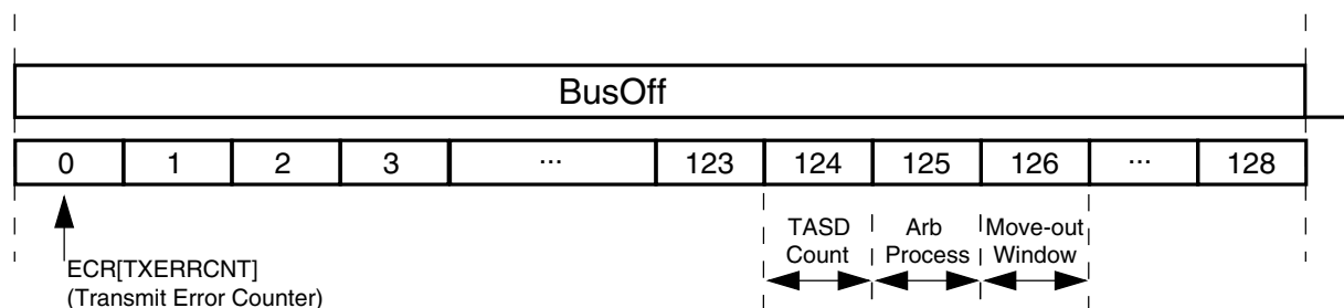
Figure 44-74. Arbitration at the end of Bus Off and Move-Out Time Windows
