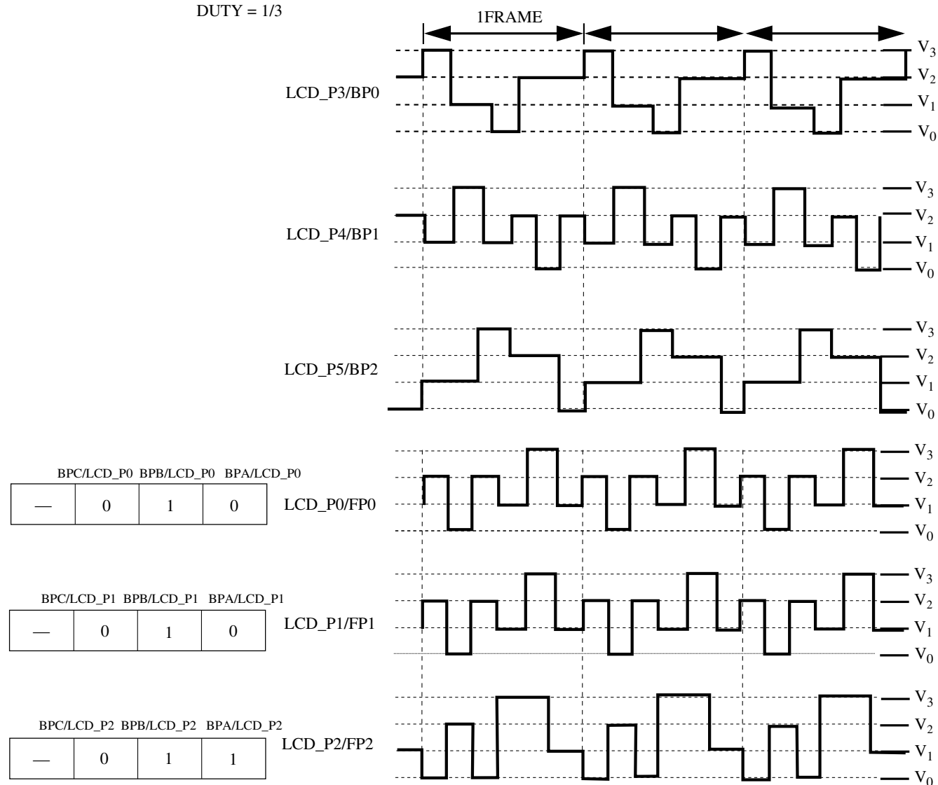
Figure 52-40. LCD waveforms
