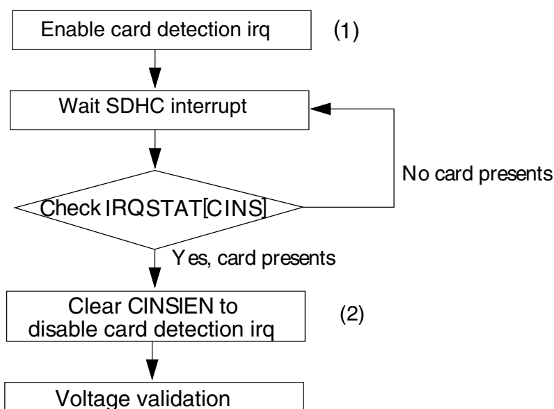
Figure 48-39. Flow diagram for card detection
