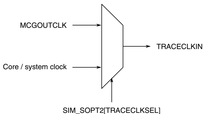
Figure 5-3. Trace clock generation
