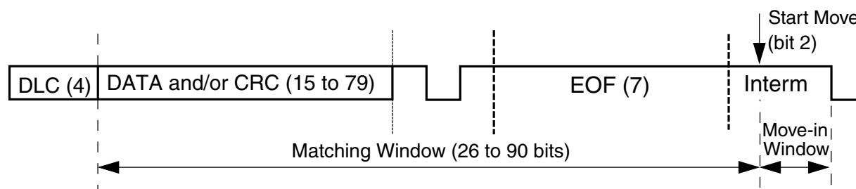
Figure 44-72. Matching and Move-In Time Windows
