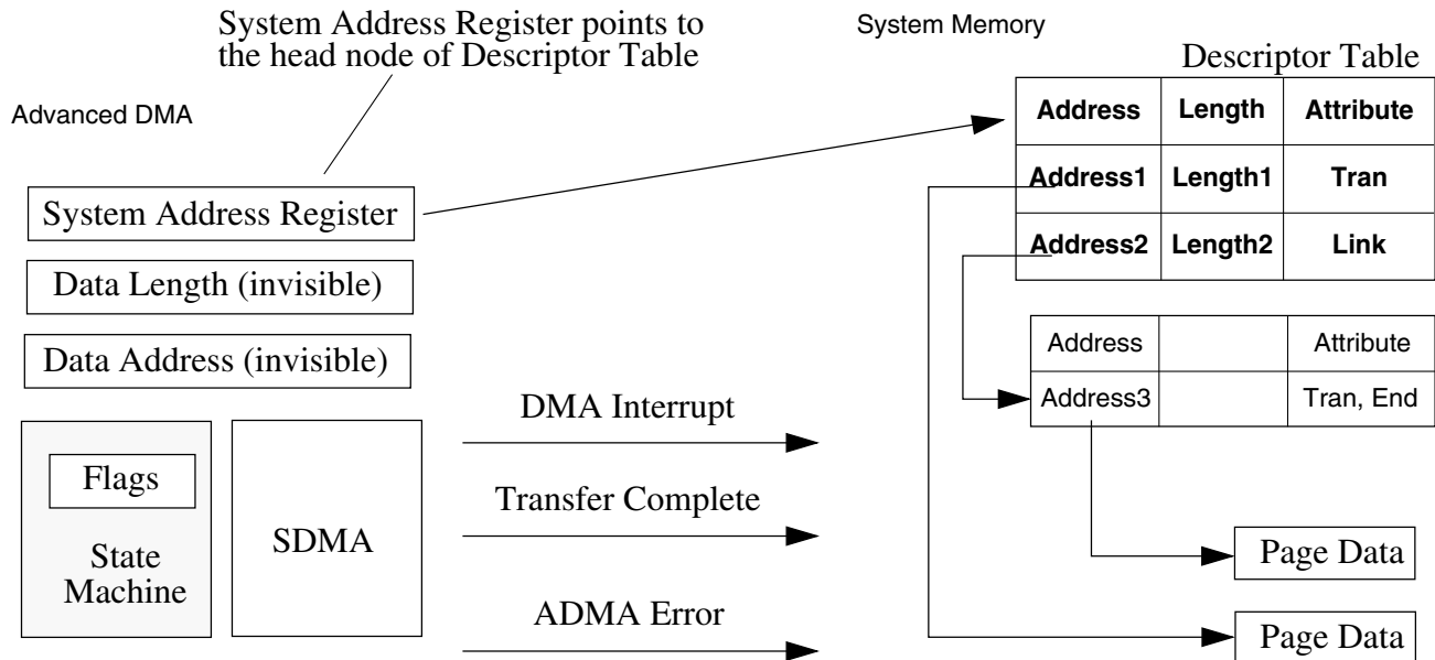
Figure 48-33. Concept and access method of ADMA2 descriptor table
