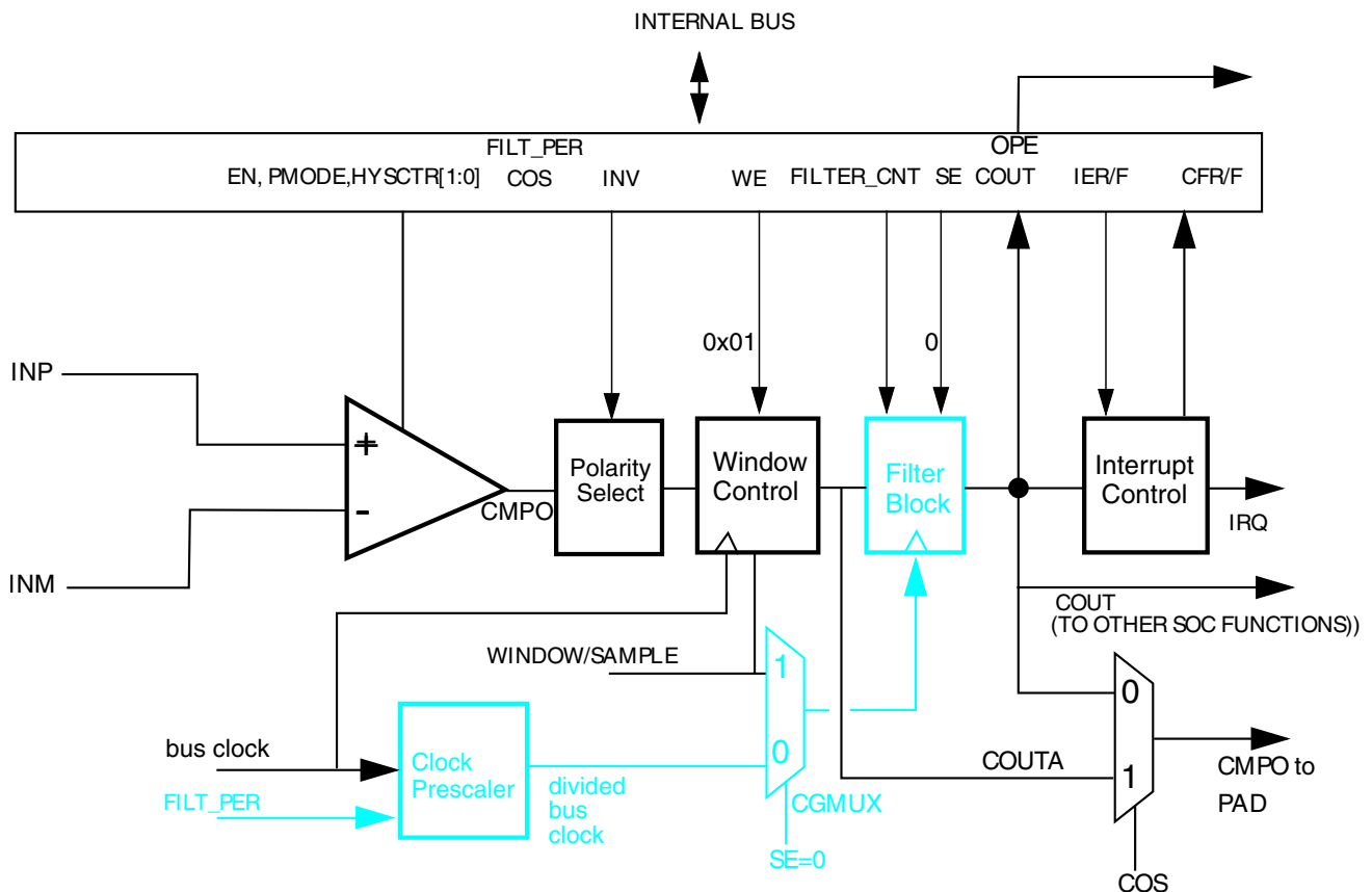
Figure 32-33. Windowed Mode
