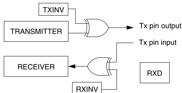
Figure 47-179. Single-wire operation (C1[LOOPS] = 1, C1[RSRC] = 1)
