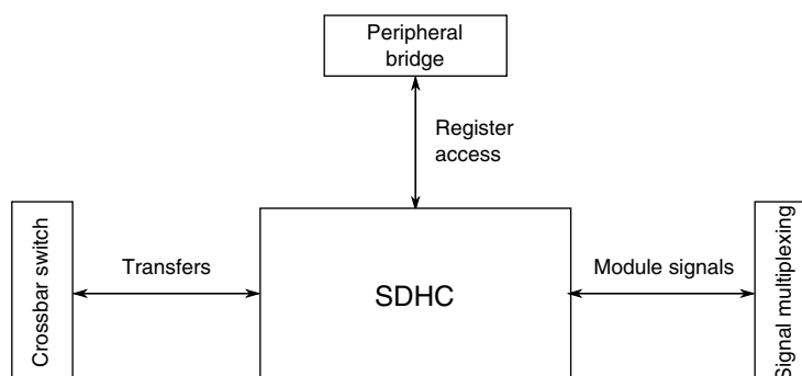
Figure 3-57. SDHC configuration
