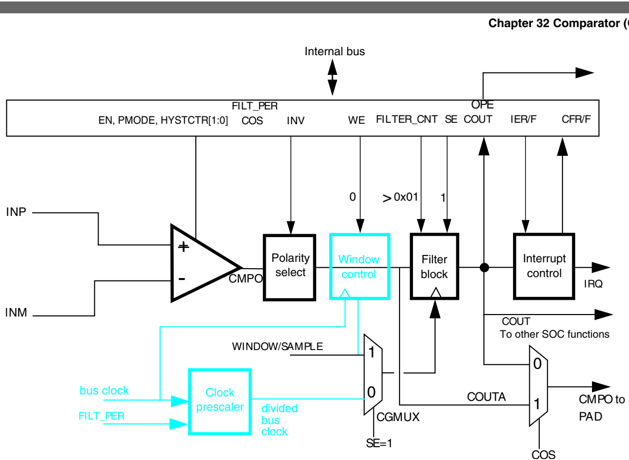
Figure 32-30. Sampled, Filtered (# 4A): sampling point externally driven
