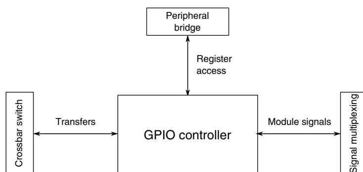
Figure 3-57. GPIO configuration
