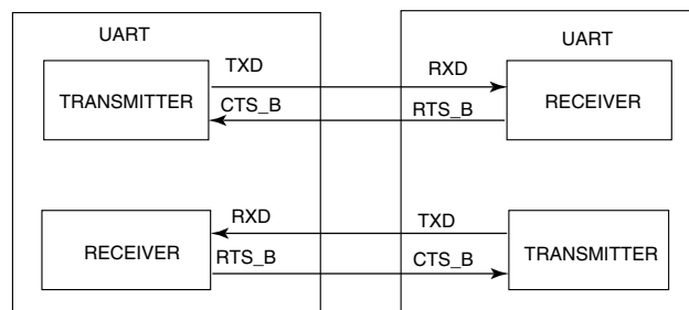
Figure 47-74. Ready-to-receive
