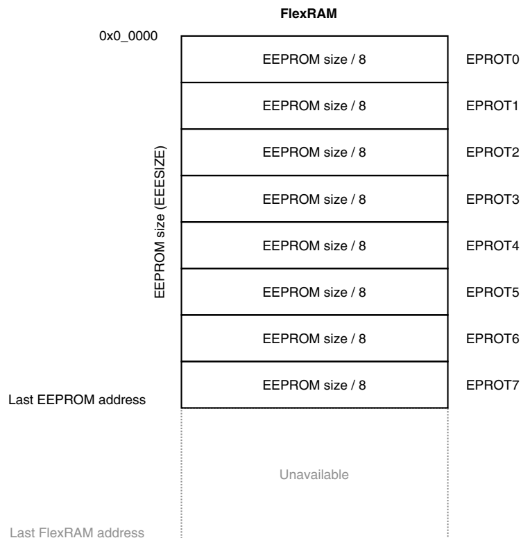
Figure 28-28. EEPROM protection
