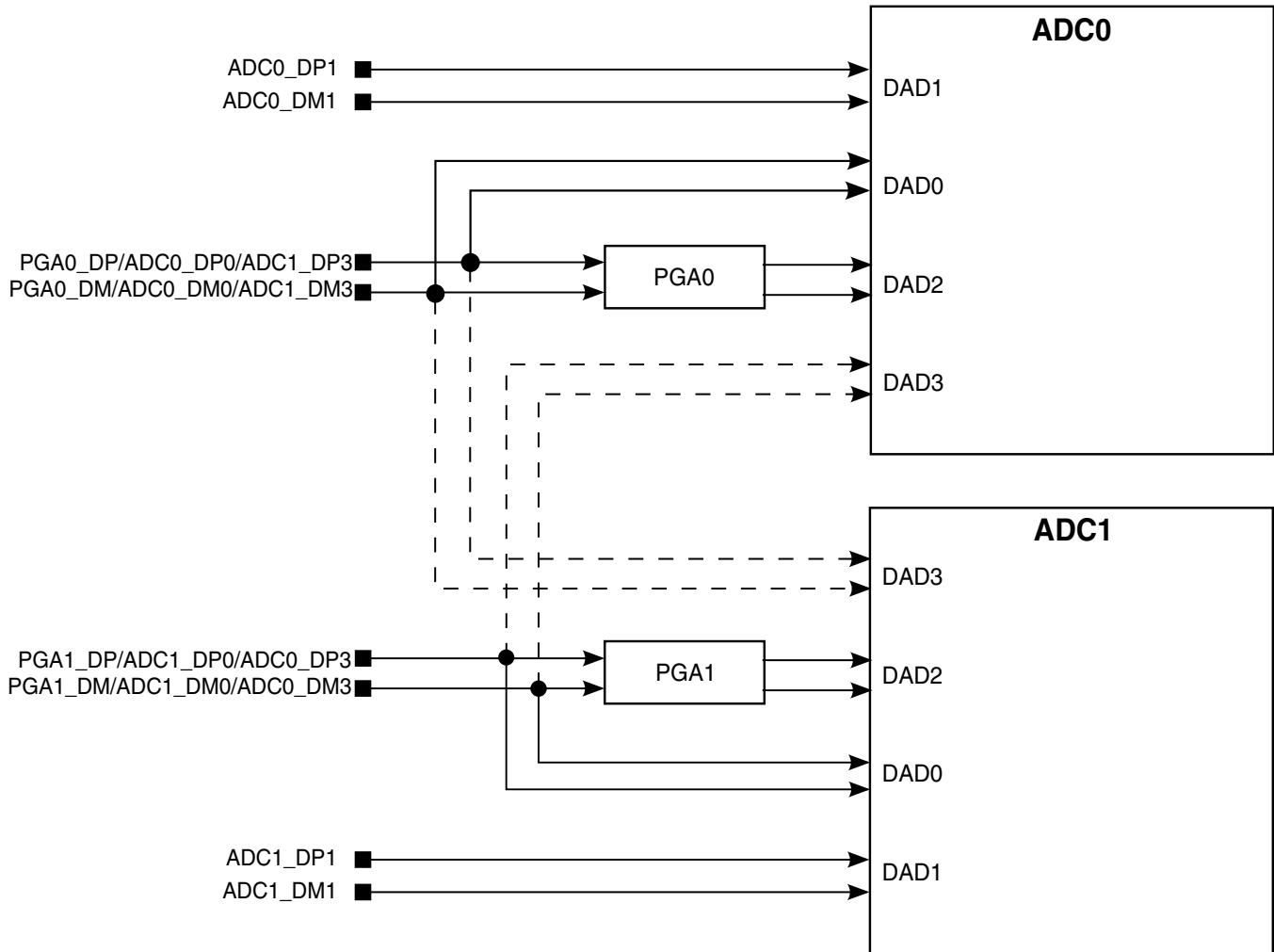
Figure 3-35. PGA Integration
