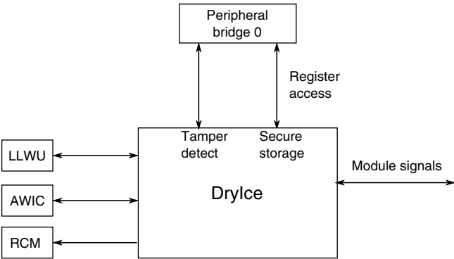
Figure 3-31. Drylce configuration
