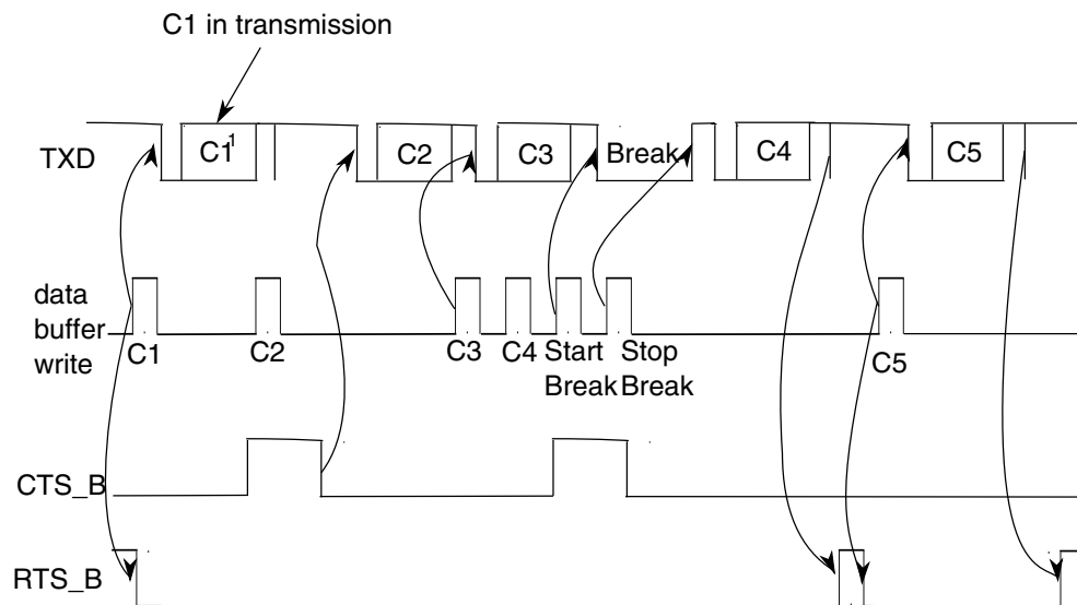
Figure 47-188. Transmitter RTS and CTS timing diagram
