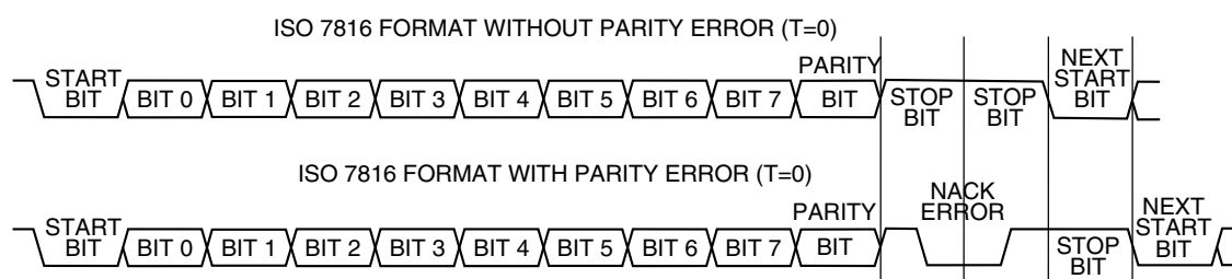
Figure 47-212. ISO-7816 T = 0 data format
