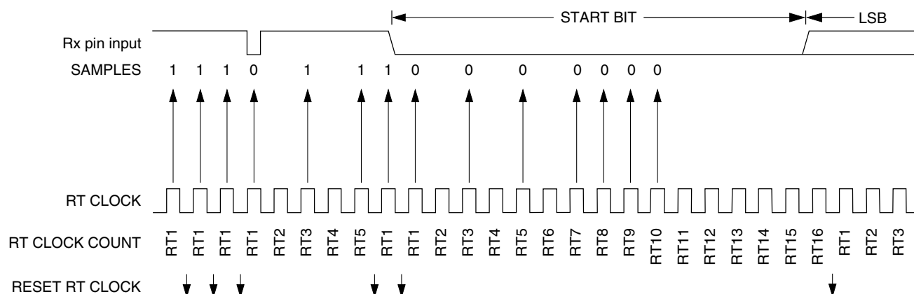
Figure 47-191. Start bit search example 1 ( C7816[ISO\_7816E] = 0 )
