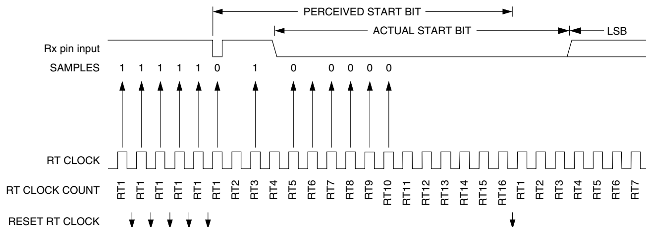
Figure 47-192. Start bit search example 2 ( C7816[ISO\_7816E] = 0 )
