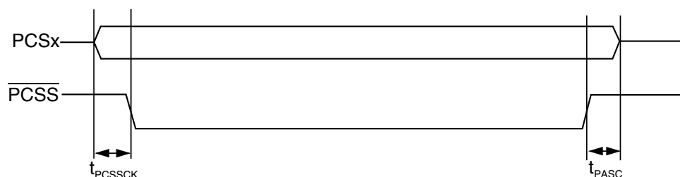
Figure 45-93. Peripheral Chip Select Strobe Timing
