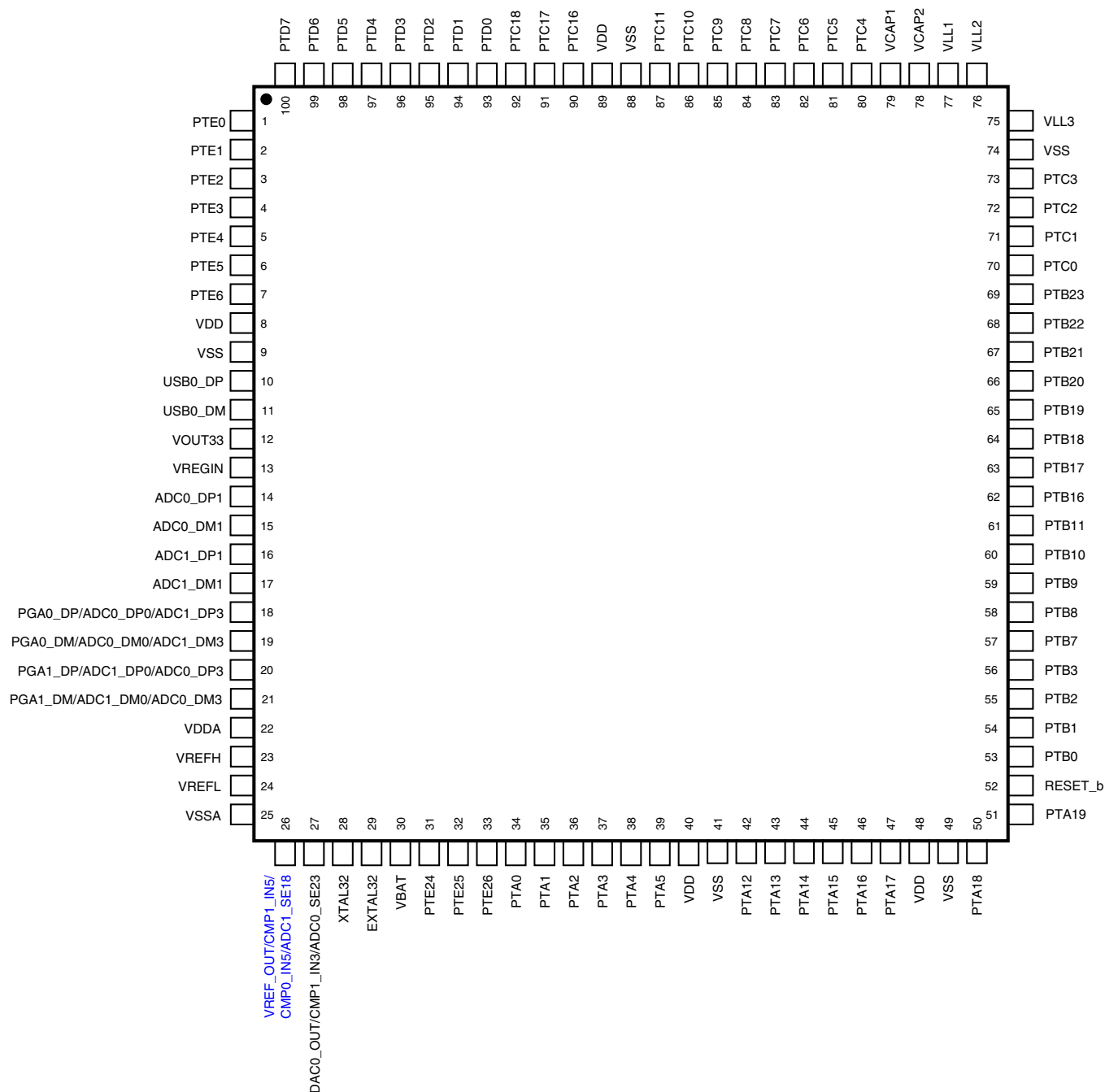
Figure 10-2. K40 100 LQFP Pinout Diagram
