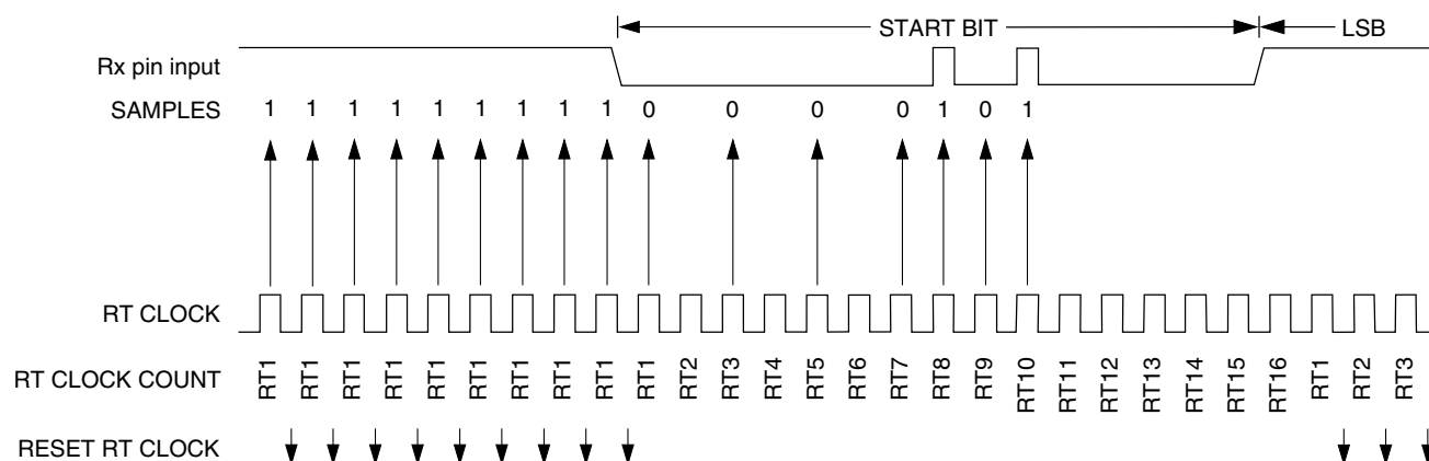
Figure 47-196. Start bit search example 6
