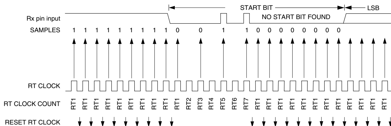
Figure 47-195. Start bit search example 5 (C7816[ISO_7816E] = 0)
