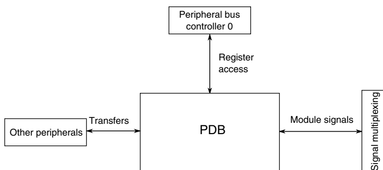
Figure 3-39. PDB configuration
