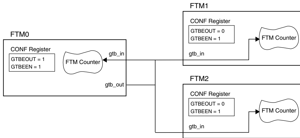
Figure 3-42. FTM Global Time Base Configuration
