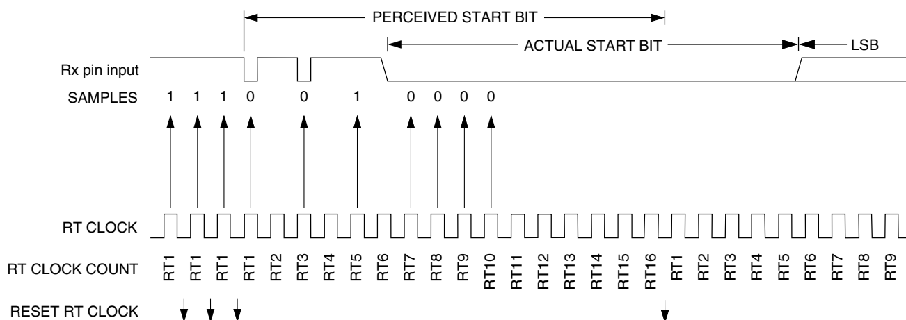
Figure 47-193. Start bit search example 3 (C7816[ISO_7816E] = 0)
