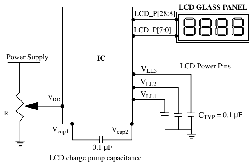
Figure 52-43. Power connections for contrast control
