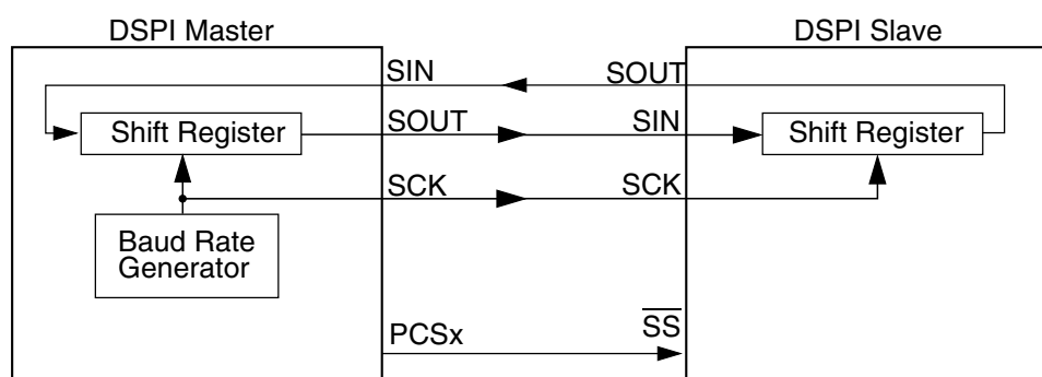
Figure 45-91. SPI Serial Protocol Overview
