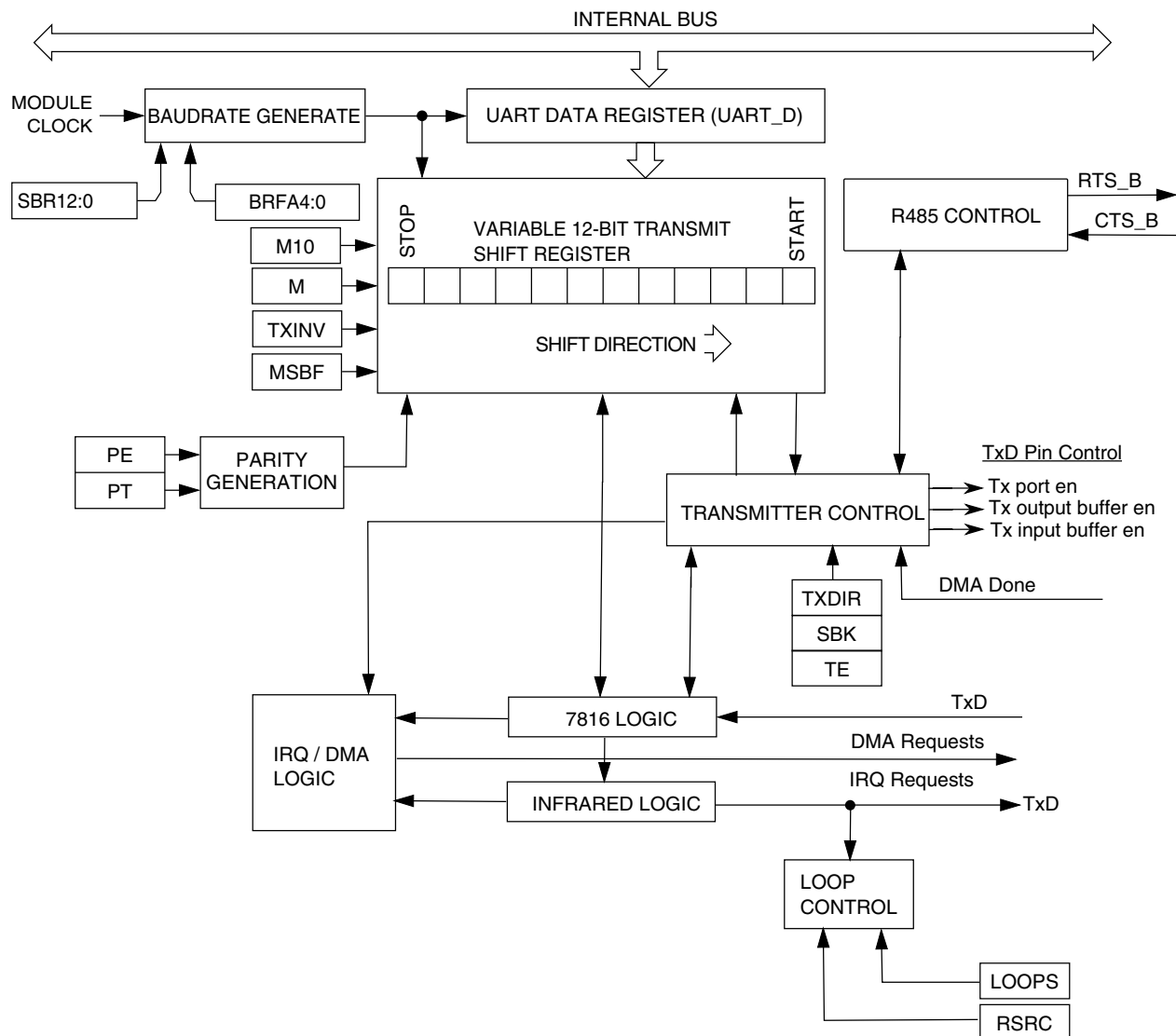
Figure 47-187. Transmitter Block Diagram
