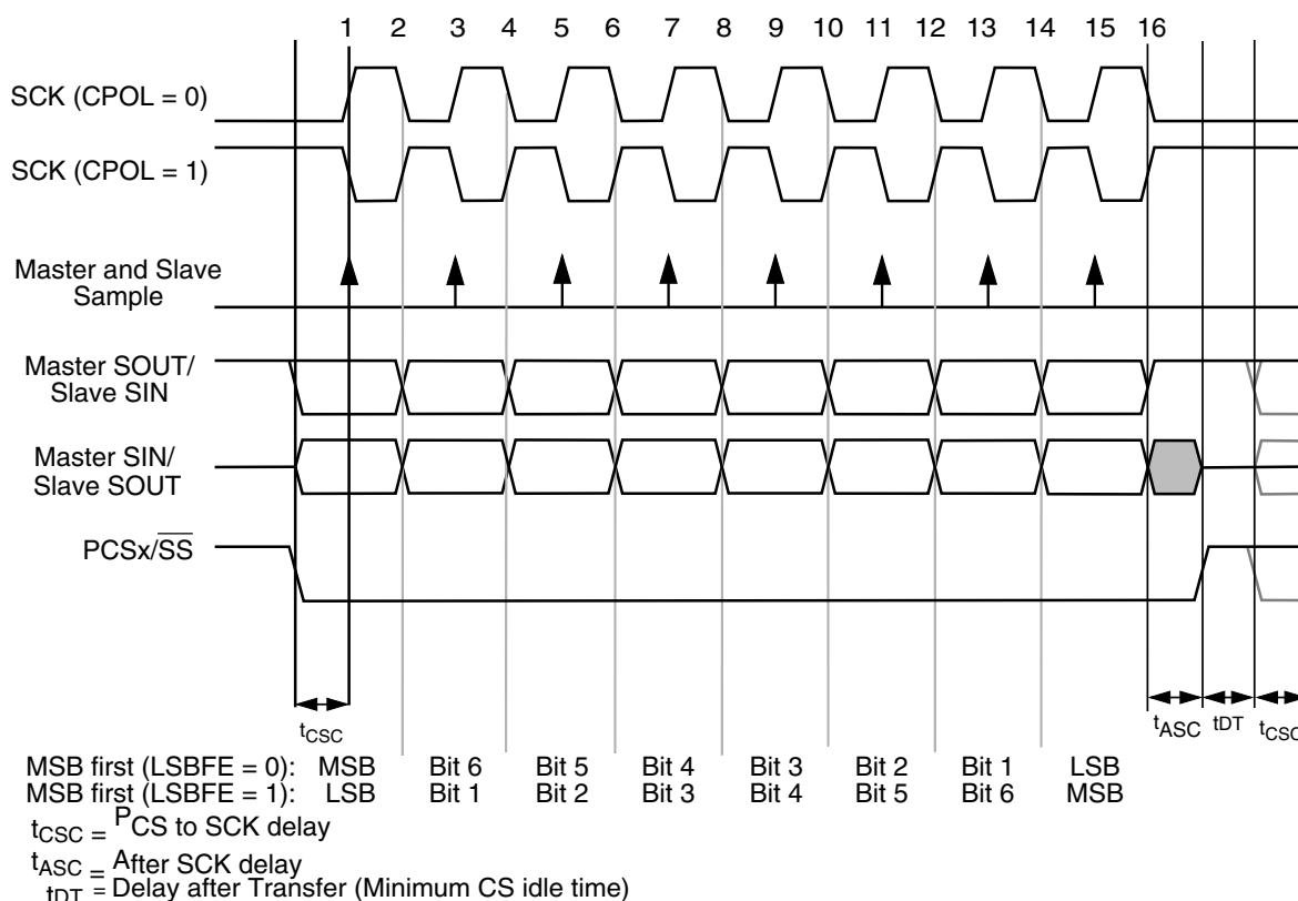
Figure 45-94. DSPI Transfer Timing Diagram (MTFE=0, CPHA=0, FMSZ=8)
