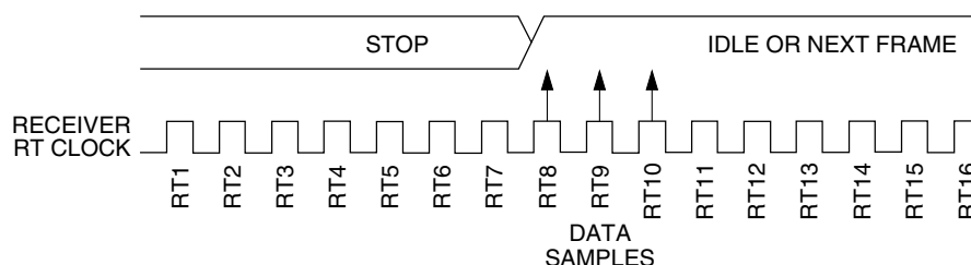
Figure 44-251. Fast data
