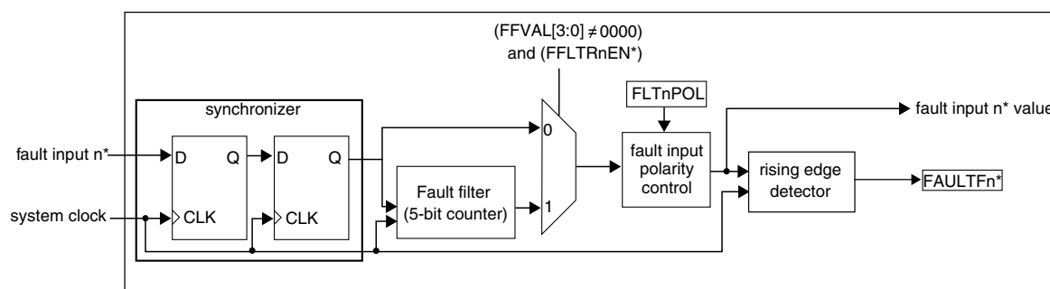
Figure 36-233. Fault Input n Control Block Diagram
