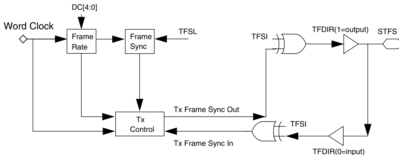
Figure 46-57. I²S transmit frame sync generator block diagram
