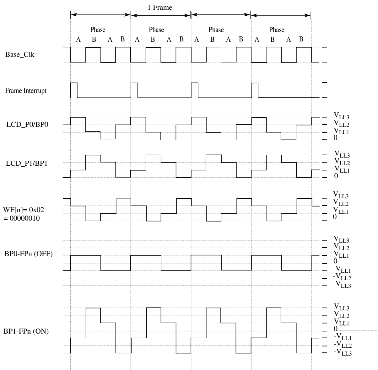
Figure 49-29. 1/2 Duty and 1/3 bias (low-power waveform)
