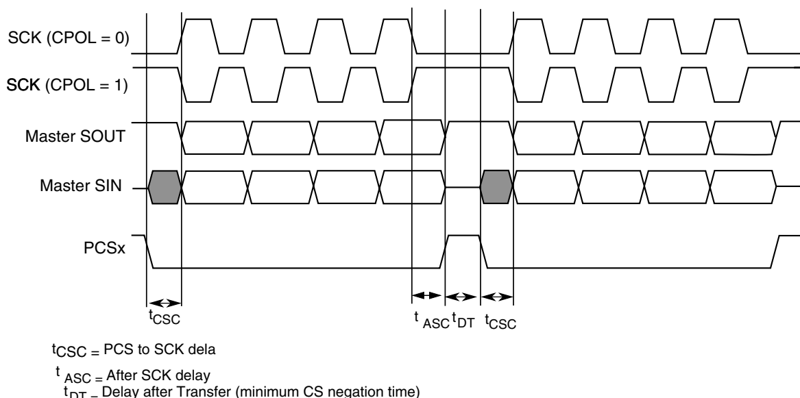
Figure 42-74. Example of Non-Continuous Format (CPHA=1, CONT=0)
