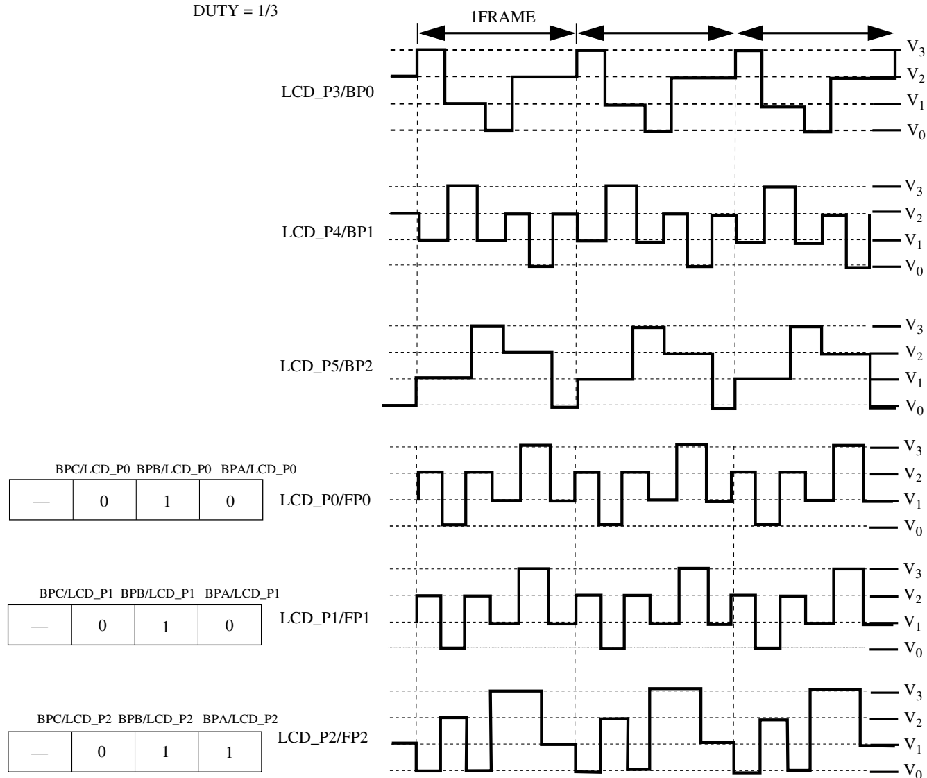
Figure 49-40. LCD waveforms
