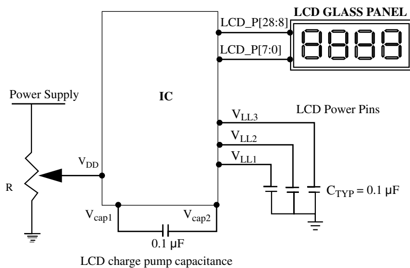
Figure 50-43. Power connections for contrast control
