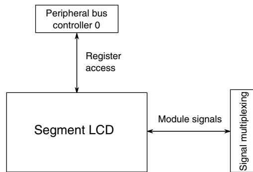
Figure 3-57. SLCD configuration
